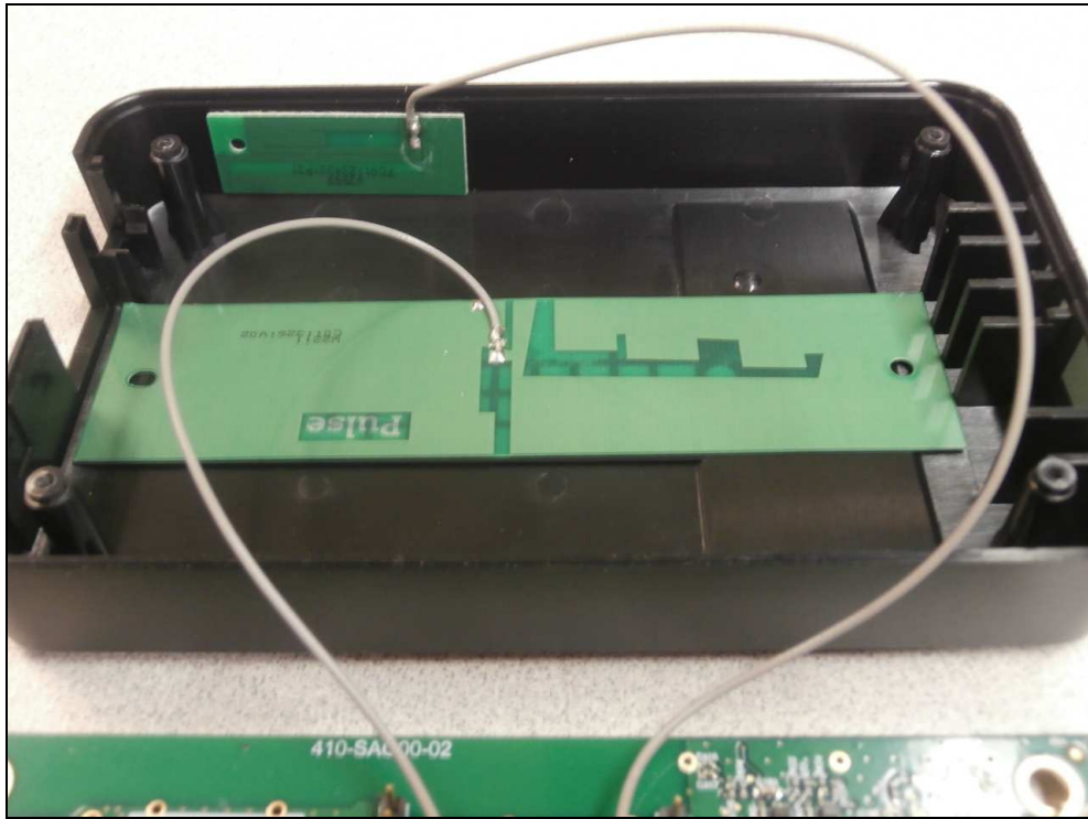
Figure 4: Internal Photo
