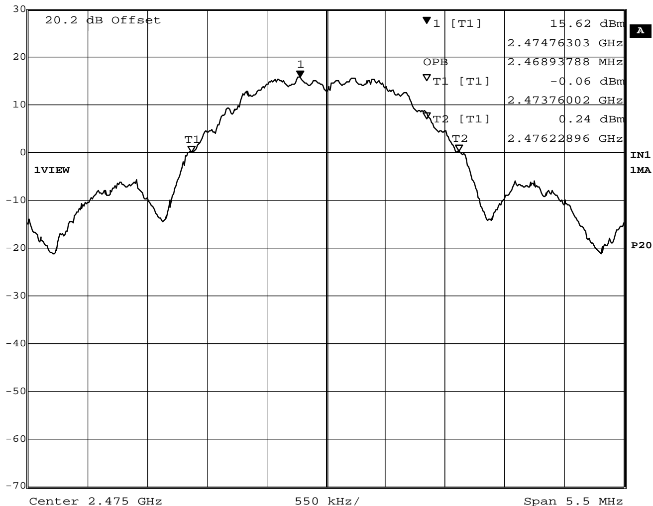
Figure 8 – 99% Power Bandwidth = 2.47 MHz
