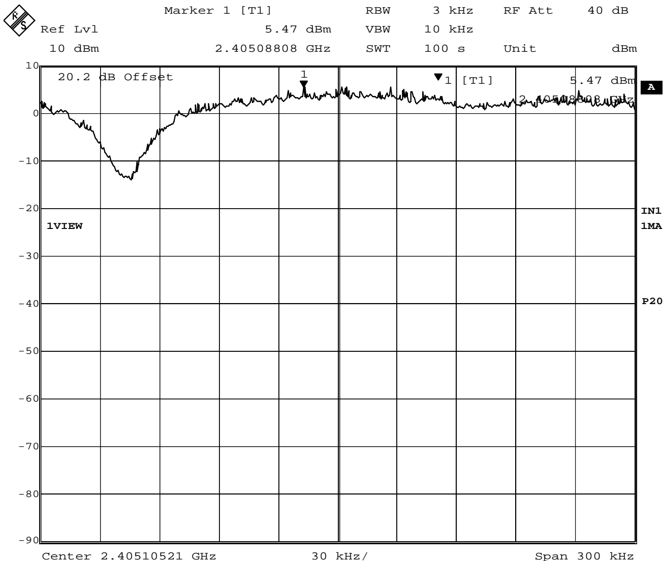
Figure 5: Power Spectral Density measurement
