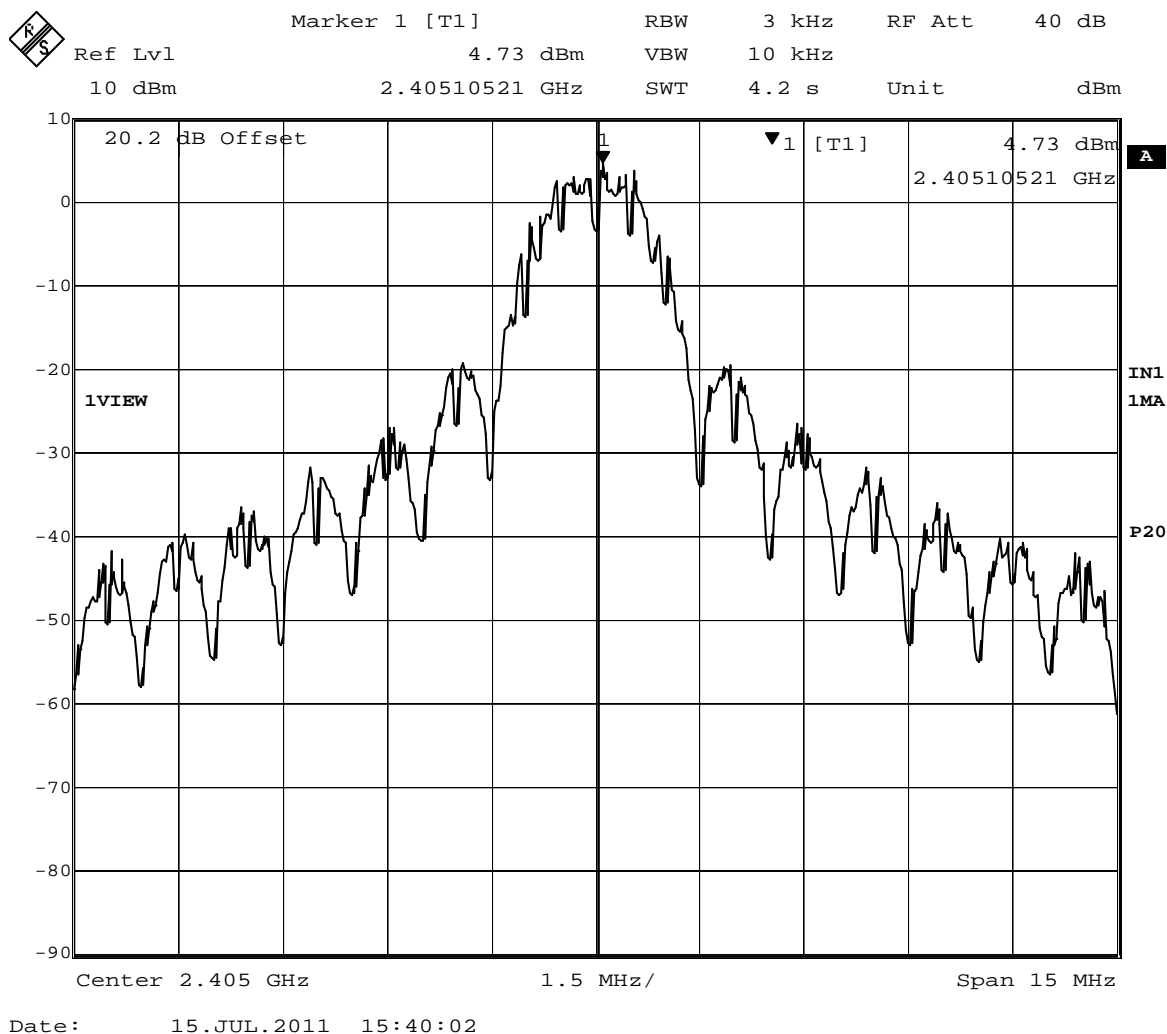
Figure 4: Peak Reference Frequency
