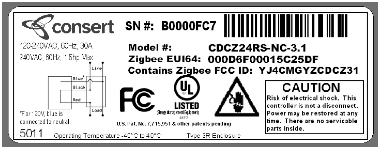
Figure 1: View of Label for a “Device Controller” using the Limited Modular Device.
