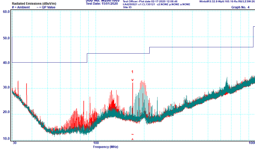
Graph 6-14: Transmitter Spurious Emissions, 30 – 1000 MHz, 80 MHz Bandwidth
