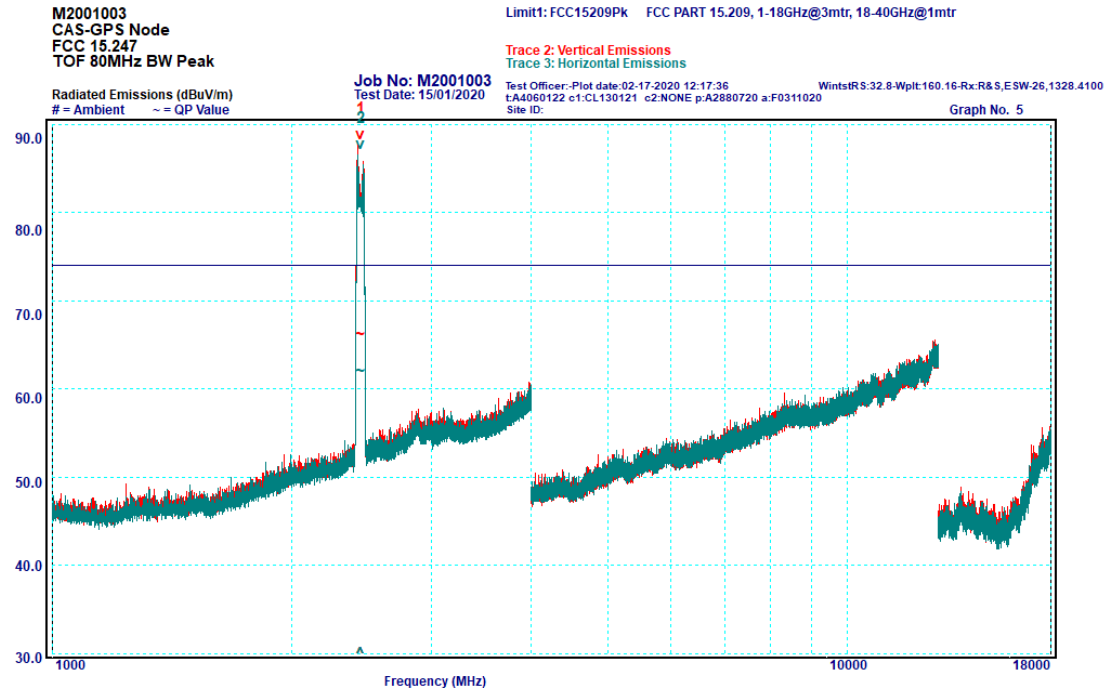
Graph 6-16: Transmitter Spurious Emissions, 1 – 18 GHz, 80 MHz Bandwidth, Peak
