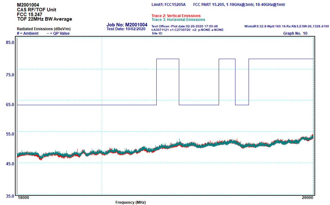
Graph 6-21: Transmitter Spurious Emissions, 18 – 26 GHz, 22 MHz Bandwidth, Average
