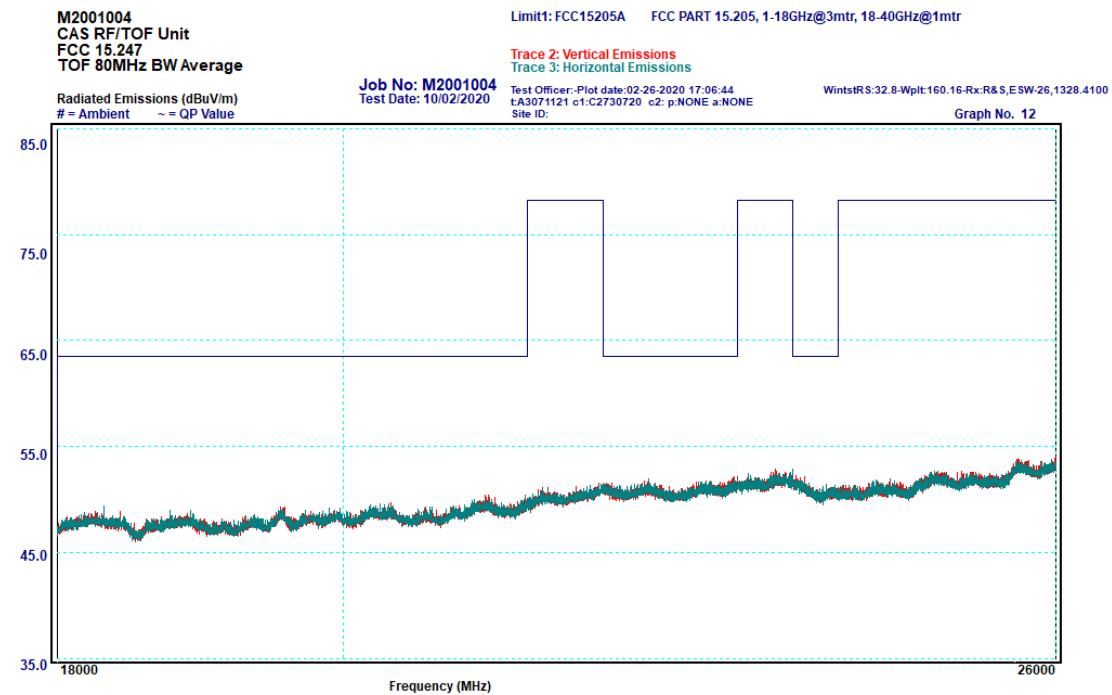
Graph 6-22: Transmitter Spurious Emissions, 18 – 26 GHz, 80 MHz Bandwidth, Average
