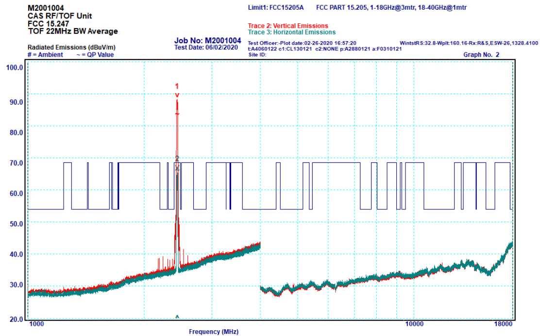
Graph 6-17: Transmitter Spurious Emissions, 1 – 18 GHz, 22 MHz Bandwidth, Average
