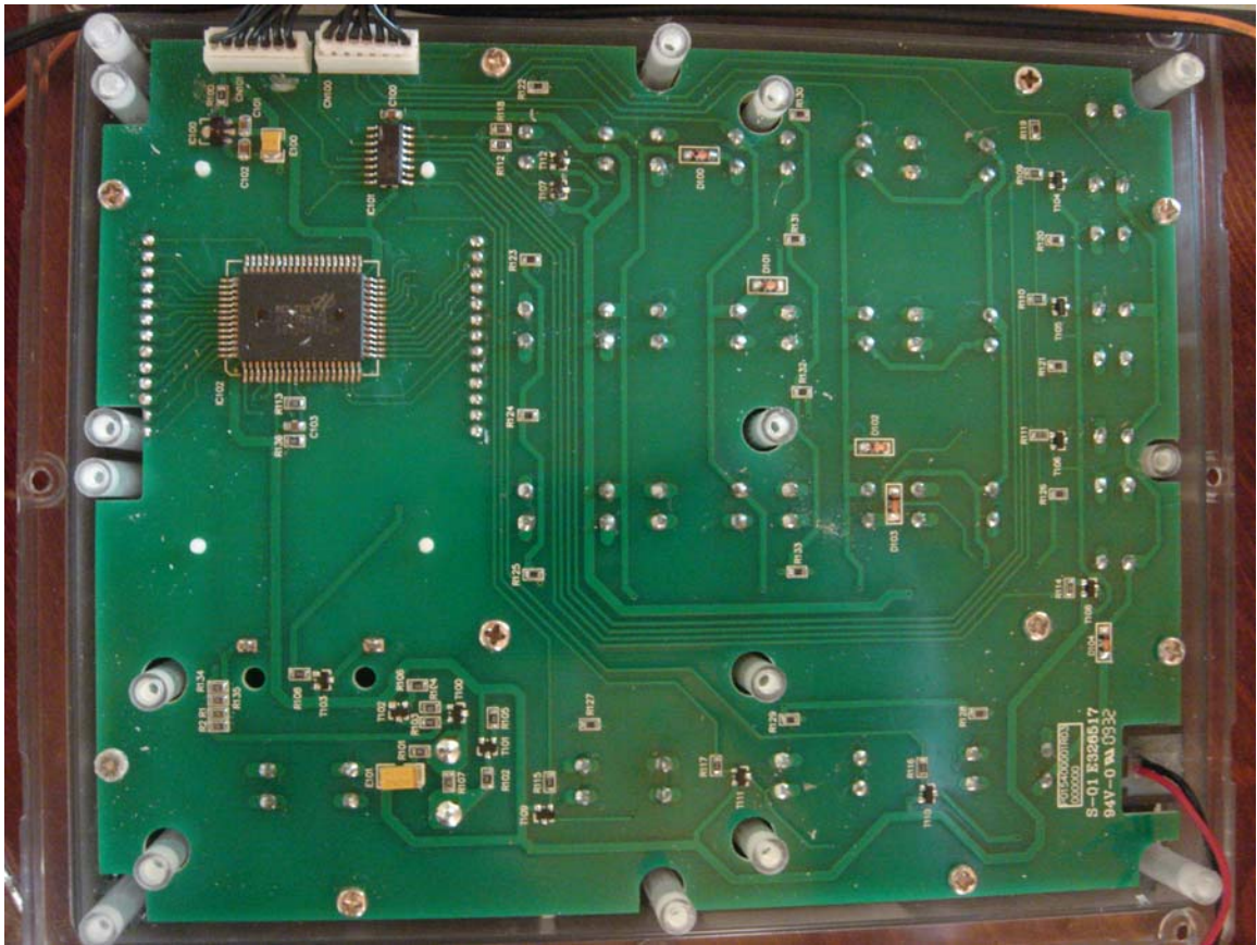
Board 3 Side 1
