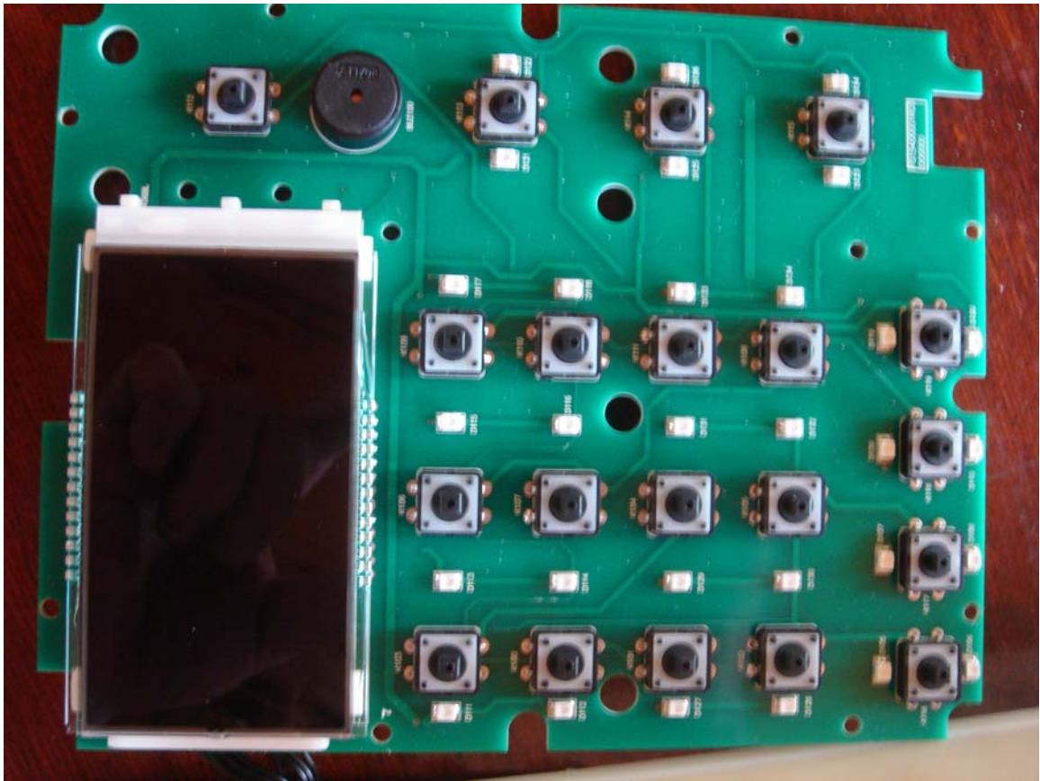
Board 3 Side 2
