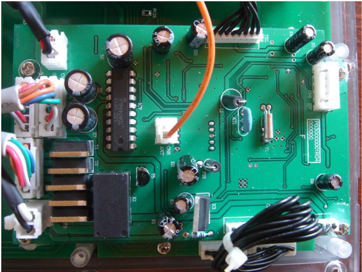
Board 2 Side 1
