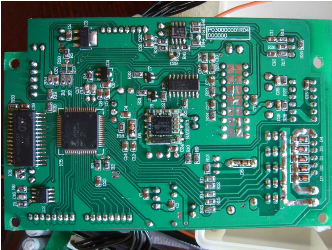
Board 2 Side 2
