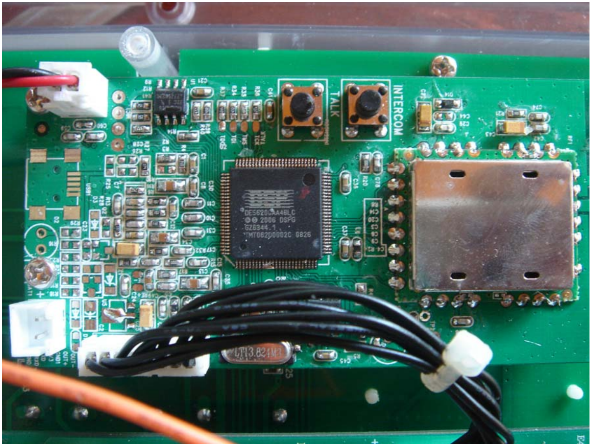
Board 1 Side 1
