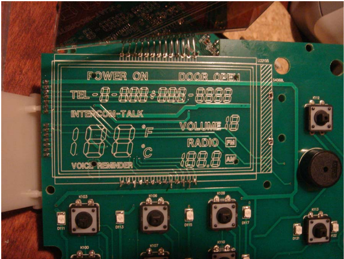
Board 3 under LCD
