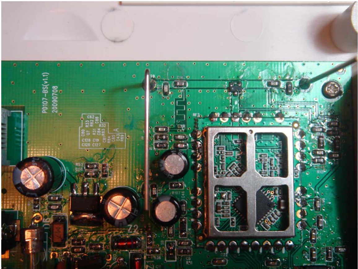
Phone Base Board 1 Can Removed
