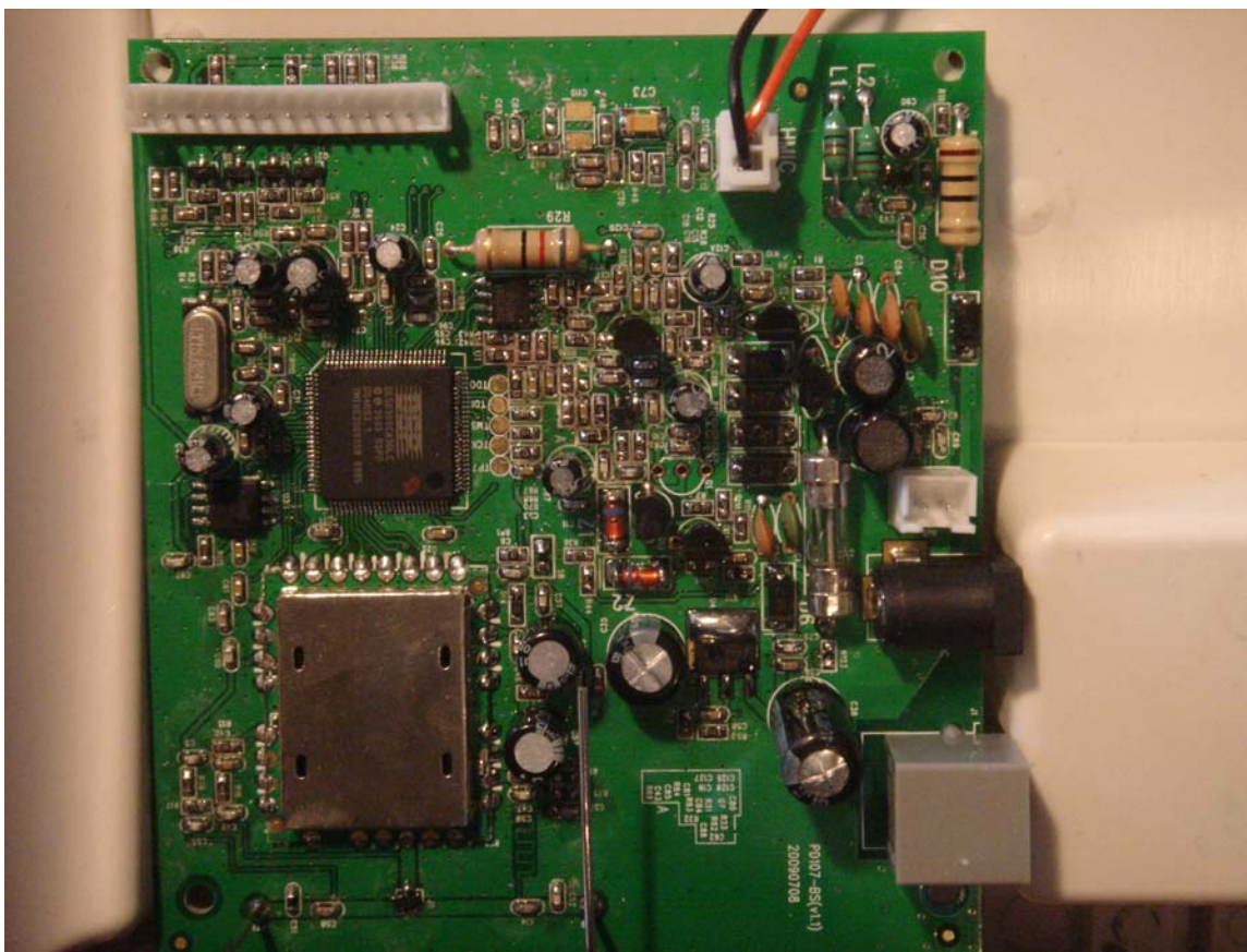
Base PC Board Side 1
