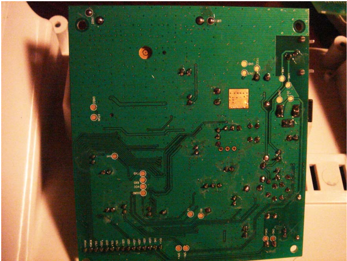
Base PC Board Side 2
