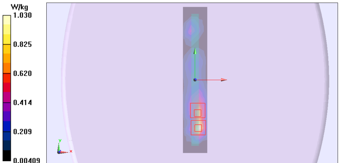
Figure 12 802.11b Test Position 3 Channel 1
