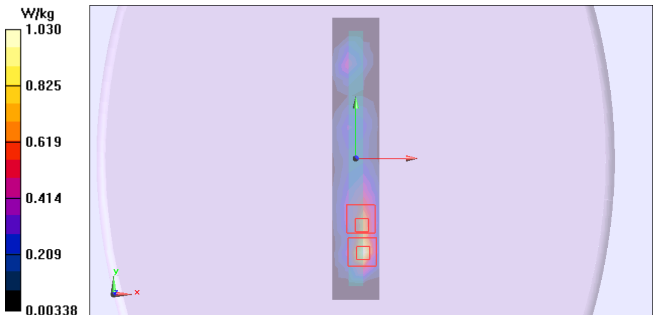
Figure 11 802.11b Test Position 3 Channel 6
