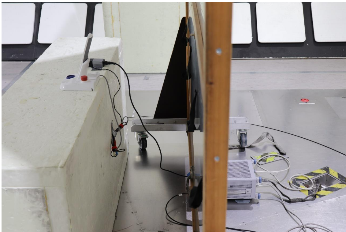
Photograph 1. AC Power-Line Conducted Emissions
