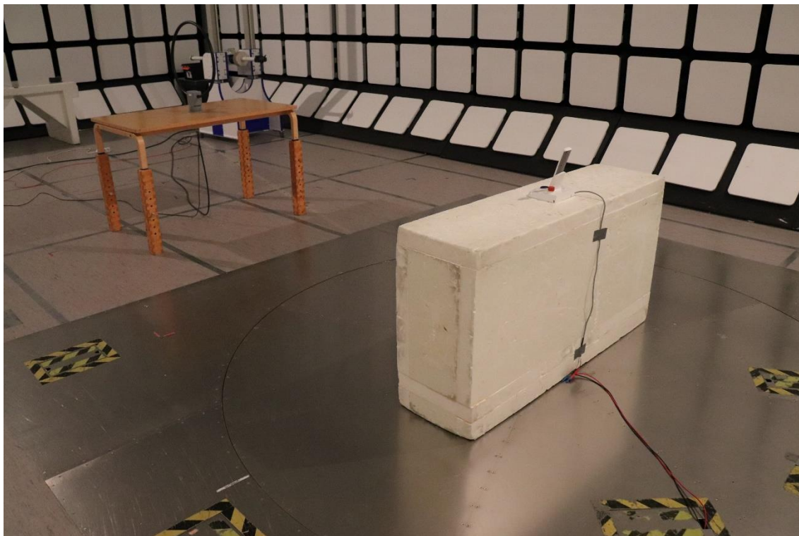
Photograph 2. Radiated Emissions 9 kHz – 30 MHz
