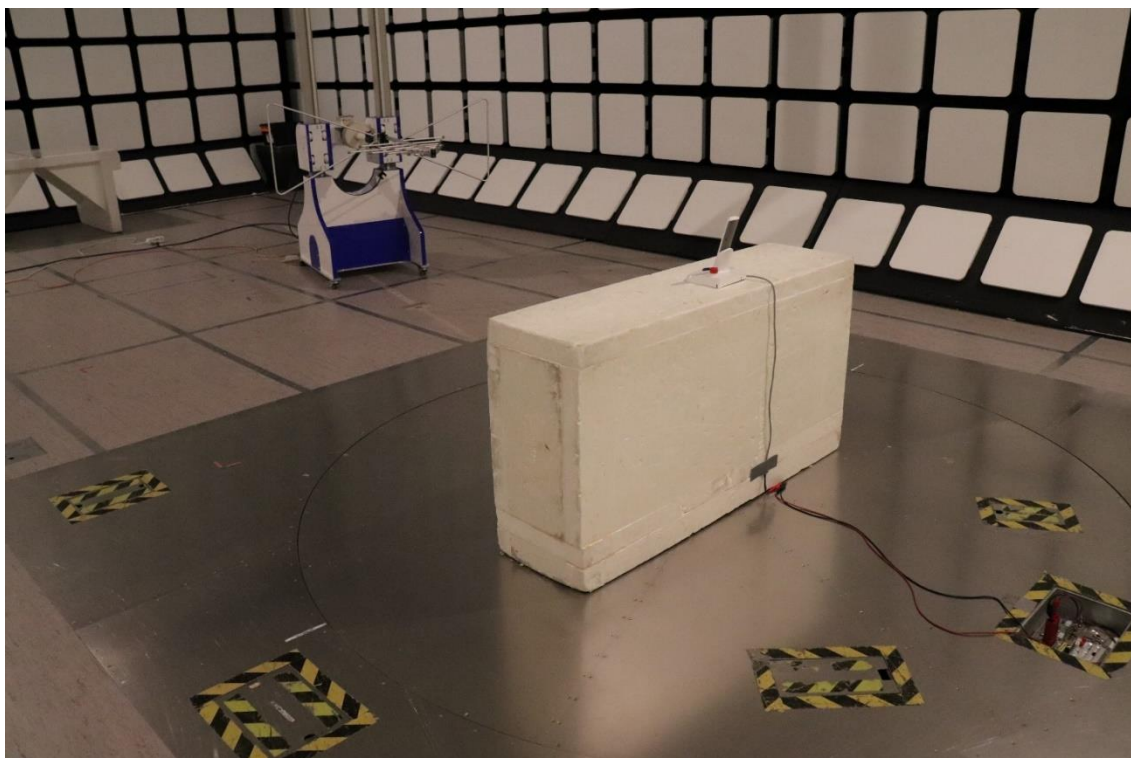
Photograph 3. Radiated Emissions 30 – 1000 MHz
