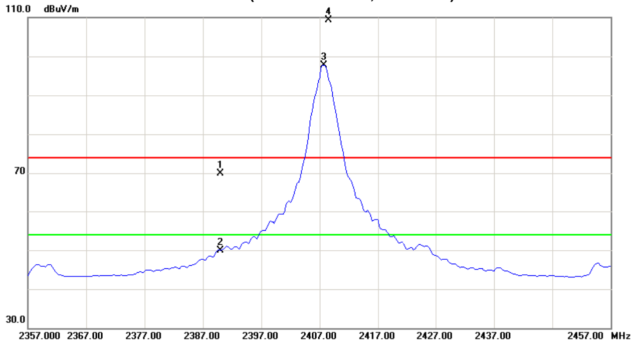
TX CH01(Above 1000 MHz, Horizontal)
