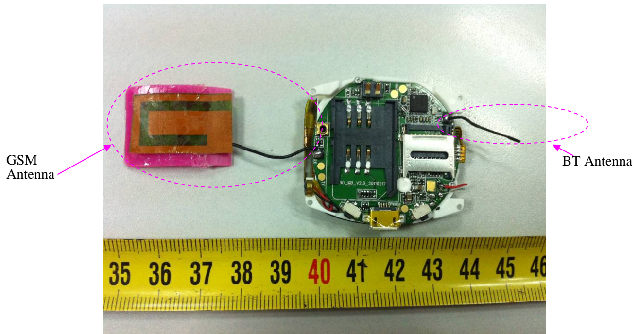
EUT – Main Board with LCD Bottom View
