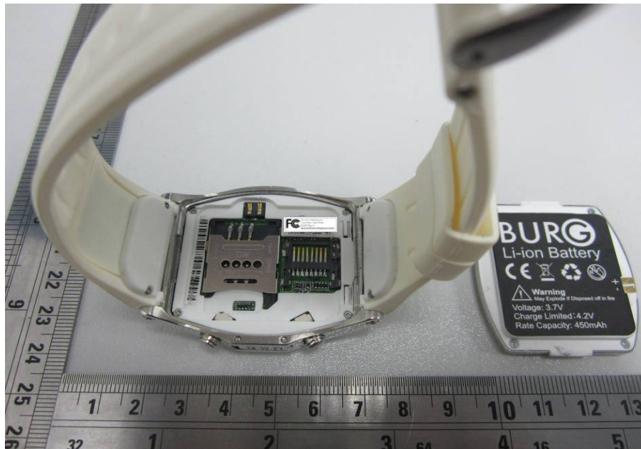
EUT – Battery off View
