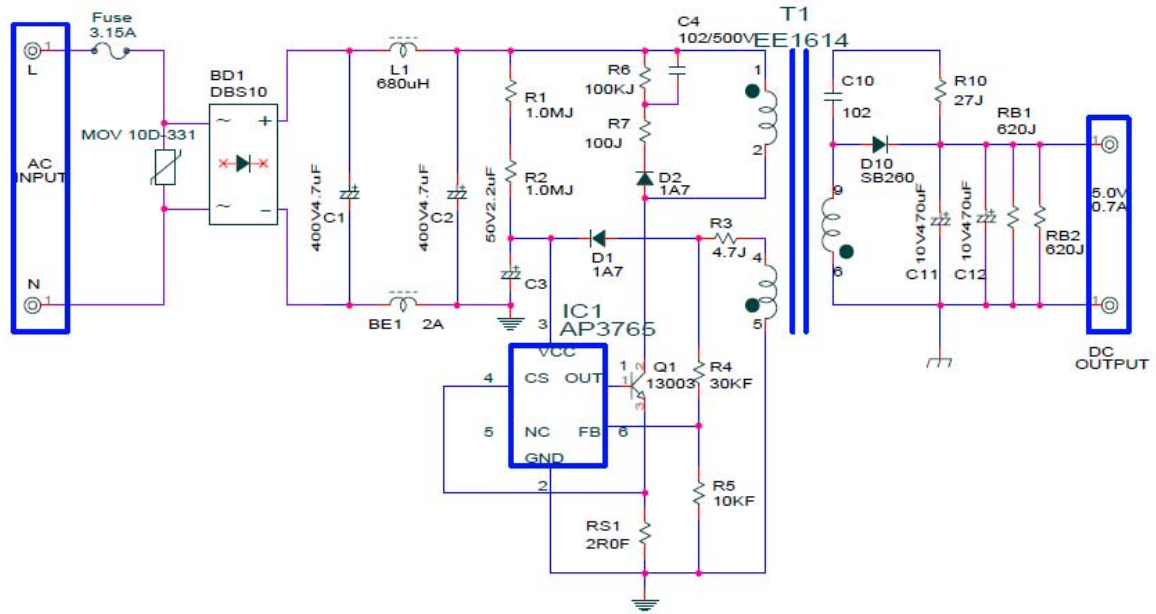
Before Schematic
