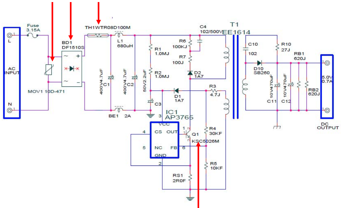
After Schematic
