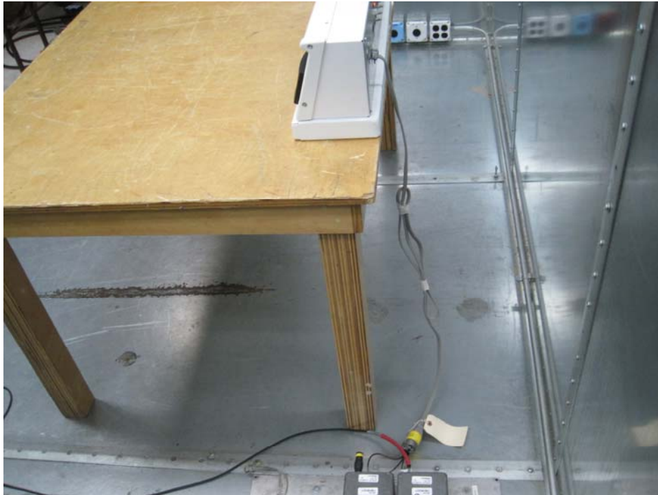
Conducted Emissions, Power Leads, Cable Setup
