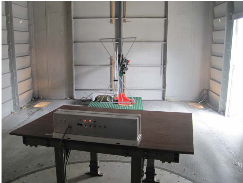
Radiated Emissions, Harmonics, Vertical Antenna Polarization, 80 MHz to 1 GHz
