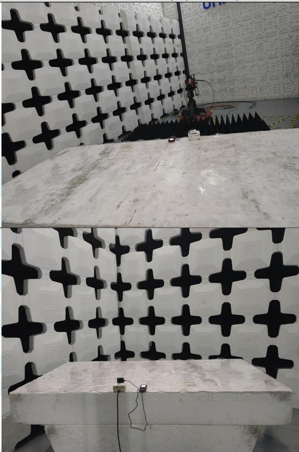
Radiated emission Test Setup-2 (Above 1 GHz)
