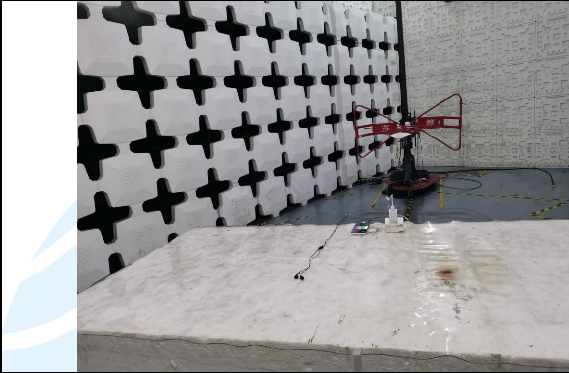
Radiated emission Test Setup-1 (30 MHz~1 GHz) – Test Mode 1
