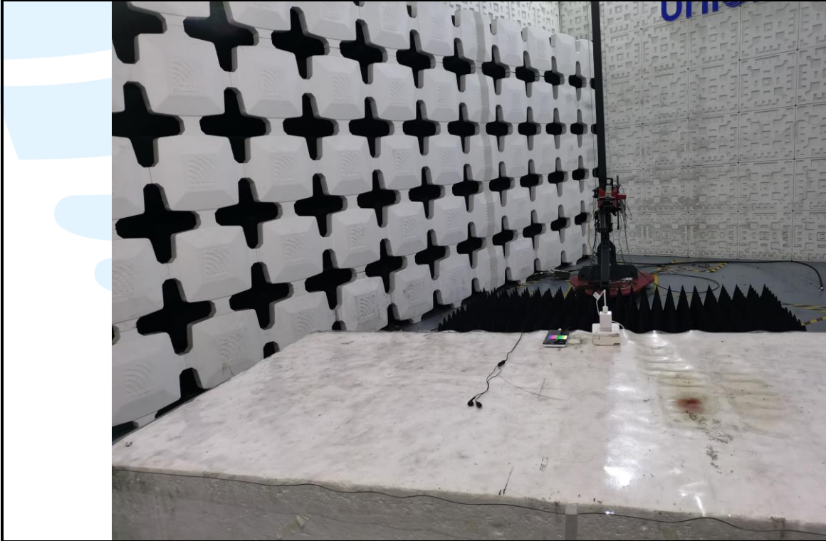
Radiated emission Test Setup-2 (Above 1 GHz) - Test Mode 1
