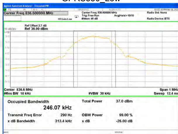
GPRS850_Middle
