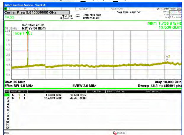
HSDPA_Band 4_High
