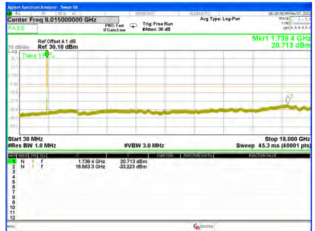
WCDMA_Band 4_Middle
