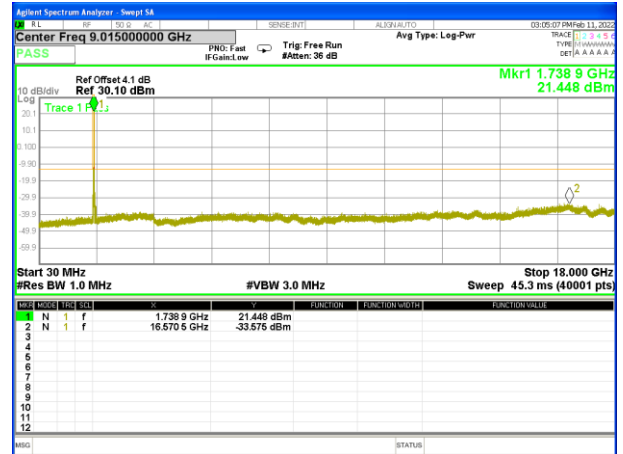
HSUPA_Band 4_Middle
