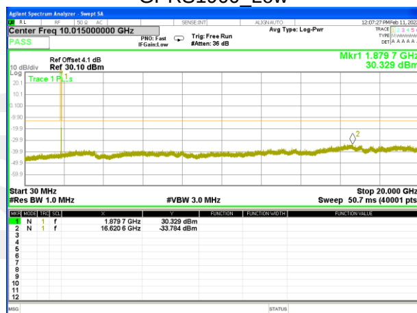
GPRS1900_Middle
