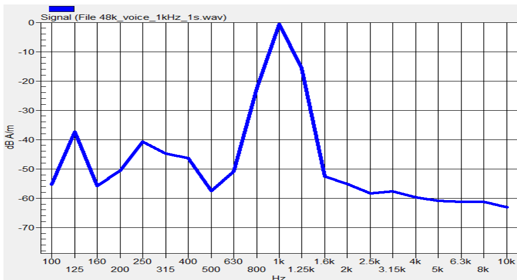
Fig. 5.12 Audio signal spectrum of the narrowband signal (48kHz_voice_1kHz)
