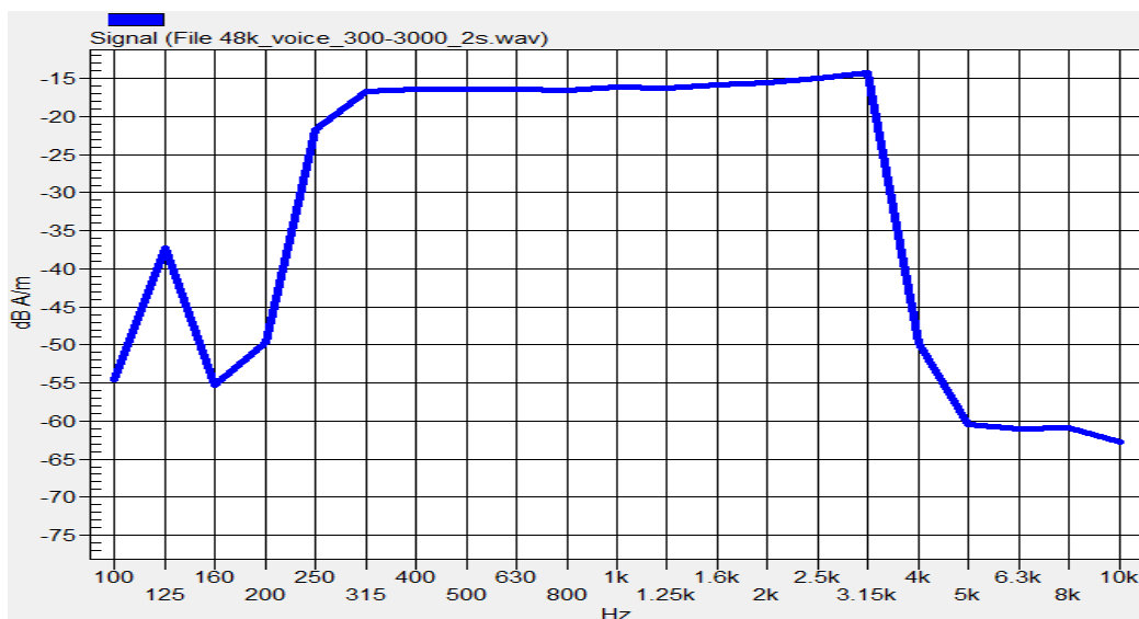
Fig. 5.11 Audio signal spectrum of the broadband signal (48kHz_voice_300Hz~3 kHz)
