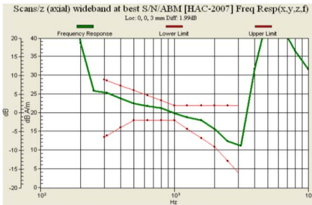
Fig. 9.5 GSM1900 Ch661
