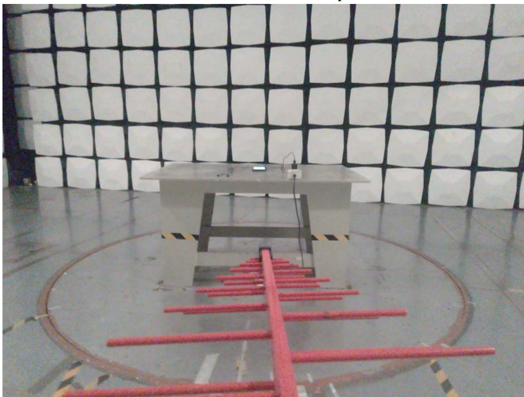
Radiated Emission Below 1GHz Adapter 2# View
