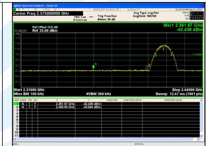
Out Of Band Emission IEEE 802.11b_Channel 1_20MHz_Antenna 0
