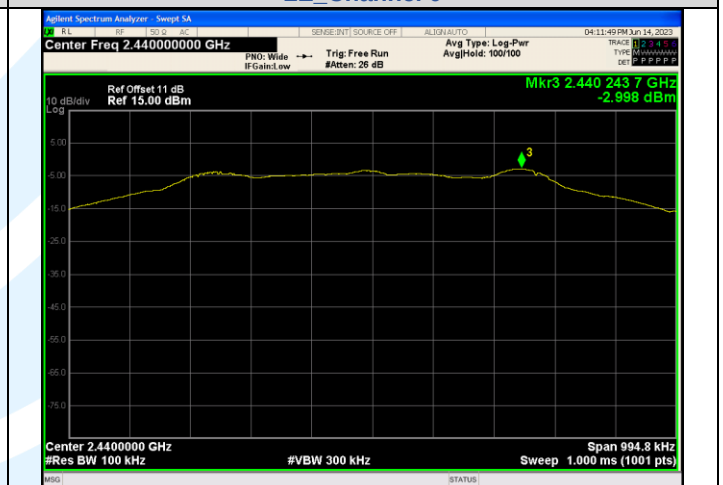
In-Band Reference Level LE_Channel 19
