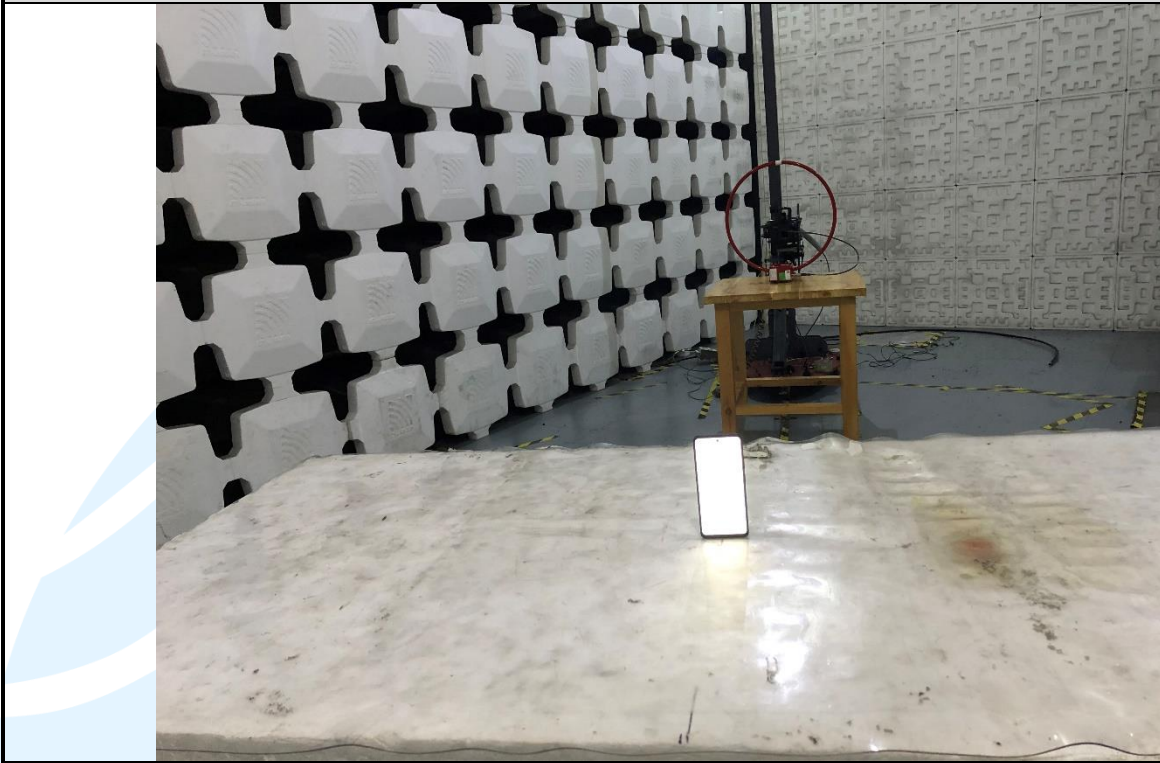
Radiated emission Test Setup (Below 30 MHz)
