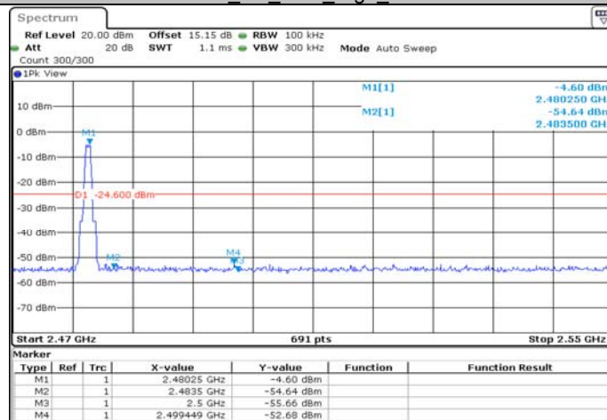
BLE_1M_Ant1_High_2480
