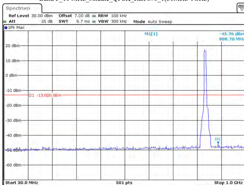
Band 5_10 MHz_Middle_QPSK_RB50#0_1(30MHz-1GHz)
