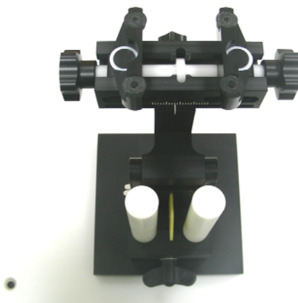
Fig. 5.8 Phone Positioner
