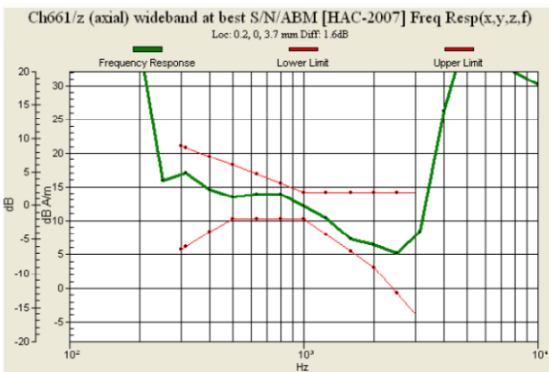
Fig. 9.5 GSM1900 Ch661
