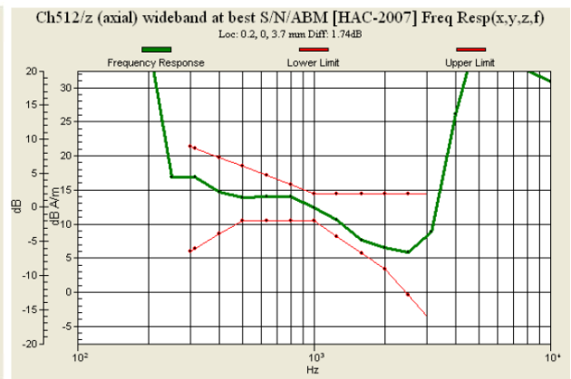
Fig. 9.4 GSM1900 Ch512
