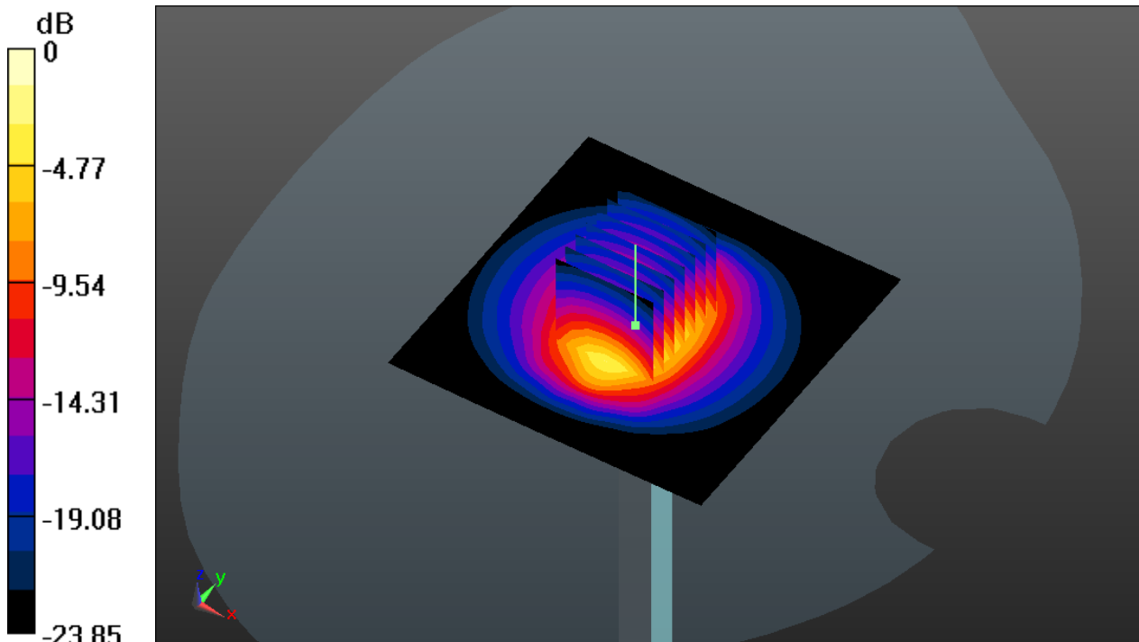
0 dB = 21.0 W/kg
