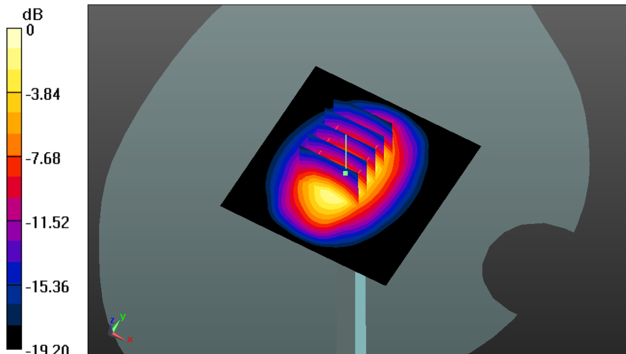
0 dB = 12.8 W/kg
