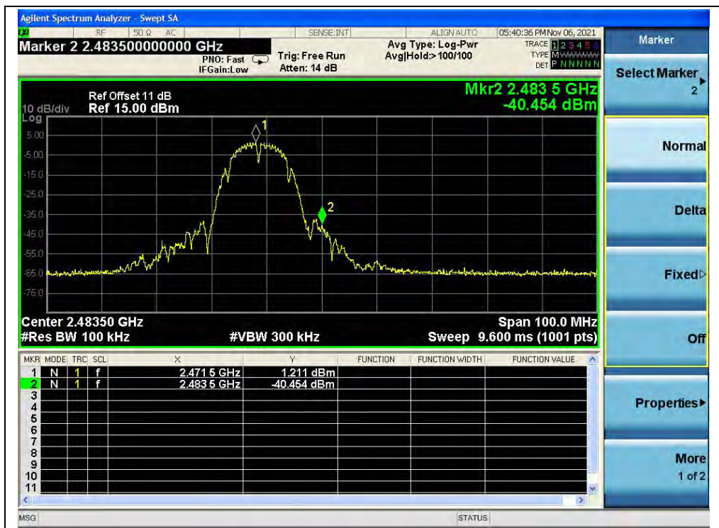
(Band Edge, Channel 13, 802.11b)
