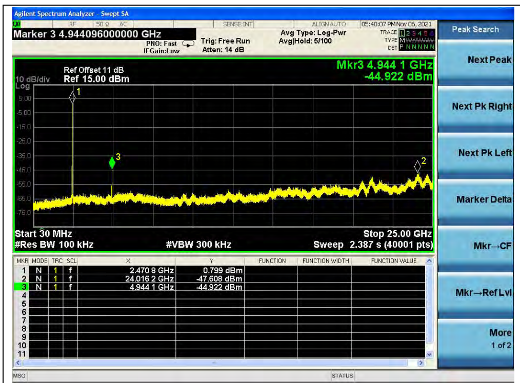
(30MHz to 25GHz, Channel 13, 802.11b)
