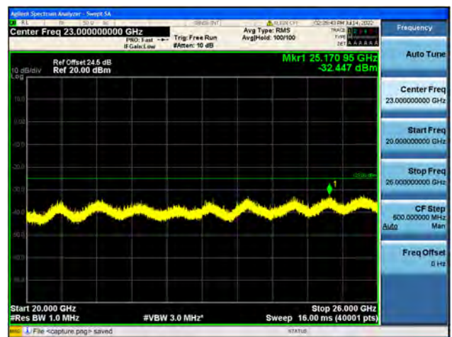
Band7-20G-26G / 15MHz / Mid CH / 64QAM
