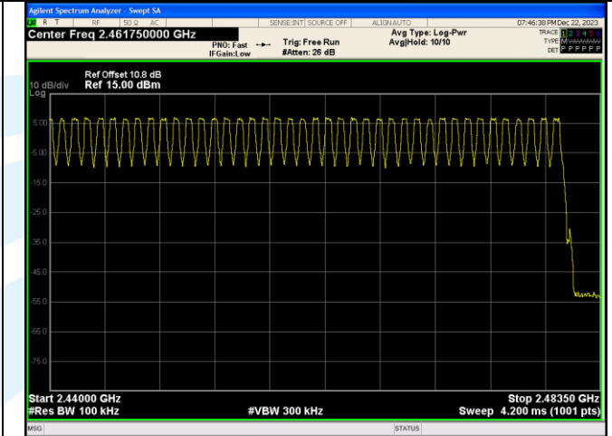
High End Spectrum Channel Hopping Plot GFSK
