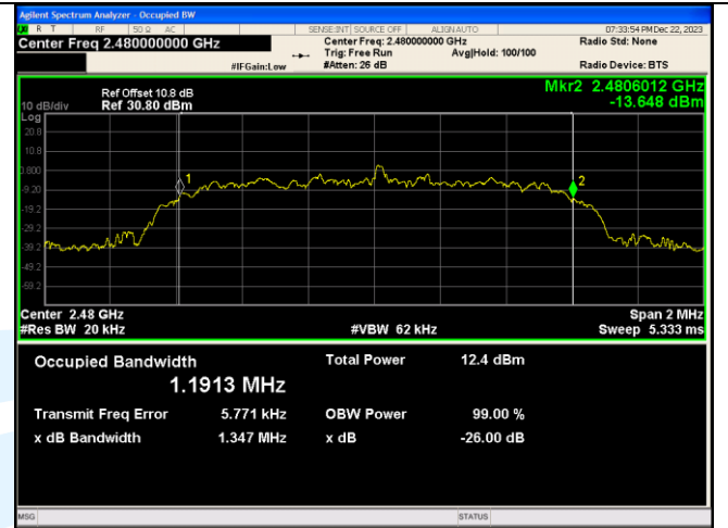
π/4DQPSK_2-DH5_Channel 78
