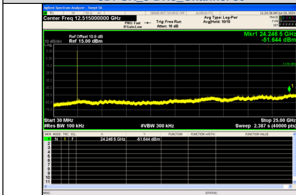
30.0 MHz - 25000.0 MHz
