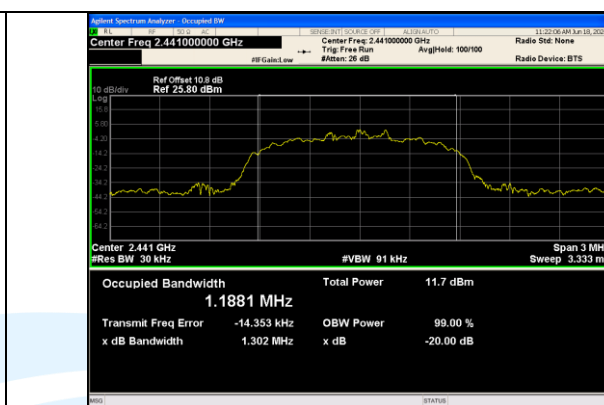
8DPSK_3-DH5_Channel 39
