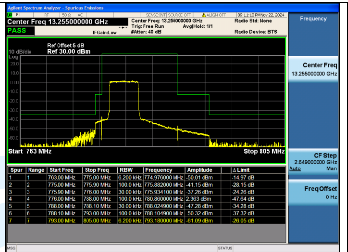
Band13 5MHz 64QAM 23205 25RB#0
