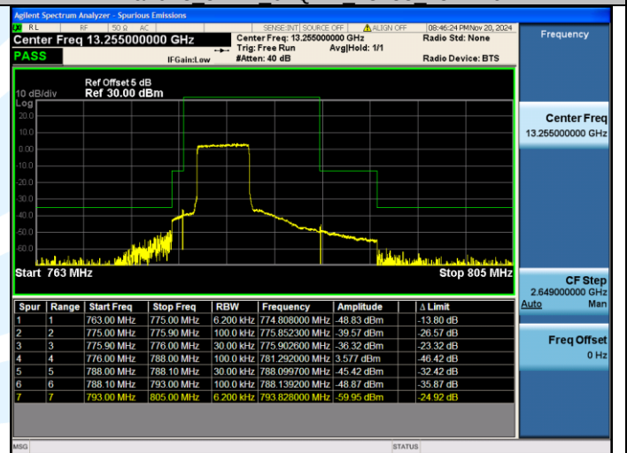
Band13 5MHz 16QAM 23205 25RB#0
