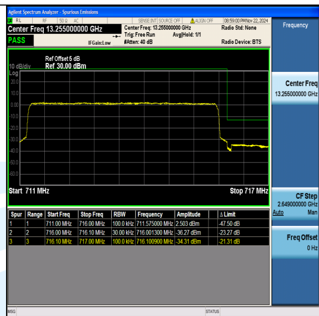
Band12 5MHz 64QAM 23155 25RB#0
