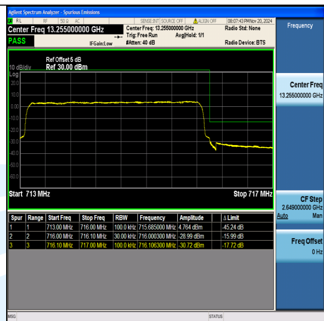
Band12 3MHz QPSK 23165 15RB#0
