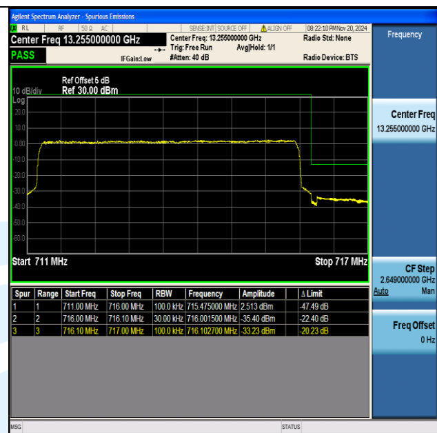
Band12 5MHz QPSK 23155 25RB#0
