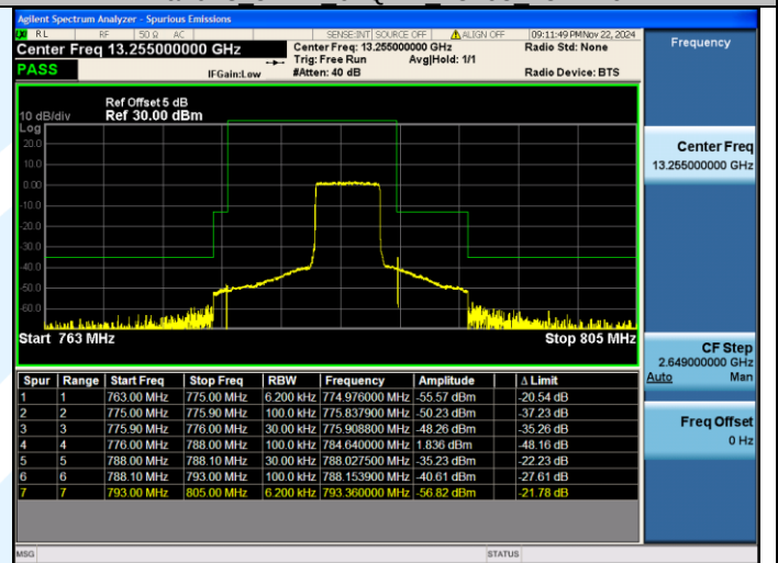
Band13 5MHz 64QAM 23255 25RB#0
