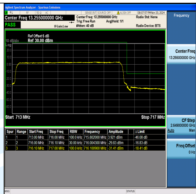
Band12 3MHz 16QAM 23165 15RB#0
