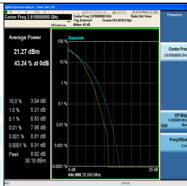
Band38-20MHz-64QAM-38150-100RB#0-PASS
