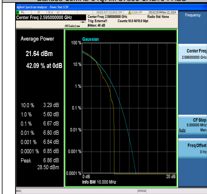
Band38-10MHz-64QAM-38000-1RB#0-PASS
