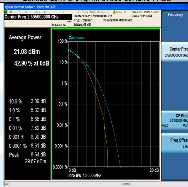
Band38-10MHz-64QAM-38000-50RB#0-PASS
