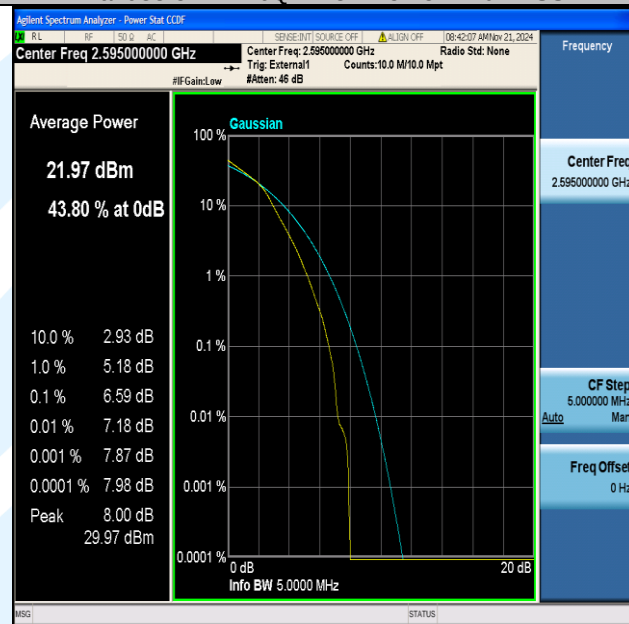
Band38-5MHz-16QAM-38000-25RB#0-PASS
