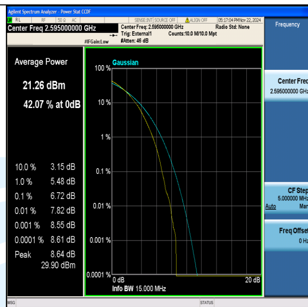
Band38-15MHz-64QAM-38000-75RB#0-PASS
