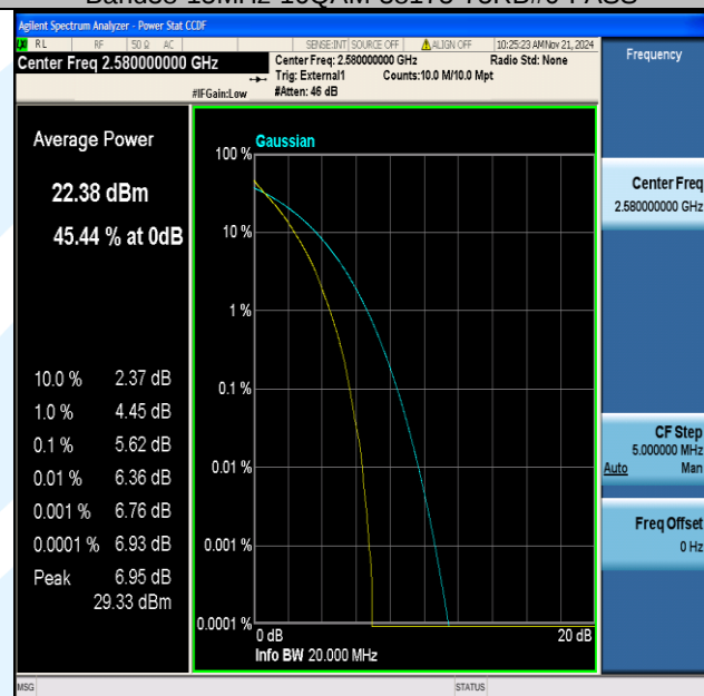
Band38-20MHz-QPSK-37850-100RB#0-PASS
