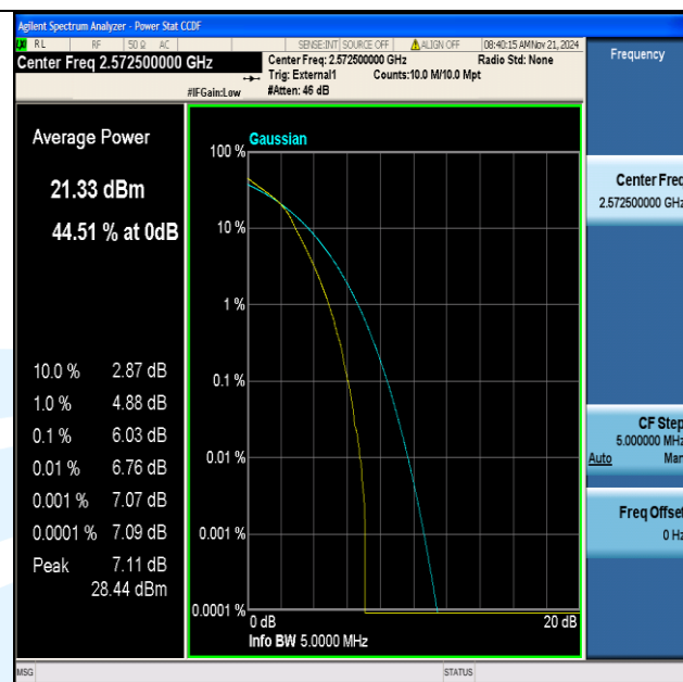
Band38-5MHz-16QAM-37775-25RB#0-PASS
