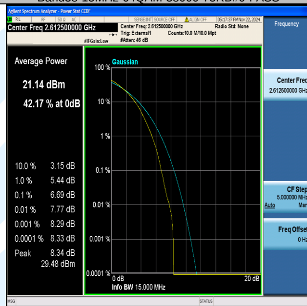
Band38-15MHz-64QAM-38175-75RB#0-PASS
