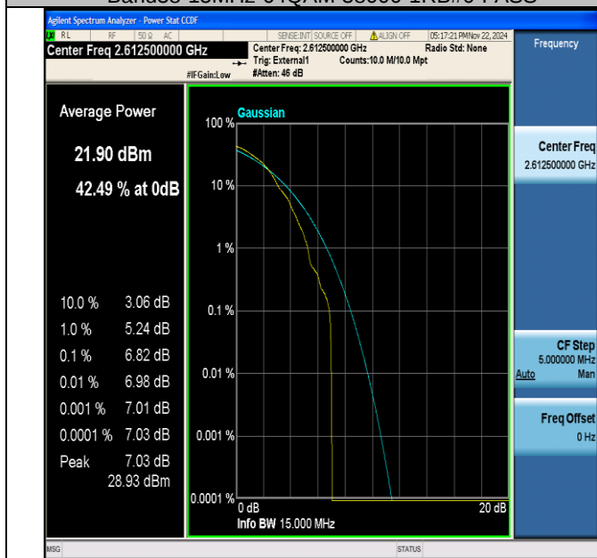
Band38-15MHz-64QAM-38175-1RB#0-PASS
