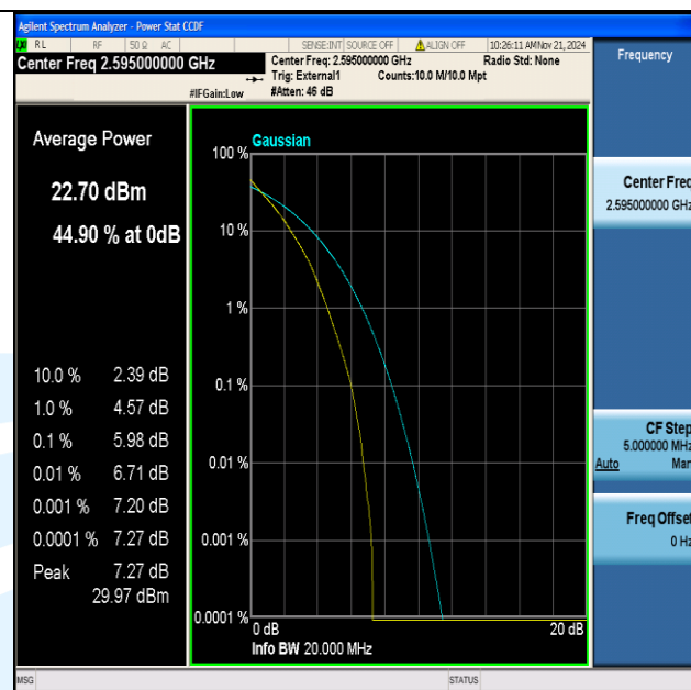
Band38-20MHz-QPSK-38000-100RB#0-PASS
