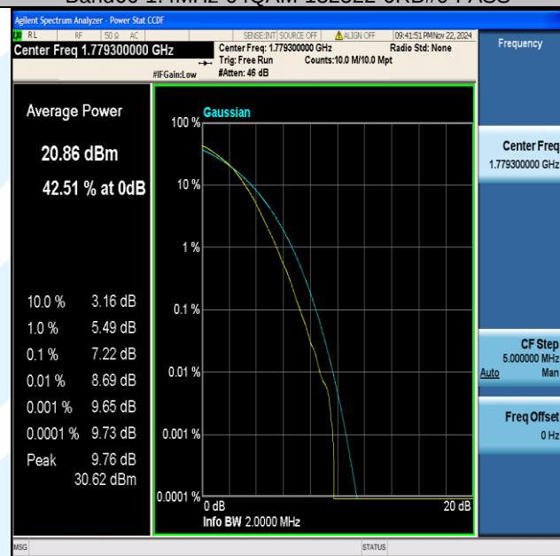
Band66-1.4MHz-64QAM-132665-6RB#0-PASS
