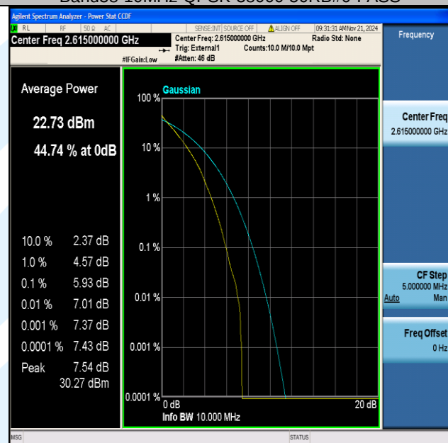
Band38-10MHz-QPSK-38200-50RB#0-PASS
