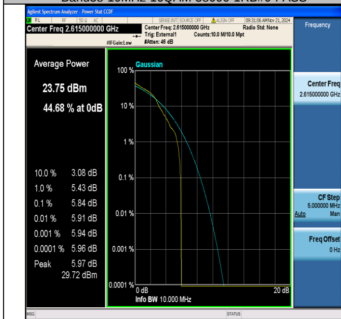
Band38-10MHz-16QAM-38200-1RB#0-PASS
