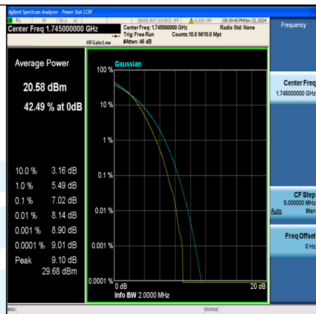
Band66-1.4MHz-64QAM-132322-6RB#0-PASS
