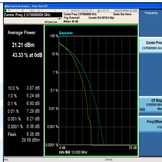
Band38-10MHz-64QAM-37800-50RB#0-PASS
