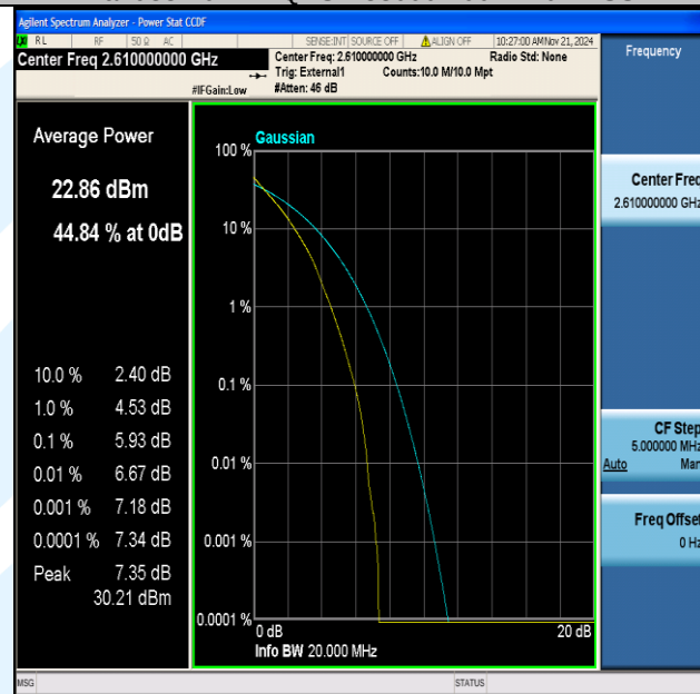
Band38-20MHz-QPSK-38150-100RB#0-PASS
