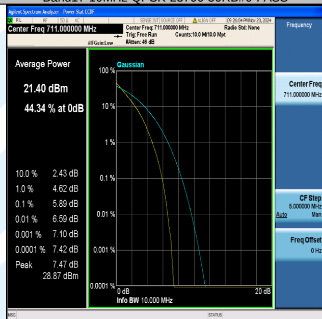
Band17-10MHz-QPSK-23800-50RB#0-PASS
