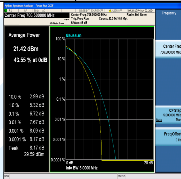
Band17-5MHz-64QAM-23755-25RB#0-PASS
