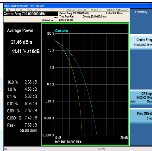
Band17-10MHz-QPSK-23790-50RB#0-PASS
