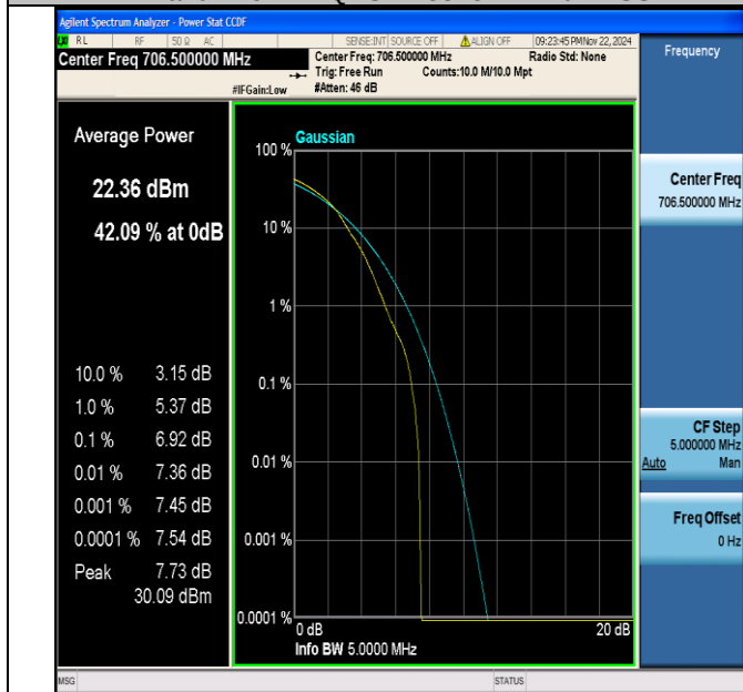
Band17-5MHz-64QAM-23755-1RB#0-PASS
