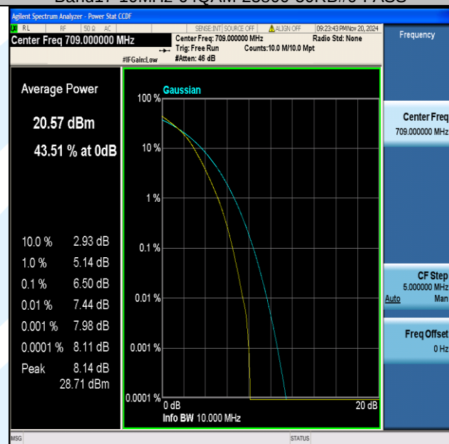
Band17-10MHz-16QAM-23780-50RB#0-PASS
