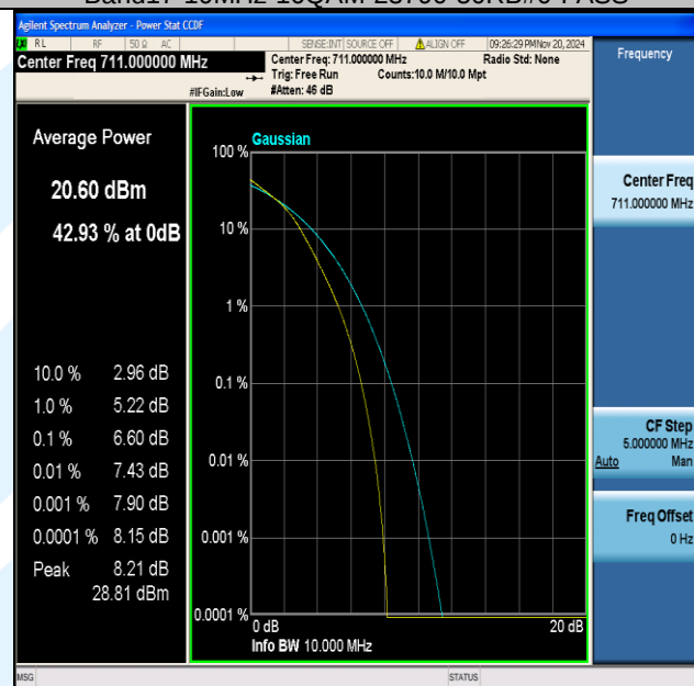
Band17-10MHz-16QAM-23800-50RB#0-PASS
