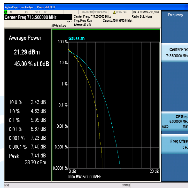
Band17-5MHz-QPSK-23825-25RB#0-PASS
