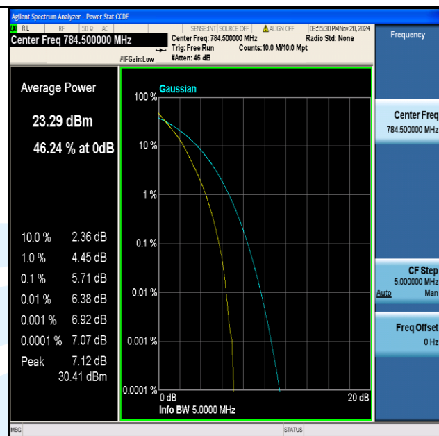
Band13-5MHz-QPSK-23255-25RB#0-PASS
