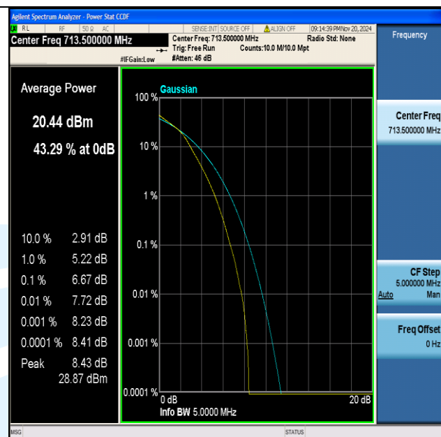
Band17-5MHz-16QAM-23825-25RB#0-PASS
