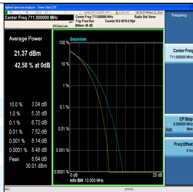
Band17-10MHz-64QAM-23800-50RB#0-PASS
