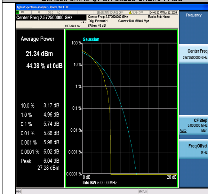
Band38-5MHz-64QAM-37775-1RB#0-PASS
