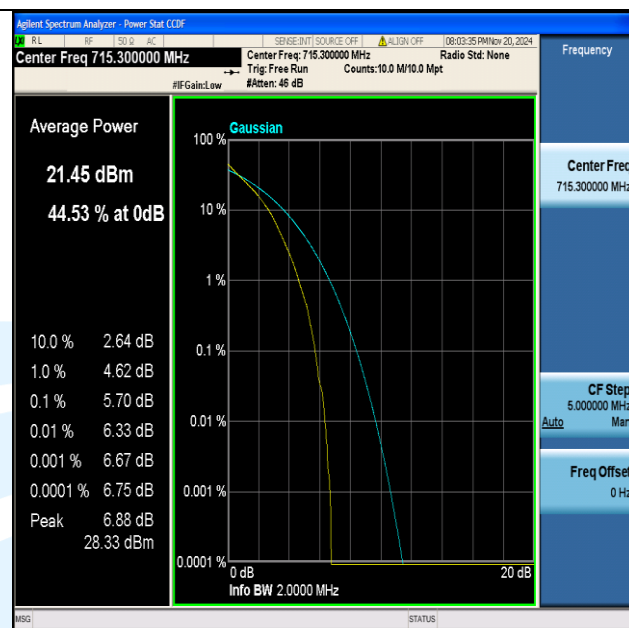
Band12-1.4MHz-QPSK-23173-6RB#0-PASS
