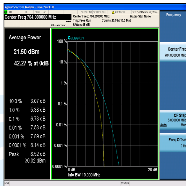
Band12-10MHz-64QAM-23060-50RB#0-PASS
