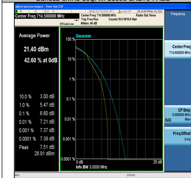
Band12-3MHz-16QAM-23165-1RB#0-PASS
