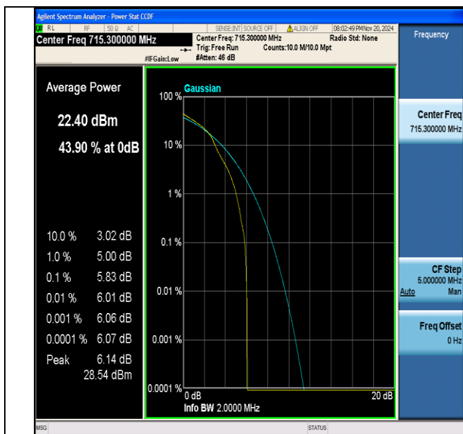
Band12-1.4MHz-16QAM-23173-1RB#0-PASS
