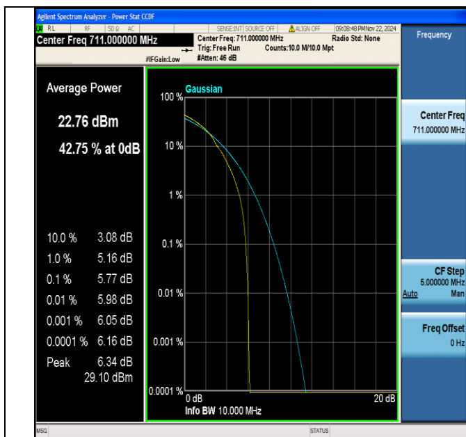
Band12-10MHz-64QAM-23130-1RB#0-PASS
