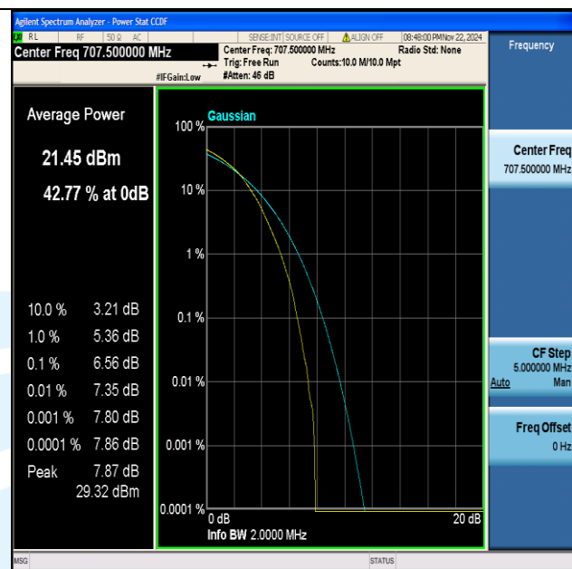
Band12-1.4MHz-64QAM-23095-6RB#0-PASS
