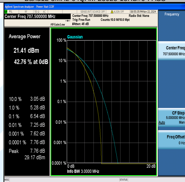
Band12-3MHz-64QAM-23095-15RB#0-PASS
