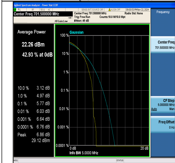
Band12-5MHz-64QAM-23035-1RB#0-PASS
