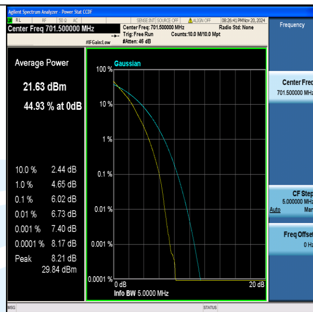
Band12-5MHz-QPSK-23035-25RB#0-PASS
