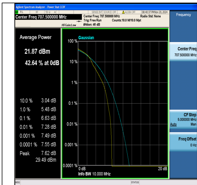
Band12-10MHz-16QAM-23095-1RB#0-PASS
