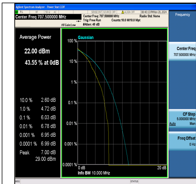
Band12-10MHz-QPSK-23095-1RB#0-PASS
