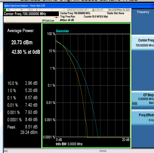
Band12-3MHz-16QAM-23025-15RB#0-PASS
