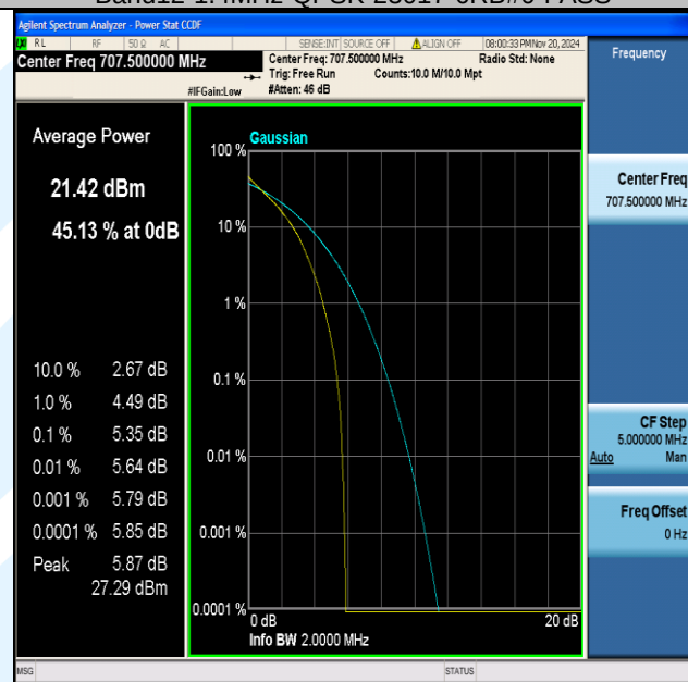
Band12-1.4MHz-QPSK-23095-6RB#0-PASS
