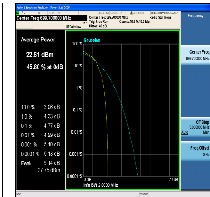
Band12-1.4MHz-16QAM-23017-1RB#0-PASS
