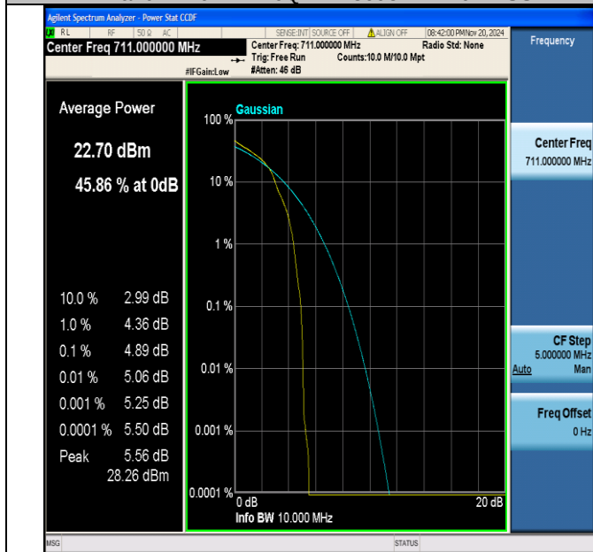
Band12-10MHz-16QAM-23130-1RB#0-PASS
