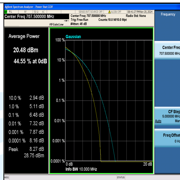
Band12-10MHz-16QAM-23095-50RB#0-PASS
