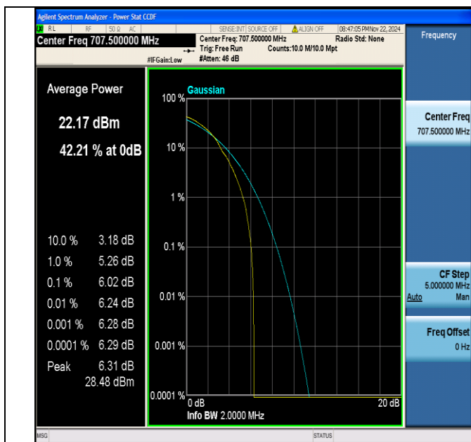
Band12-1.4MHz-64QAM-23095-1RB#0-PASS
