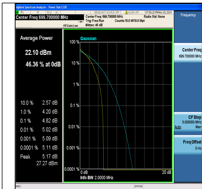
Band12-1.4MHz-QPSK-23017-1RB#0-PASS
