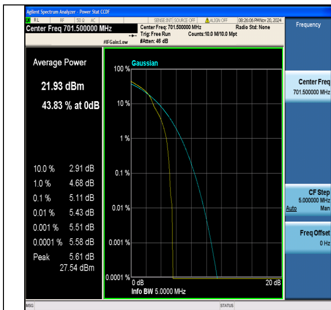
Band12-5MHz-16QAM-23035-1RB#0-PASS
