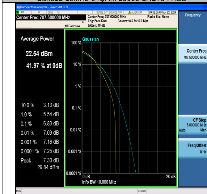
Band12-10MHz-64QAM-23095-1RB#0-PASS
