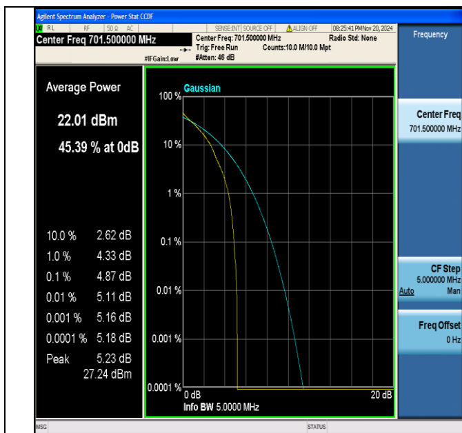
Band12-5MHz-QPSK-23035-1RB#0-PASS
