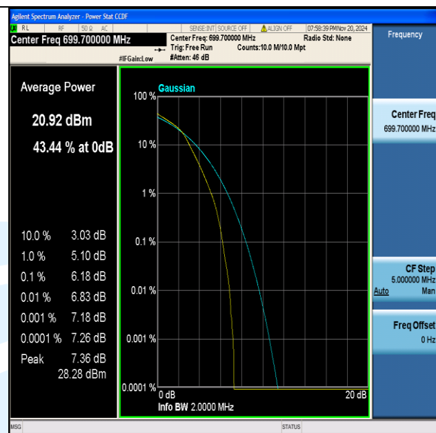
Band12-1.4MHz-16QAM-23017-6RB#0-PASS
