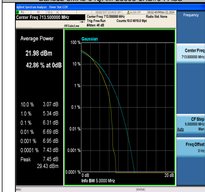
Band12-5MHz-64QAM-23155-1RB#0-PASS
