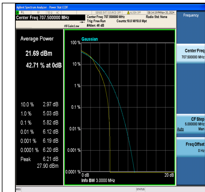
Band12-3MHz-16QAM-23095-1RB#0-PASS
