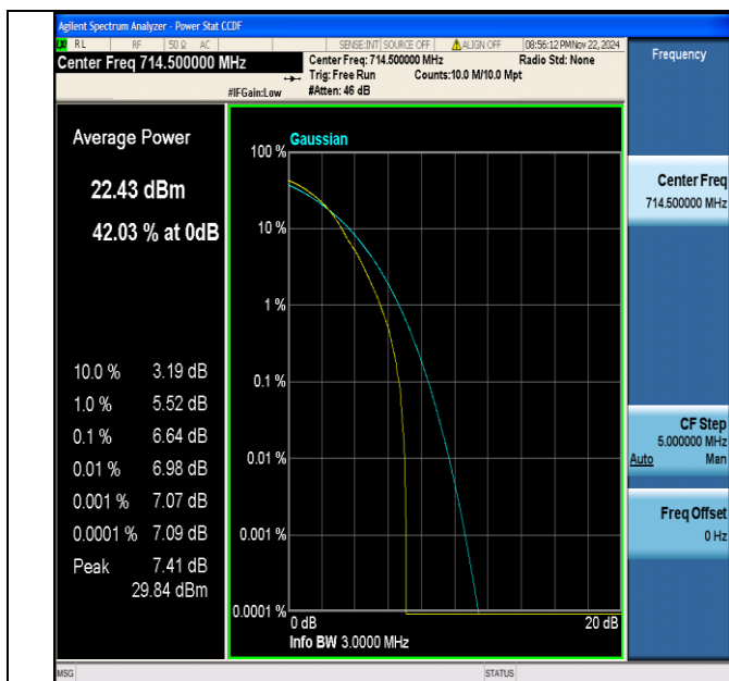
Band12-3MHz-64QAM-23165-1RB#0-PASS
