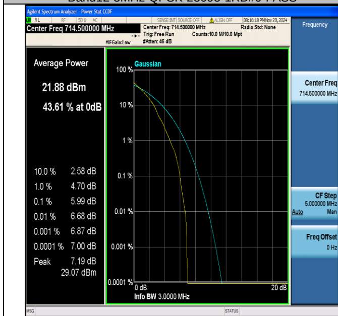
Band12-3MHz-QPSK-23165-1RB#0-PASS
