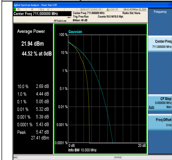
Band12-10MHz-QPSK-23130-1RB#0-PASS
