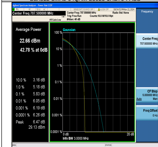
Band12-3MHz-64QAM-23095-1RB#0-PASS
