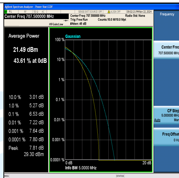
Band12-5MHz-64QAM-23095-25RB#0-PASS
