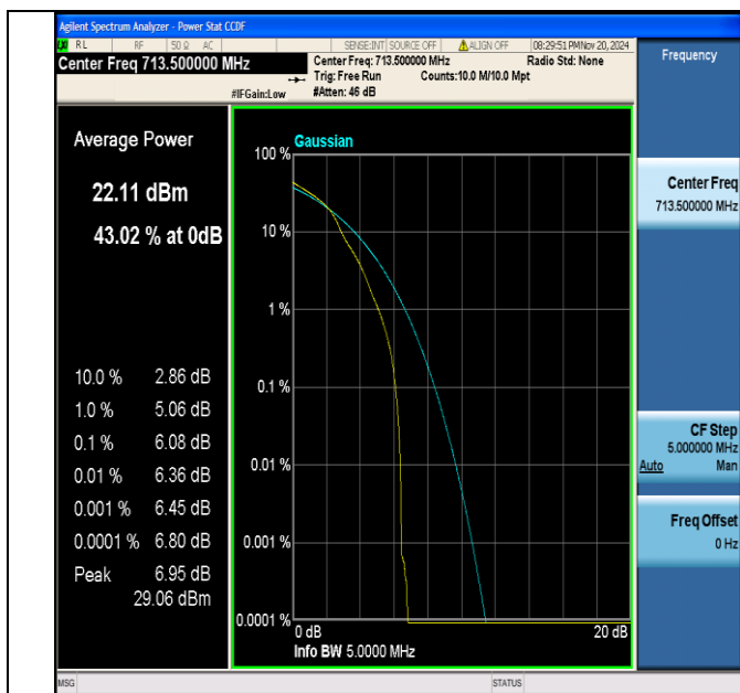
Band12-5MHz-16QAM-23155-1RB#0-PASS
