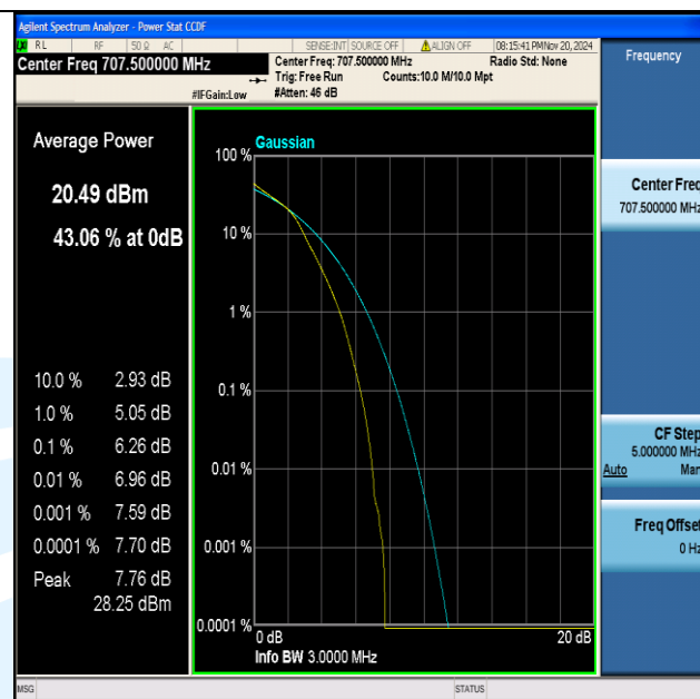
Band12-3MHz-16QAM-23095-15RB#0-PASS
