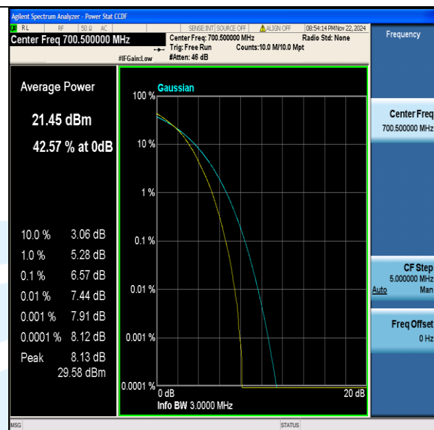
Band12-3MHz-64QAM-23025-15RB#0-PASS
