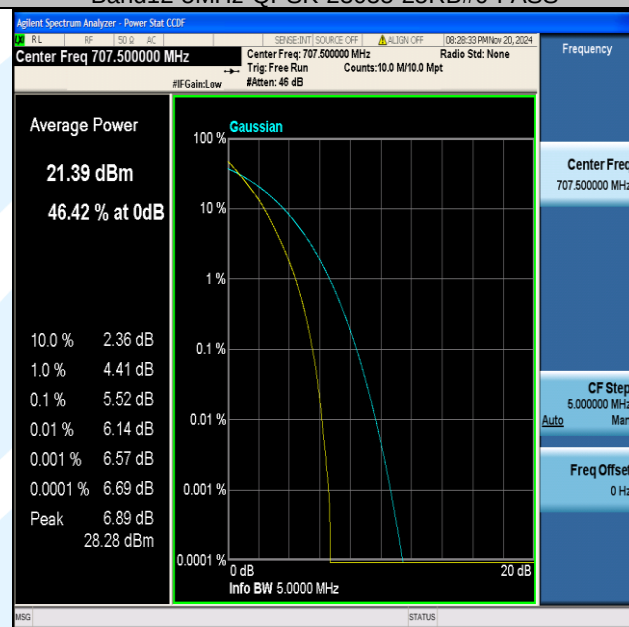
Band12-5MHz-QPSK-23095-25RB#0-PASS
