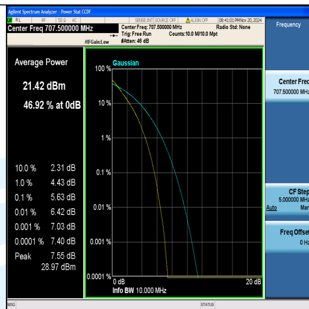
Band12-10MHz-QPSK-23095-50RB#0-PASS
