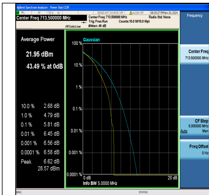
Band12-5MHz-QPSK-23155-1RB#0-PASS
