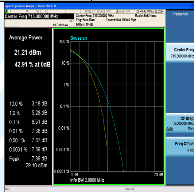
Band12-1.4MHz-64QAM-23173-6RB#0-PASS
