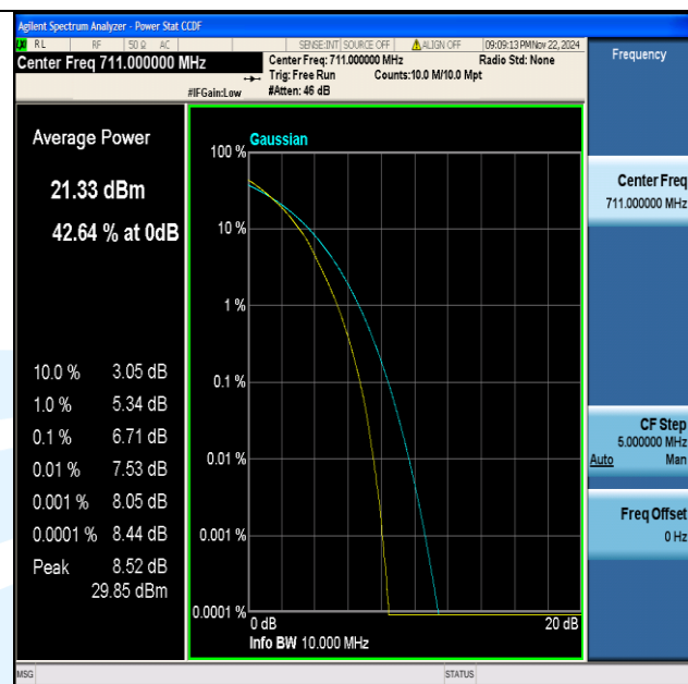
Band12-10MHz-64QAM-23130-50RB#0-PASS
