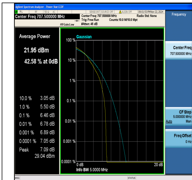
Band12-5MHz-64QAM-23095-1RB#0-PASS
