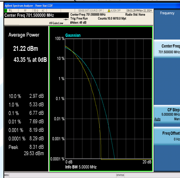
Band12-5MHz-64QAM-23035-25RB#0-PASS
