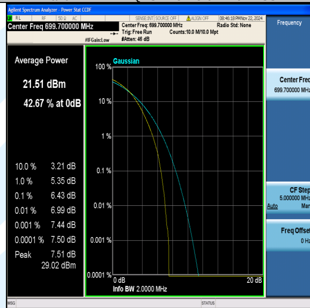
Band12-1.4MHz-64QAM-23017-6RB#0-PASS
