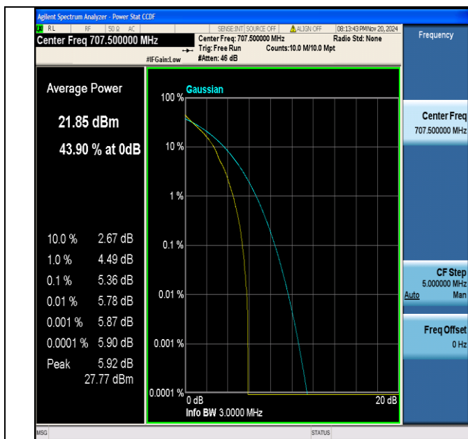
Band12-3MHz-QPSK-23095-1RB#0-PASS
