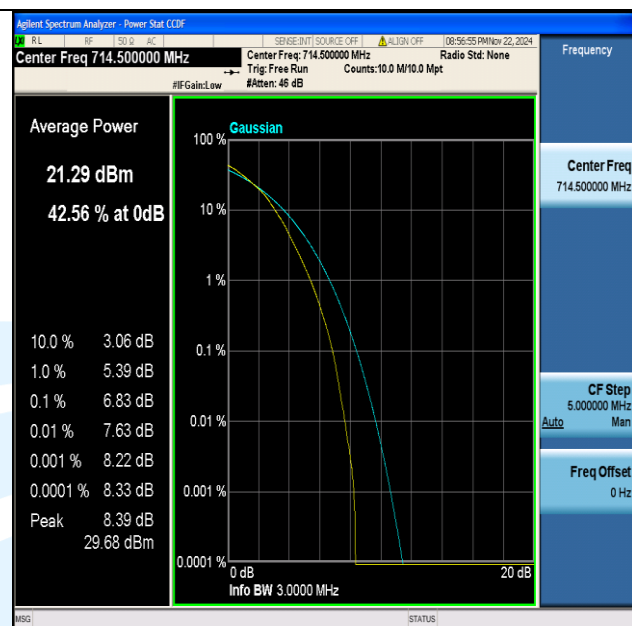
Band12-3MHz-64QAM-23165-15RB#0-PASS
