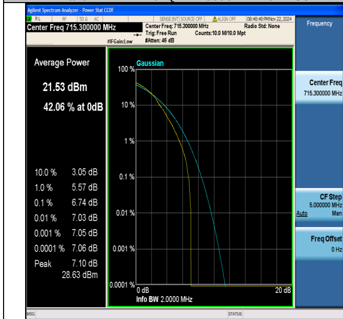
Band12-1.4MHz-64QAM-23173-1RB#0-PASS
