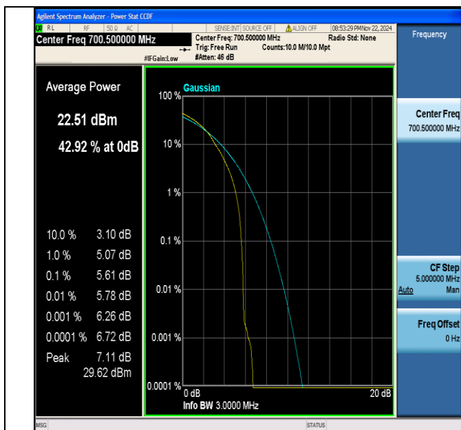
Band12-3MHz-64QAM-23025-1RB#0-PASS
