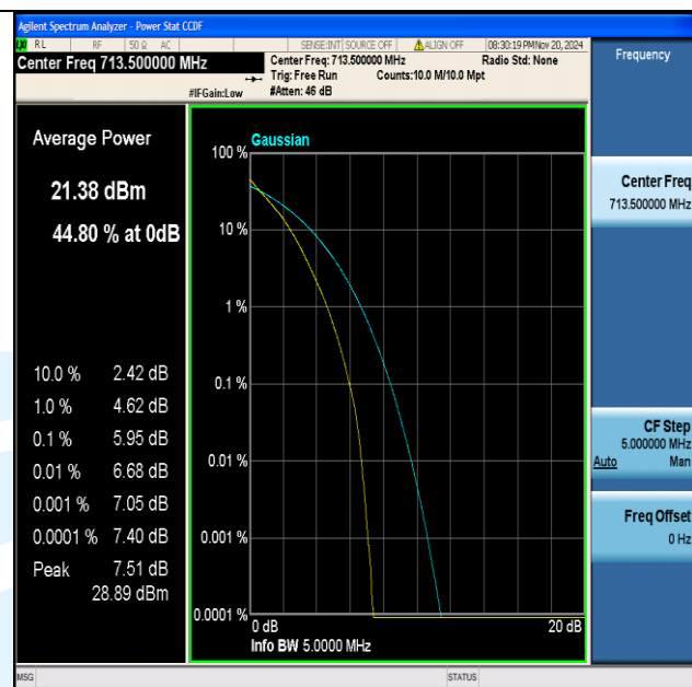
Band12-5MHz-QPSK-23155-25RB#0-PASS
