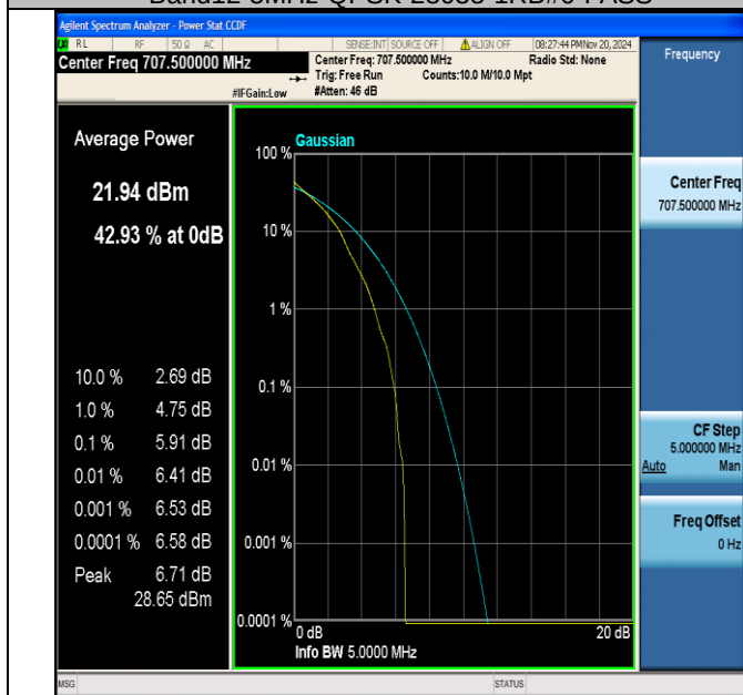
Band12-5MHz-QPSK-23095-1RB#0-PASS
