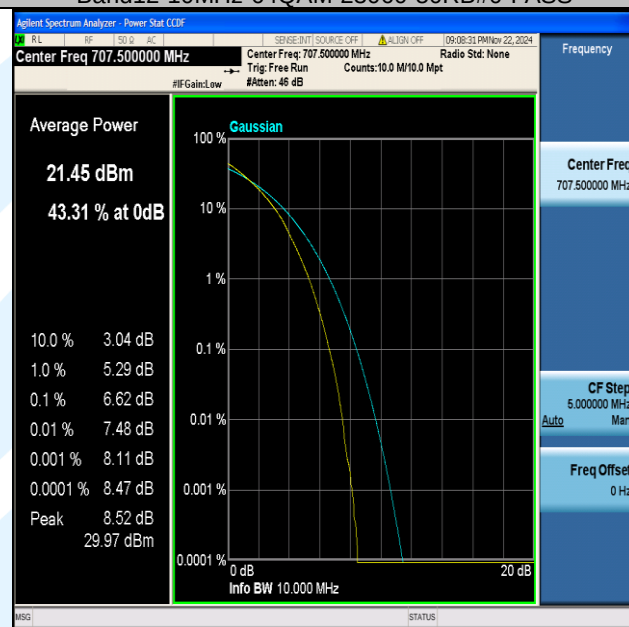
Band12-10MHz-64QAM-23095-50RB#0-PASS
