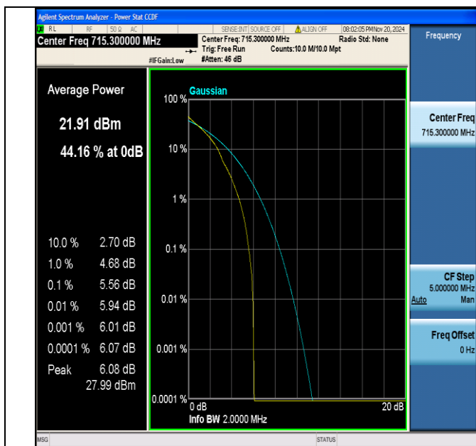
Band12-1.4MHz-QPSK-23173-1RB#0-PASS
