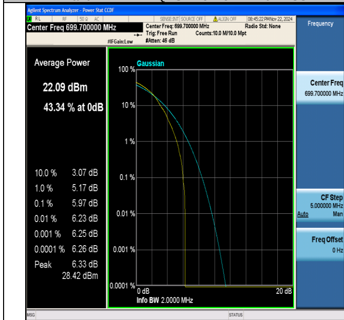
Band12-1.4MHz-64QAM-23017-1RB#0-PASS
