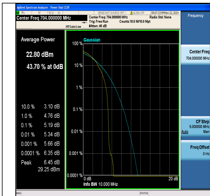
Band12-10MHz-64QAM-23060-1RB#0-PASS
