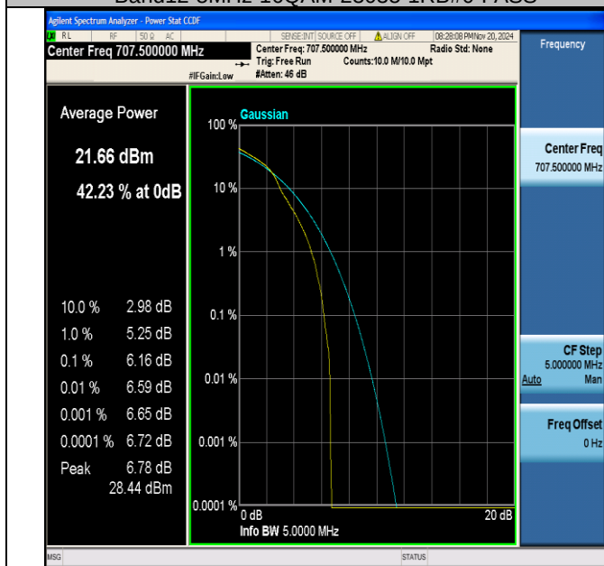
Band12-5MHz-16QAM-23095-1RB#0-PASS
