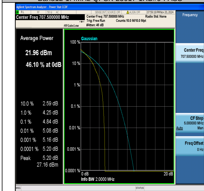
Band12-1.4MHz-QPSK-23095-1RB#0-PASS
