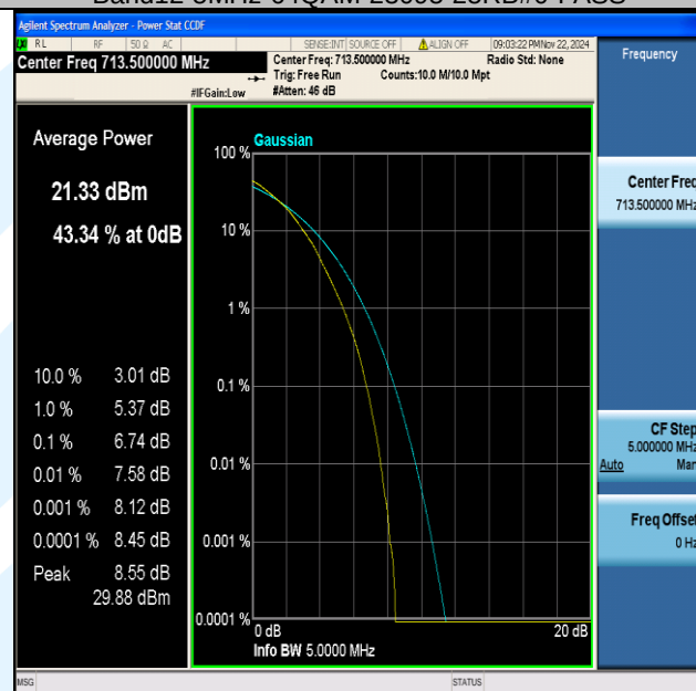
Band12-5MHz-64QAM-23155-25RB#0-PASS
