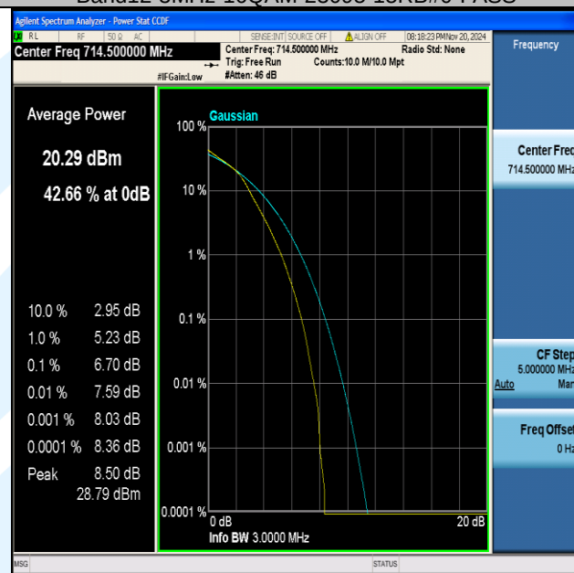
Band12-3MHz-16QAM-23165-15RB#0-PASS
