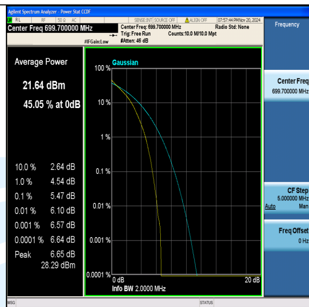
Band12-1.4MHz-QPSK-23017-6RB#0-PASS
