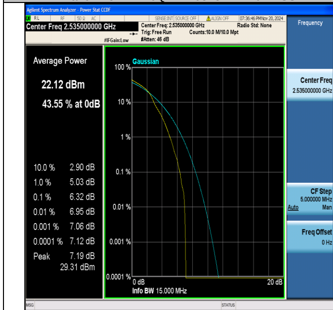
Band7-15MHz-16QAM-21100-1RB#0-PASS
