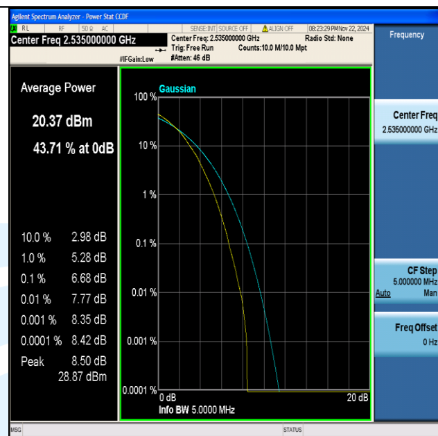
Band7-5MHz-64QAM-21100-25RB#0-PASS
