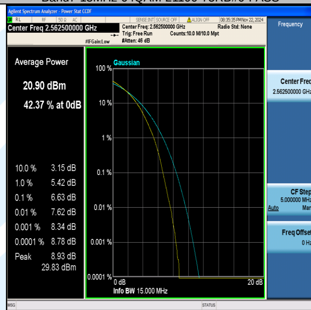
Band7-15MHz-64QAM-21375-75RB#0-PASS
