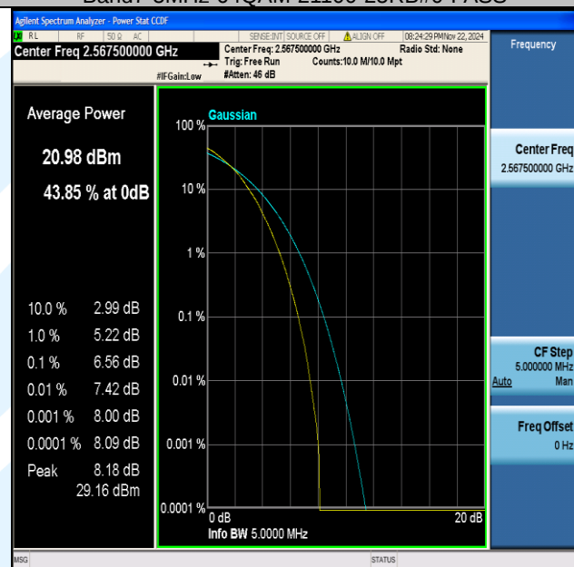
Band7-5MHz-64QAM-21425-25RB#0-PASS
