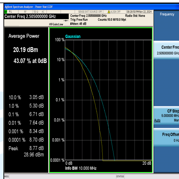
Band7-10MHz-64QAM-20800-50RB#0-PASS
