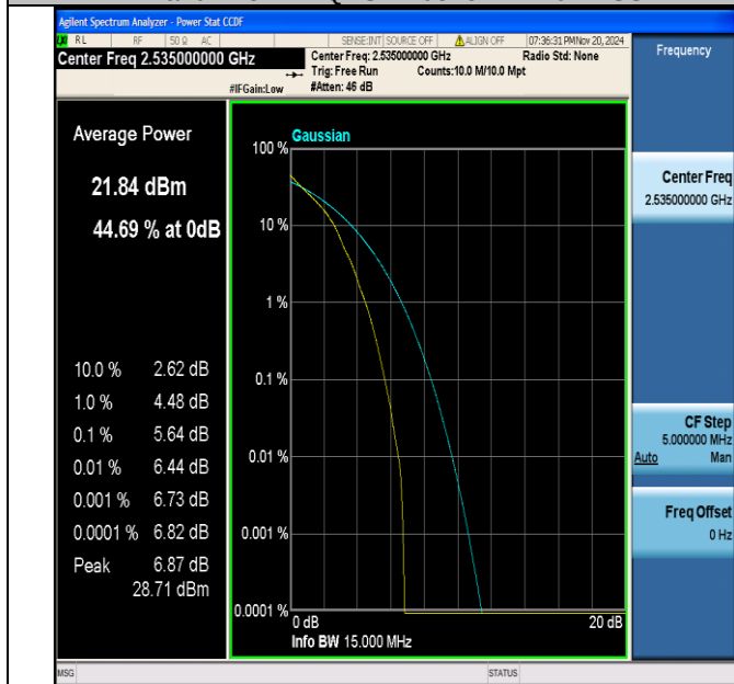
Band7-15MHz-QPSK-21100-1RB#0-PASS
