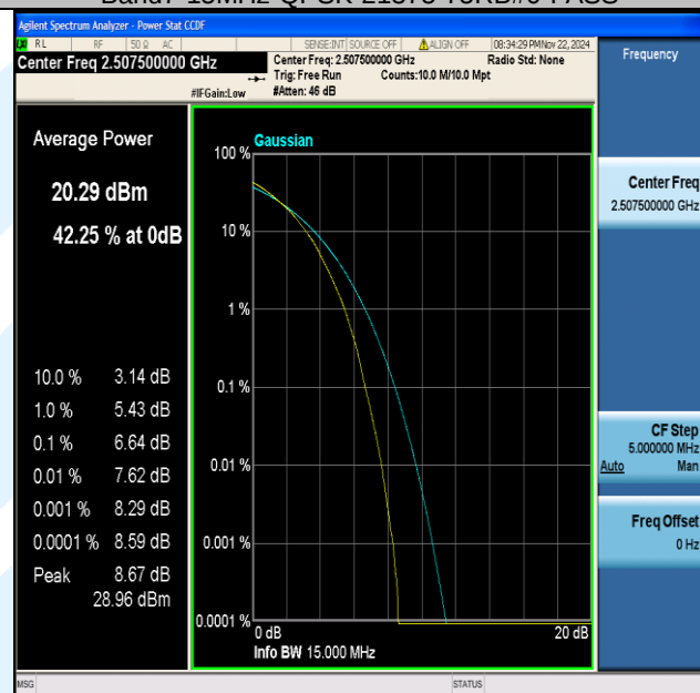
Band7-15MHz-64QAM-20825-75RB#0-PASS
