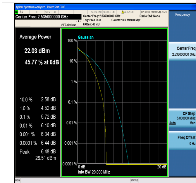
Band7-20MHz-QPSK-21100-1RB#0-PASS
