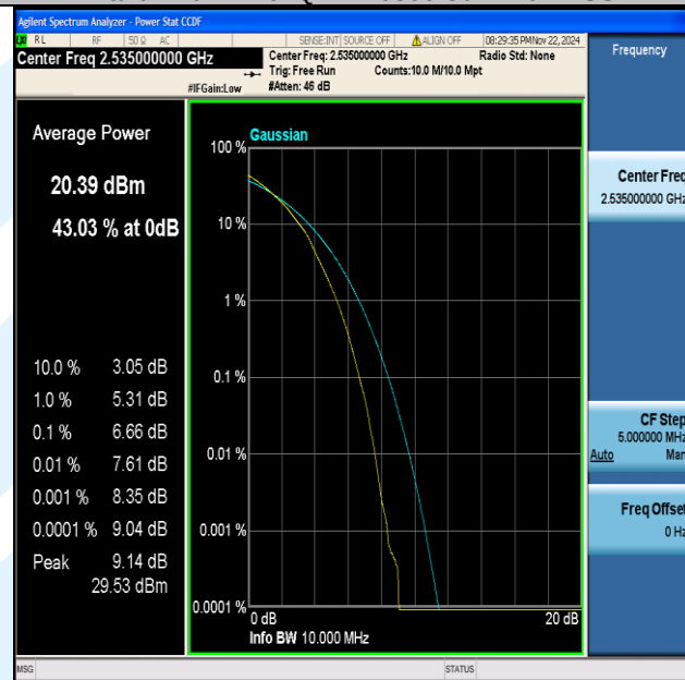
Band7-10MHz-64QAM-21100-50RB#0-PASS
