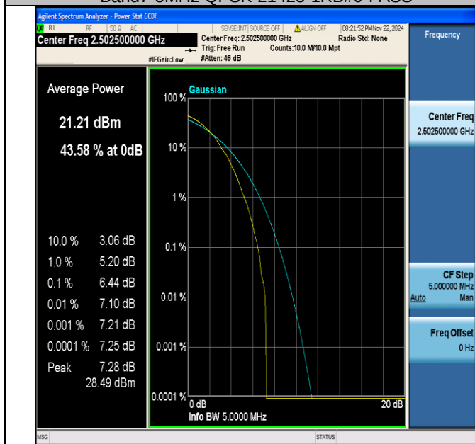
Band7-5MHz-64QAM-20775-1RB#0-PASS
