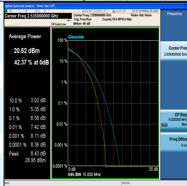
Band7-15MHz-16QAM-21100-75RB#0-PASS
