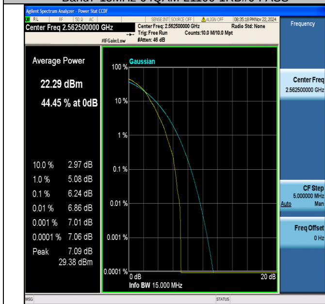
Band7-15MHz-64QAM-21375-1RB#0-PASS
