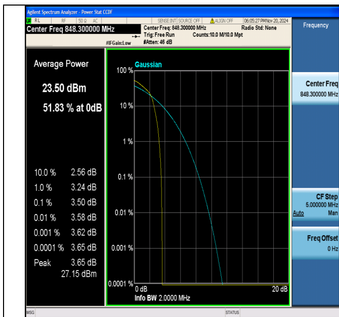
Band5-1.4MHz-16QAM-20643-1RB#0-PASS
