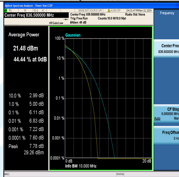
Band5-10MHz-64QAM-20525-50RB#0-PASS
