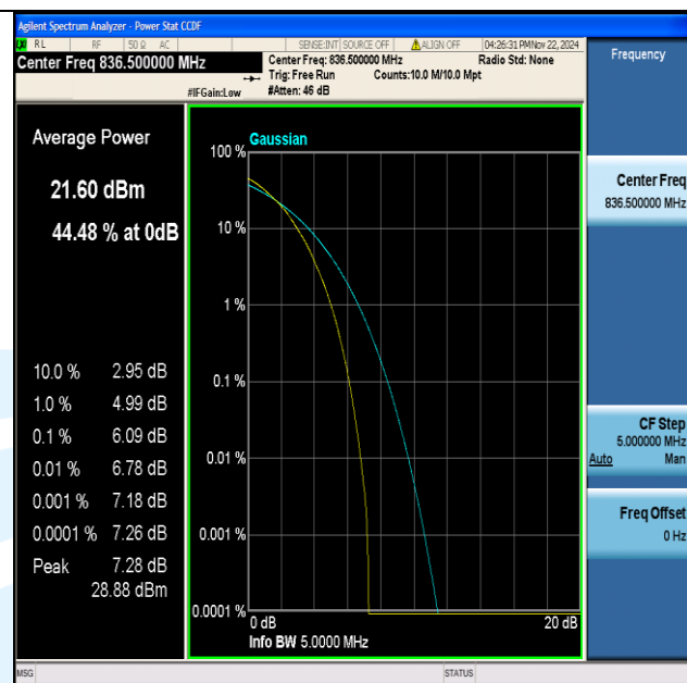
Band5-5MHz-64QAM-20525-25RB#0-PASS
