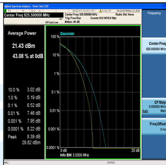
Band5-3MHz-64QAM-20415-15RB#0-PASS
