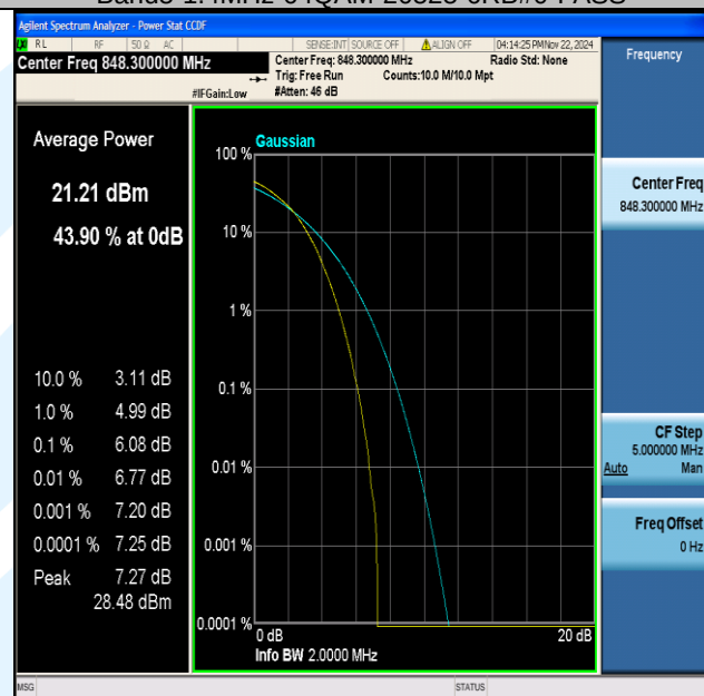
Band5-1.4MHz-64QAM-20643-6RB#0-PASS
