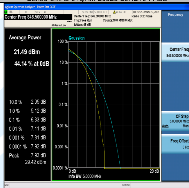
Band5-5MHz-64QAM-20625-25RB#0-PASS
