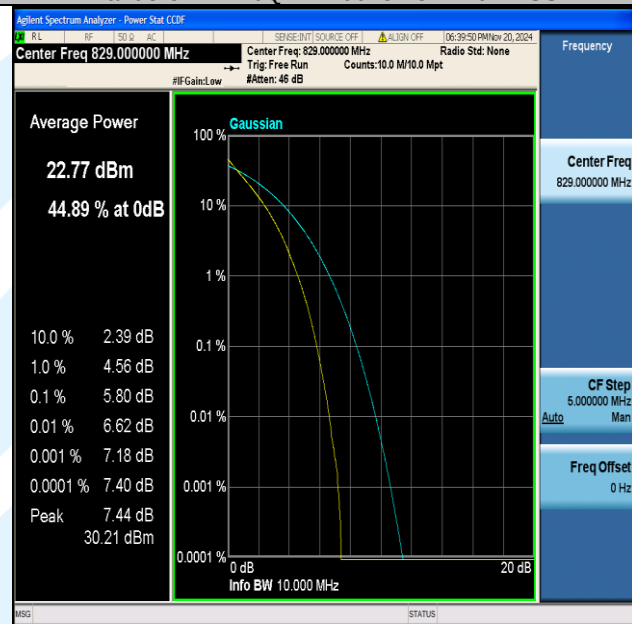
Band5-10MHz-QPSK-20450-50RB#0-PASS
