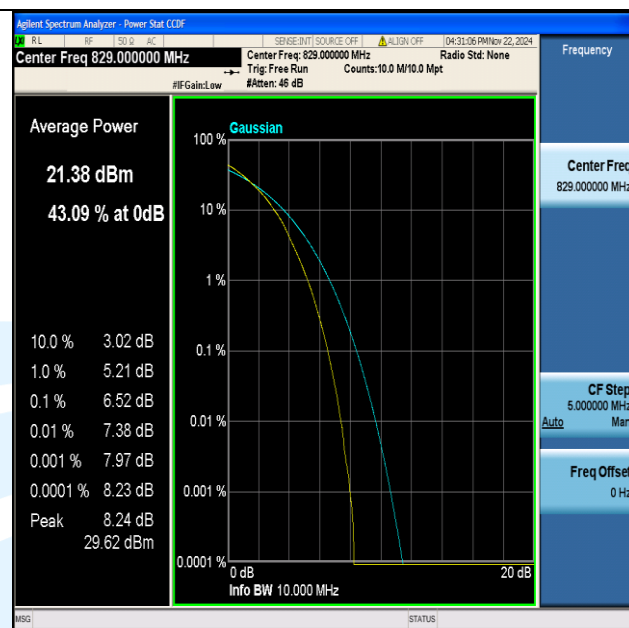
Band5-10MHz-64QAM-20450-50RB#0-PASS
