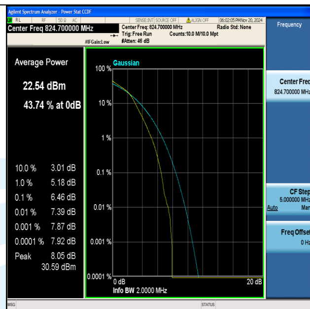
Band5-1.4MHz-16QAM-20407-6RB#0-PASS
