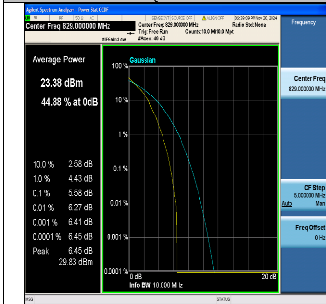
Band5-10MHz-QPSK-20450-1RB#0-PASS
