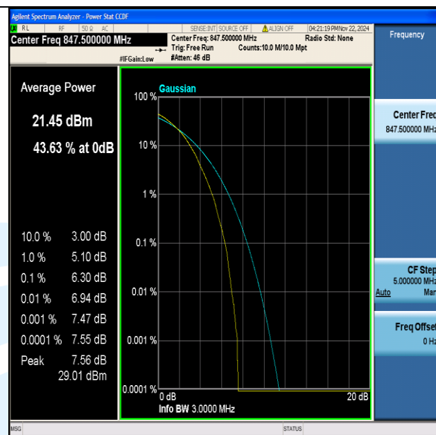
Band5-3MHz-64QAM-20635-15RB#0-PASS
