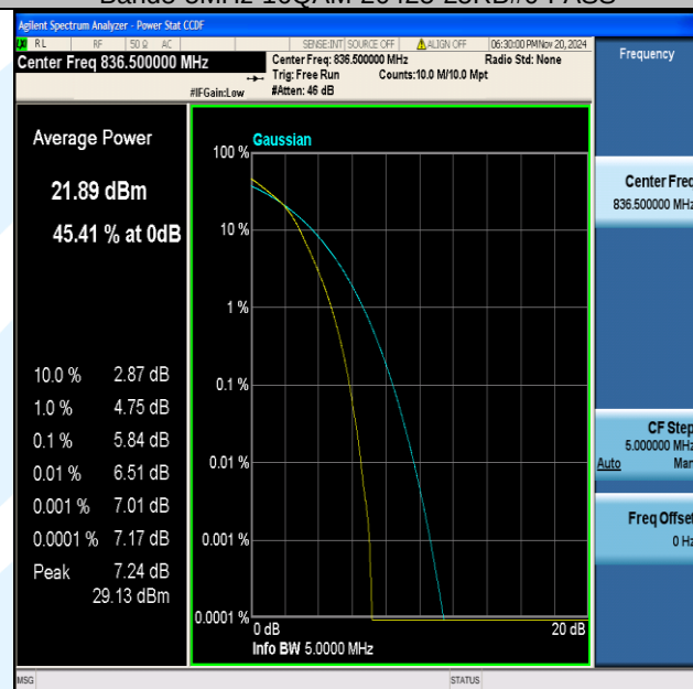
Band5-5MHz-16QAM-20525-25RB#0-PASS
