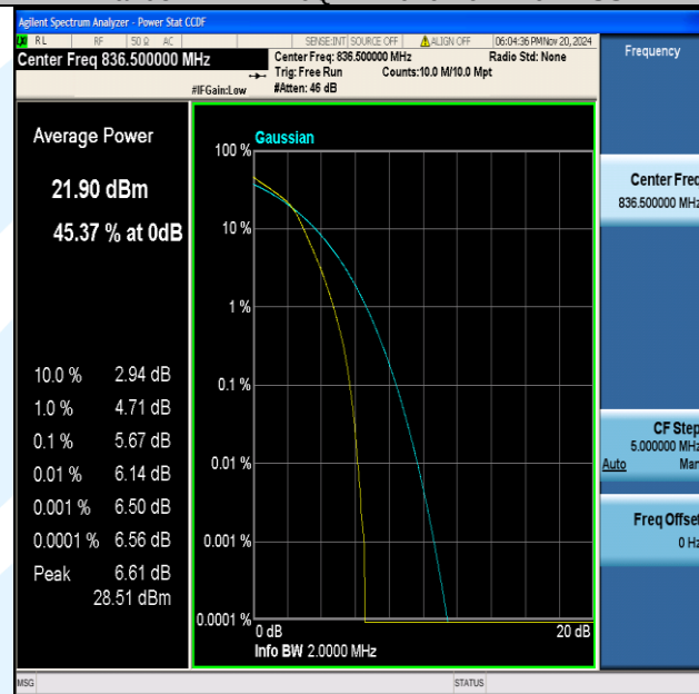
Band5-1.4MHz-16QAM-20525-6RB#0-PASS
