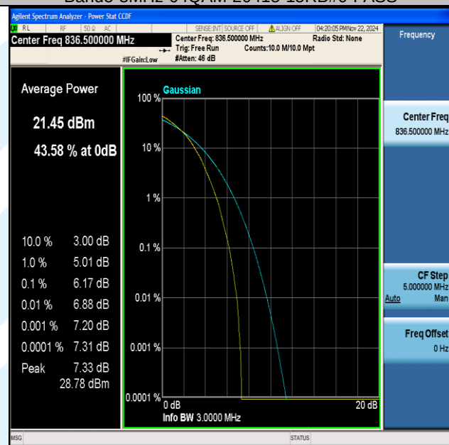
Band5-3MHz-64QAM-20525-15RB#0-PASS
