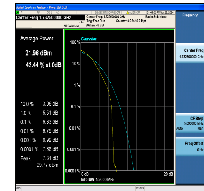
Band4-15MHz-64QAM-20175-1RB#0-PASS
