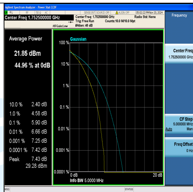
Band4-5MHz-QPSK-20375-25RB#0-PASS
