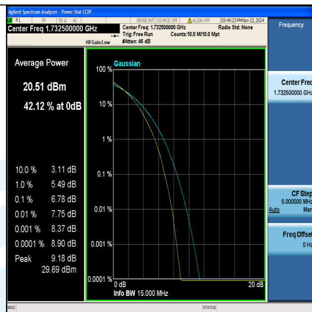
Band4-15MHz-64QAM-20175-75RB#0-PASS
