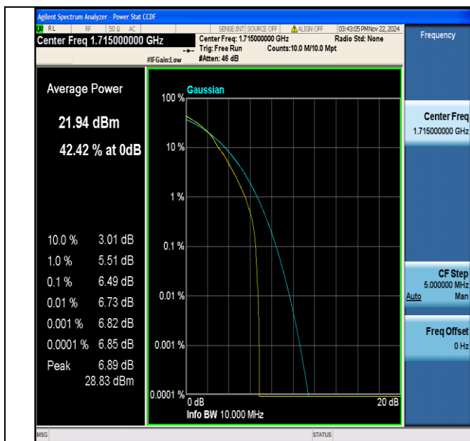
Band4-10MHz-64QAM-20000-1RB#0-PASS
