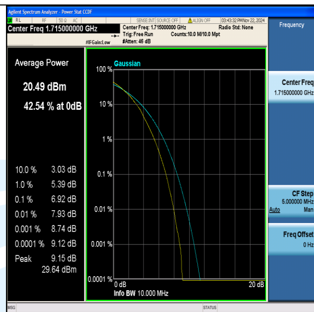
Band4-10MHz-64QAM-20000-50RB#0-PASS
