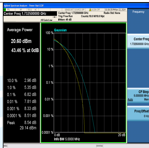
Band4-5MHz-64QAM-20175-25RB#0-PASS
