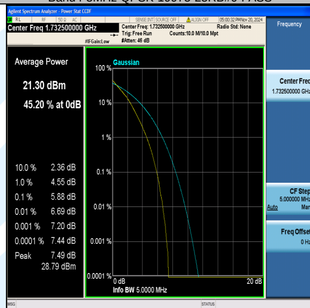
Band4-5MHz-QPSK-20175-25RB#0-PASS
