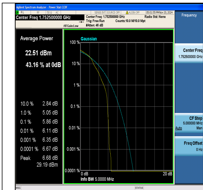
Band4-5MHz-16QAM-20375-1RB#0-PASS
