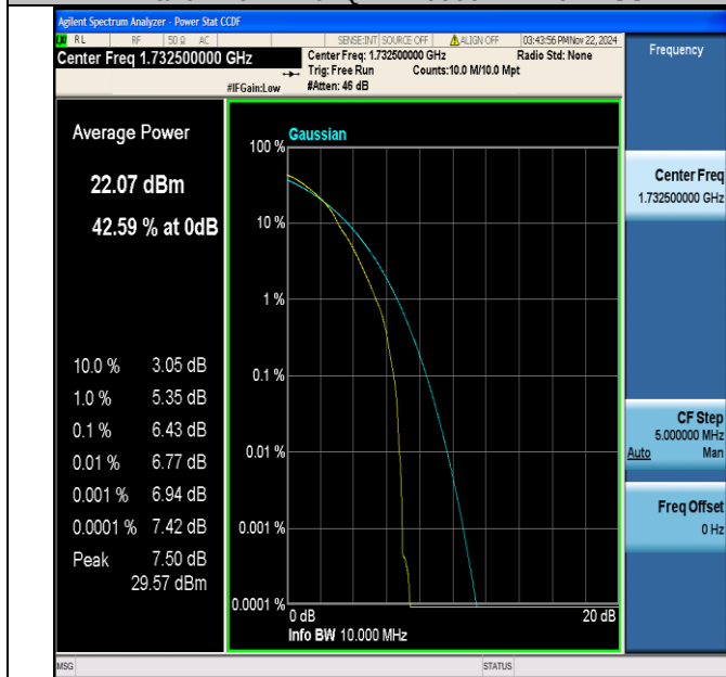
Band4-10MHz-64QAM-20175-1RB#0-PASS
