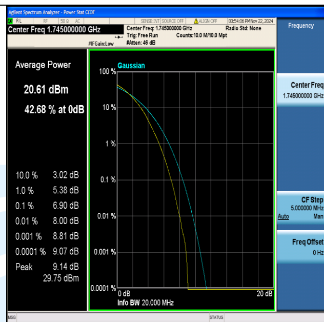
Band4-20MHz-64QAM-20300-100RB#0-PASS
