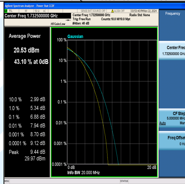
Band4-20MHz-64QAM-20175-100RB#0-PASS
