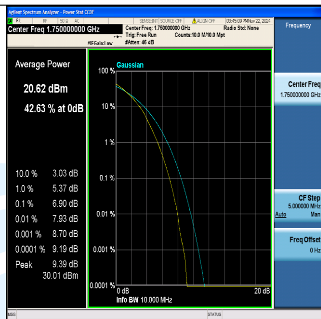
Band4-10MHz-64QAM-20350-50RB#0-PASS
