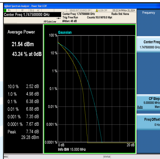
Band4-15MHz-QPSK-20325-75RB#0-PASS
