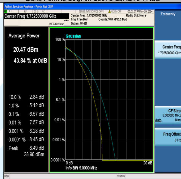
Band4-5MHz-16QAM-20175-25RB#0-PASS
