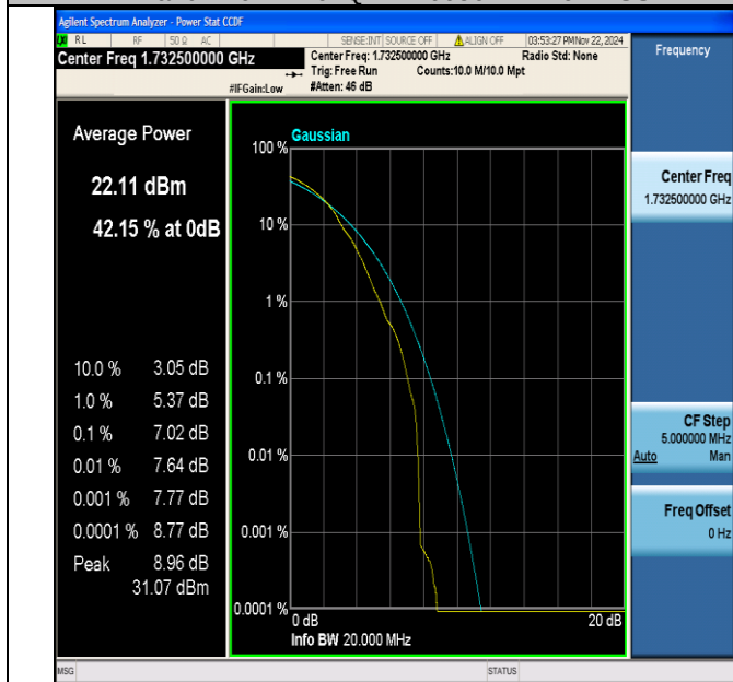
Band4-20MHz-64QAM-20175-1RB#0-PASS
