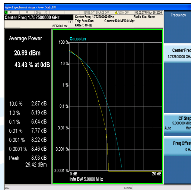
Band4-5MHz-16QAM-20375-25RB#0-PASS
