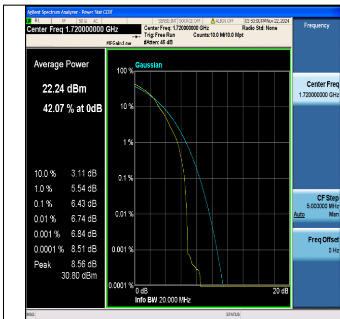
Band4-20MHz-64QAM-20050-1RB#0-PASS
