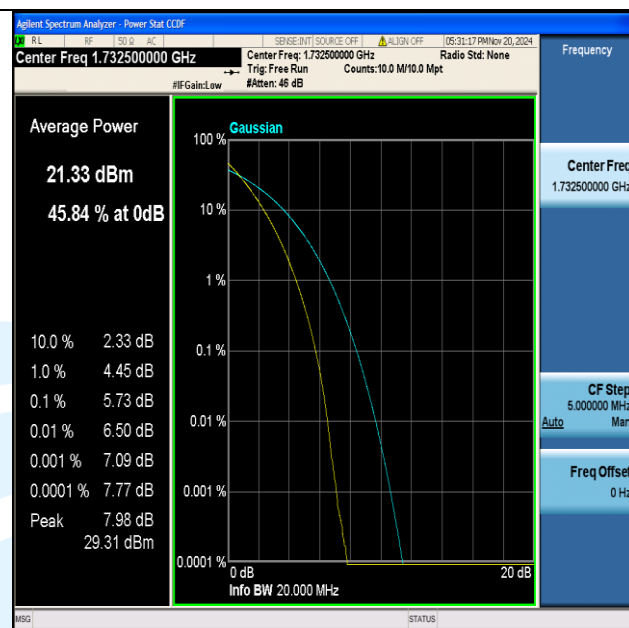
Band4-20MHz-QPSK-20175-100RB#0-PASS
