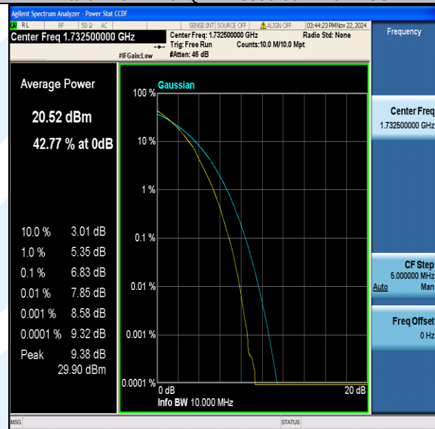
Band4-10MHz-64QAM-20175-50RB#0-PASS
