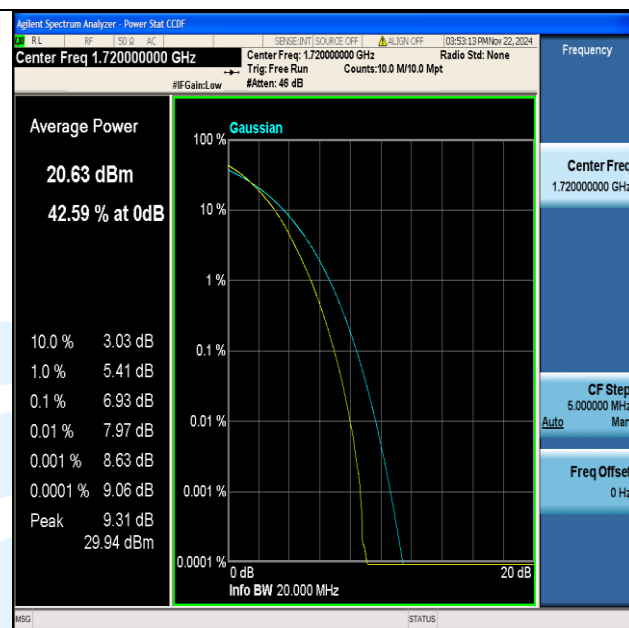
Band4-20MHz-64QAM-20050-100RB#0-PASS
