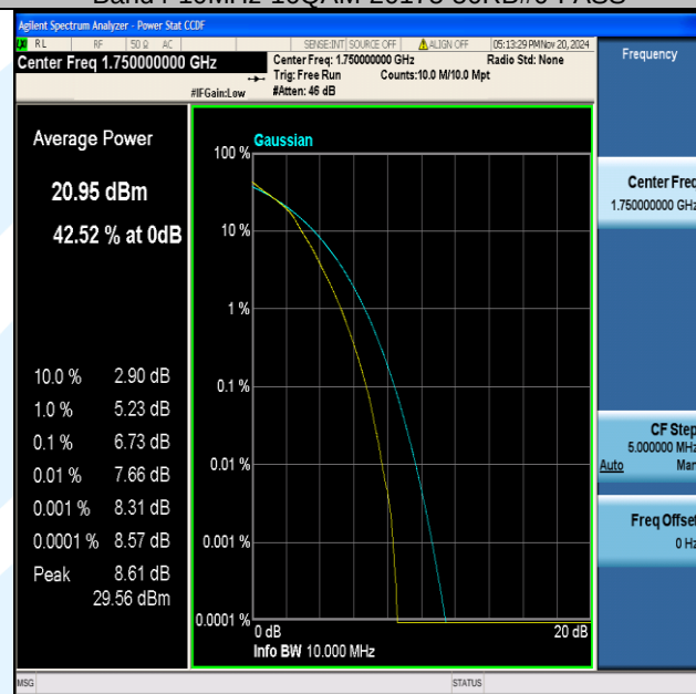
Band4-10MHz-16QAM-20350-50RB#0-PASS
