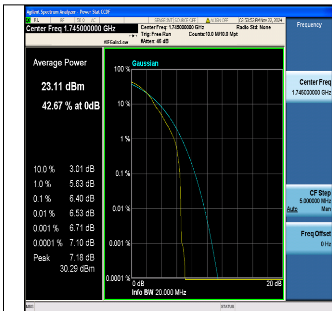
Band4-20MHz-64QAM-20300-1RB#0-PASS
