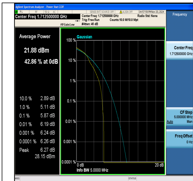
Band4-5MHz-16QAM-19975-1RB#0-PASS
