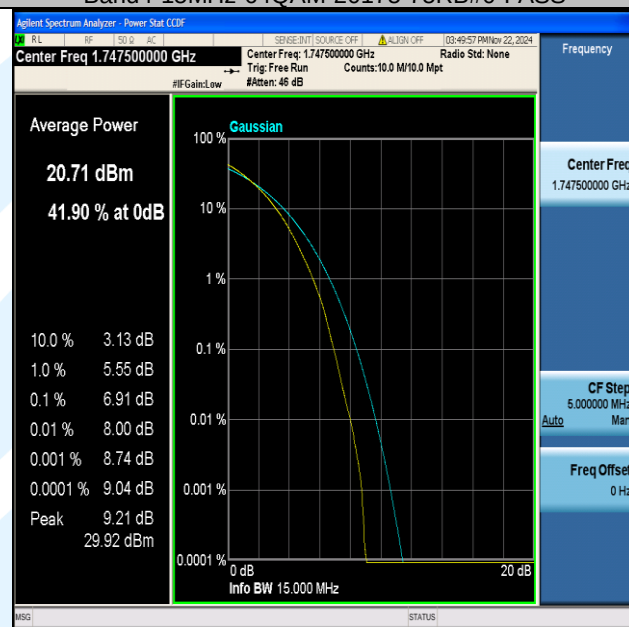
Band4-15MHz-64QAM-20325-75RB#0-PASS
