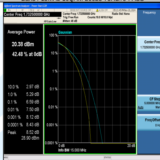
Band4-15MHz-16QAM-20175-75RB#0-PASS
