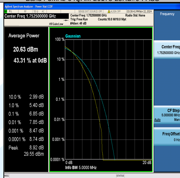
Band4-5MHz-64QAM-20375-25RB#0-PASS
