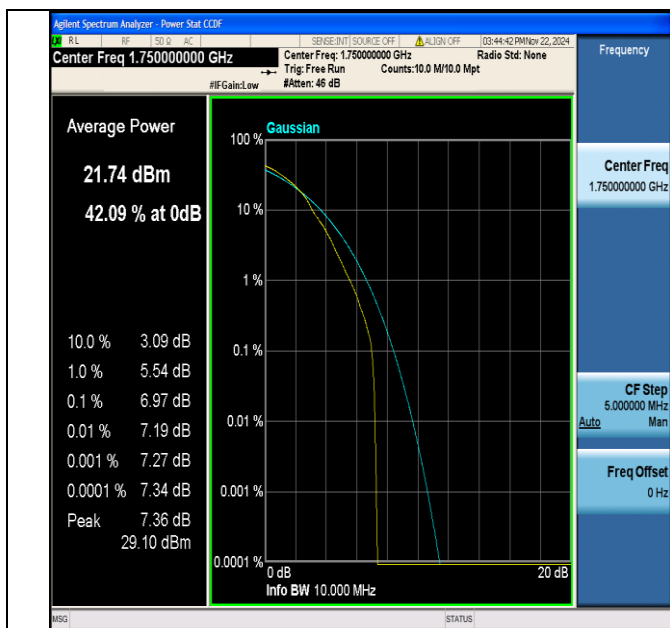
Band4-10MHz-64QAM-20350-1RB#0-PASS
