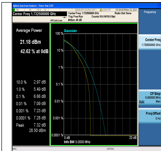
Band4-5MHz-64QAM-20175-1RB#0-PASS
