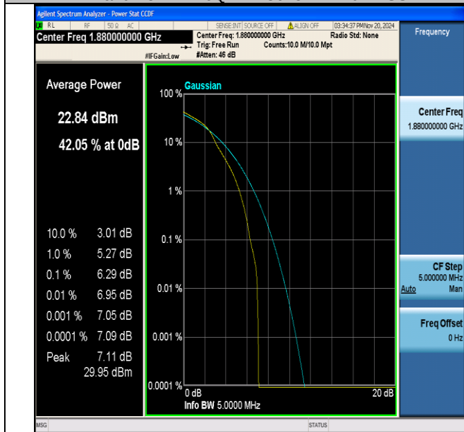
Band2-5MHz-16QAM-18900-1RB#0-PASS
