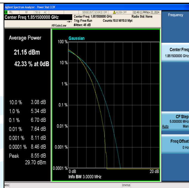
Band2-3MHz-64QAM-18615-15RB#0-PASS
