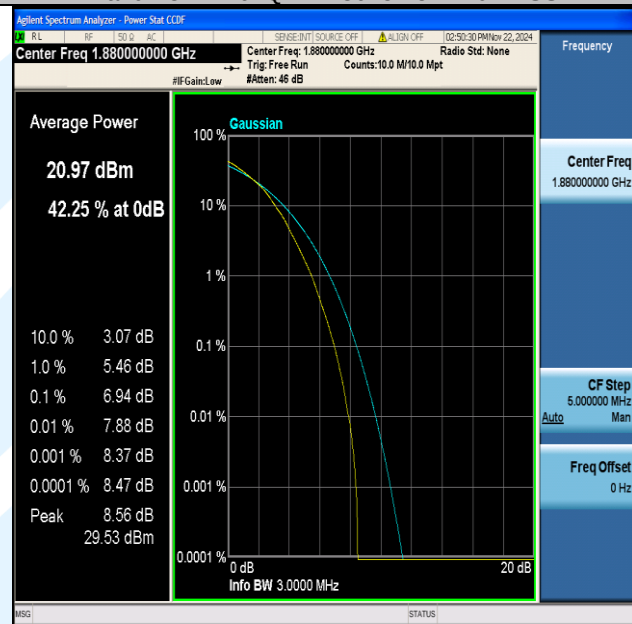
Band2-3MHz-64QAM-18900-15RB#0-PASS
