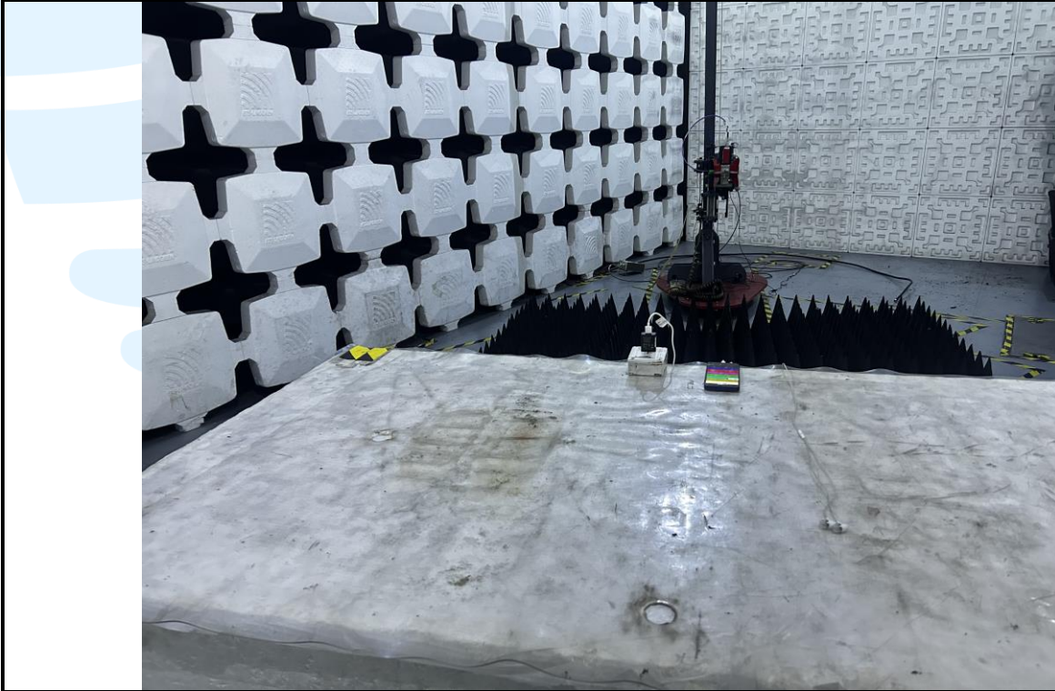
Radiated emission Test Setup-2 (Above 1 GHz)
