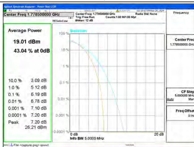
B66 / 3MHz / High CH / 64QAM
