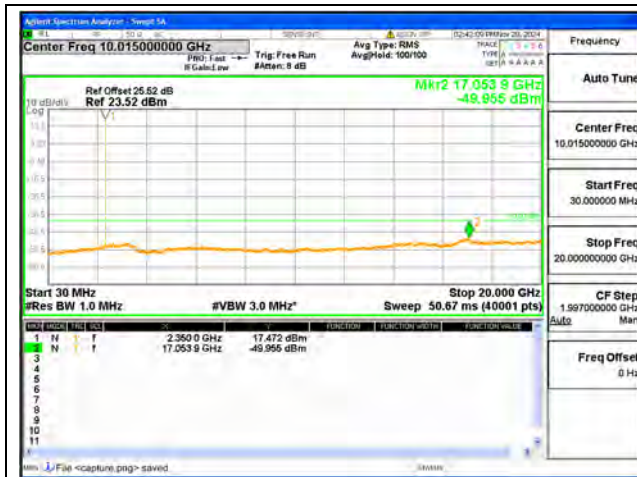
B40-2-30M-20G / 5MHz / Low CH / QPSK
