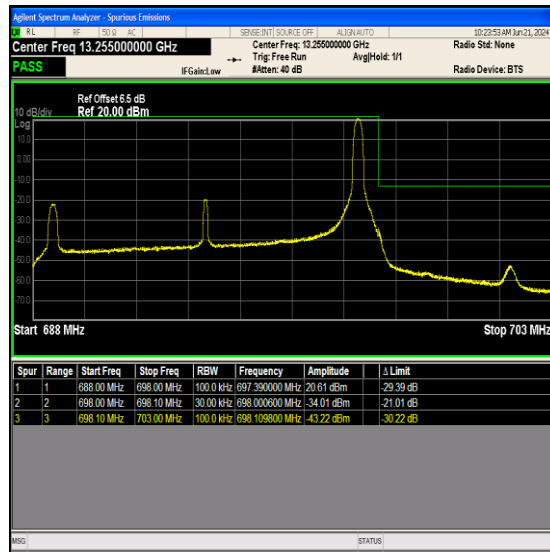
Band71_10MHz_16QAM_133422_1RB#49
