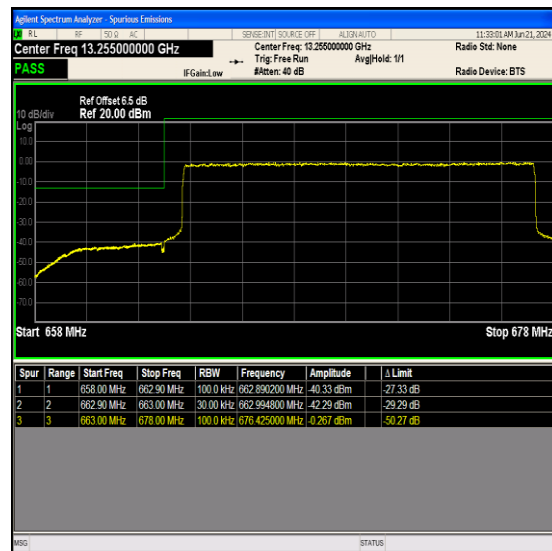
Band71_15MHz_16QAM_133197_75RB#0
