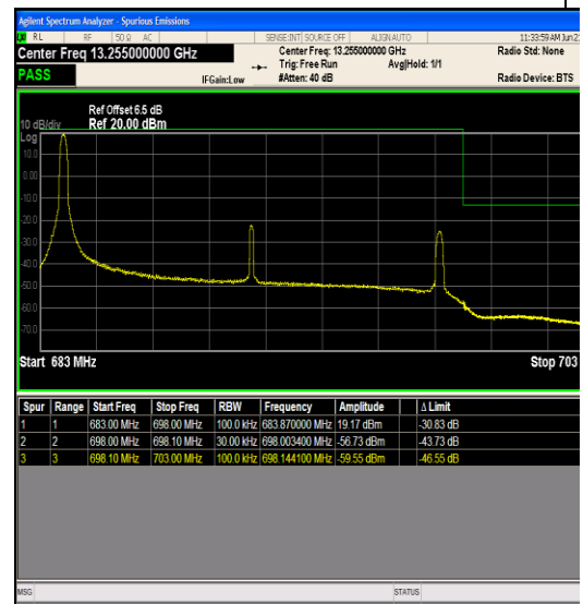
Band71_15MHz_64QAM_133397_1RB#0
