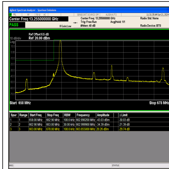
Band71_15MHz_16QAM_133197_1RB#0
