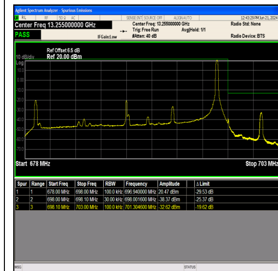
Band71_20MHz_16QAM_133372_1RB#99
