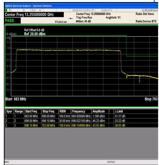
Band71_15MHz_64QAM_133397_75RB#0
