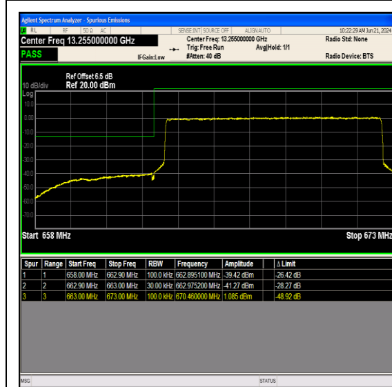
Band71_10MHz_16QAM_133172_1RB#0
