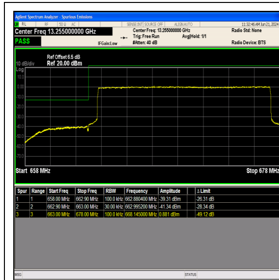
Band71_15MHz_QPSK_133197_75RB#0
