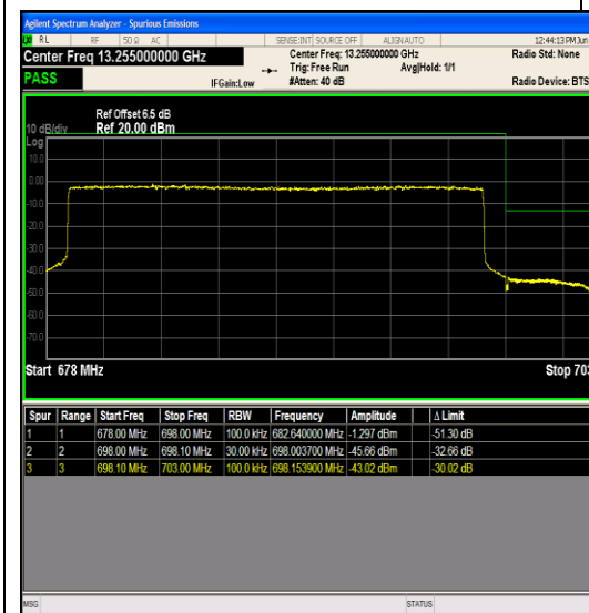
Band71_20MHz_16QAM_133372_100RB#0
