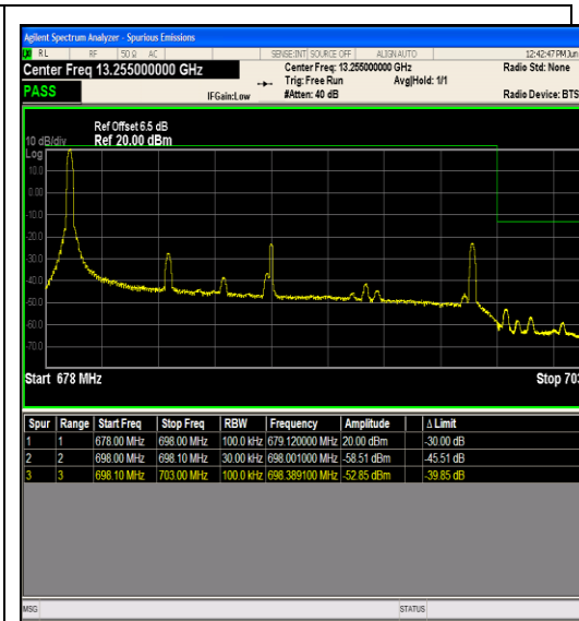
Band71_20MHz_16QAM_133372_1RB#0
