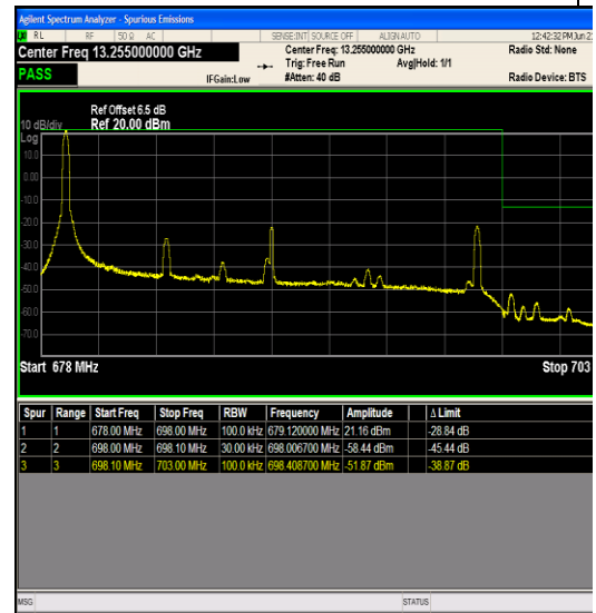
Band71_20MHz_QPSK_133372_1RB#0
