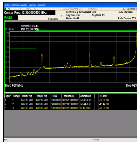
Band71_20MHz_16QAM_133222_1RB#99
