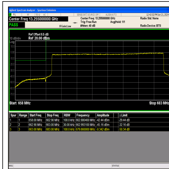
Band71_20MHz_16QAM_133222_100RB#0
