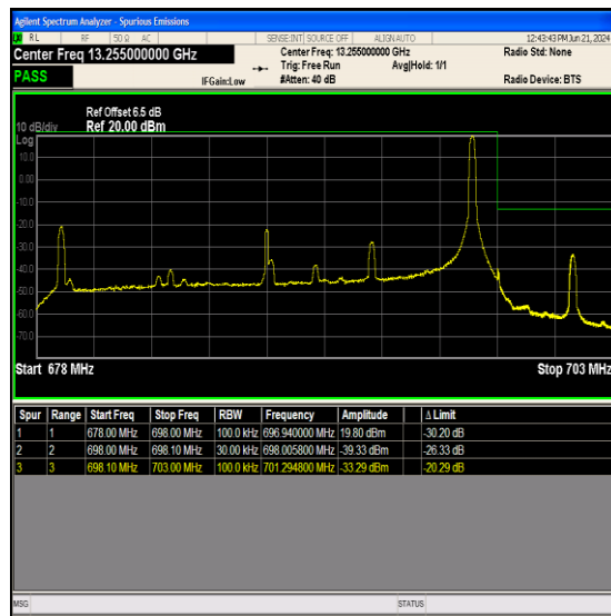
Band71_20MHz_64QAM_133372_1RB#99
