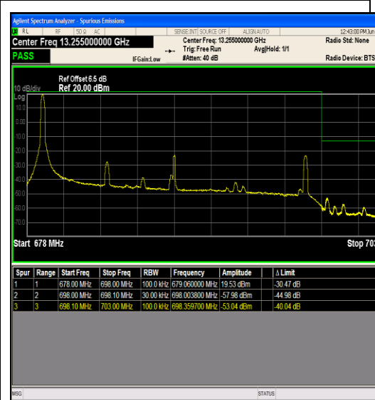
Band71_20MHz_64QAM_133222_1RB#99
