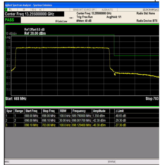
Band71_10MHz_16QAM_133422_50RB#0
