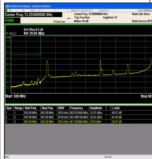
Band71_20MHz_64QAM_133222_1RB#99
