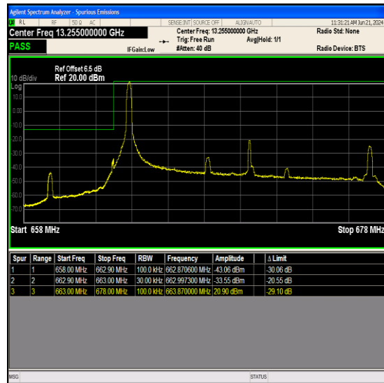
Band71_15MHz_QPSK_133197_1RB#0
