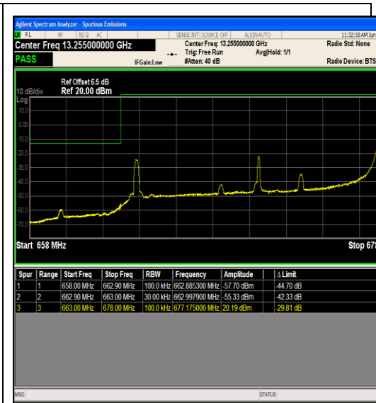
Band71_15MHz_16QAM_133197_1RB#74
