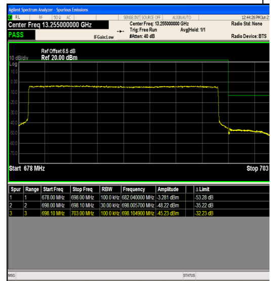
Band71_20MHz_64QAM_133372_100RB#0
