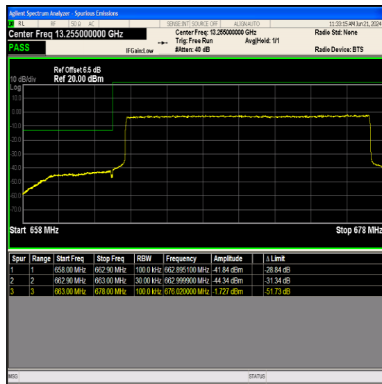
Band71_15MHz_64QAM_133197_75RB#0
