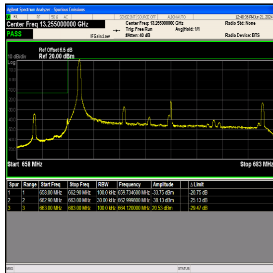
Band71_20MHz_16QAM_133222_1RB#0
