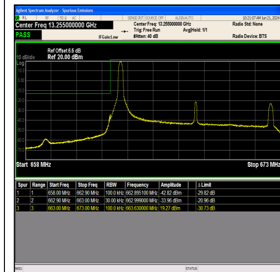
Band71_10MHz_16QAM_133172_1RB#0
