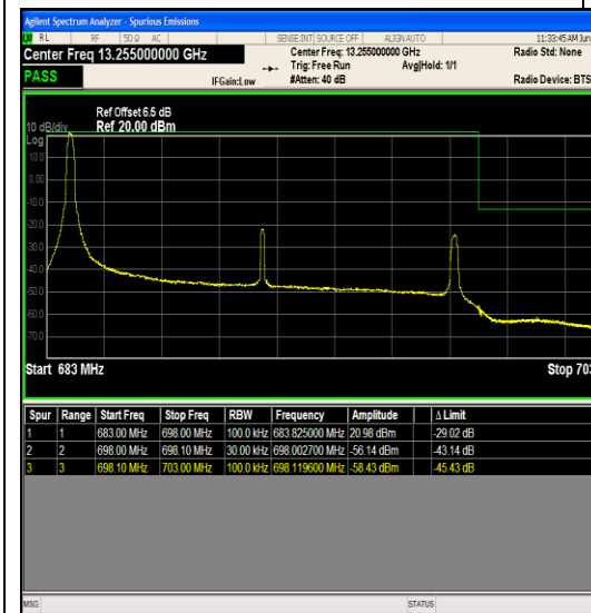
Band71_15MHz_16QAM_133397_1RB#0
