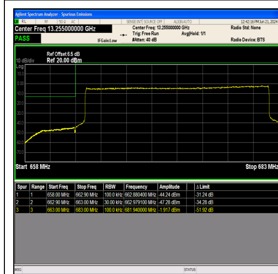
Band71_20MHz_64QAM_133222_1RB#0
