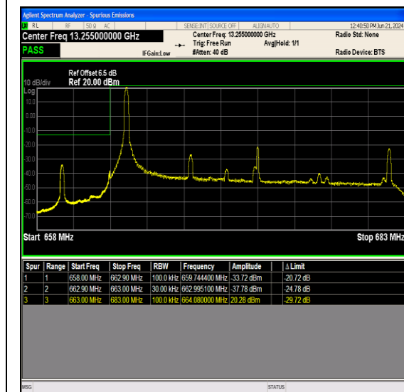
Band71_20MHz_64QAM_133222_1RB#0
