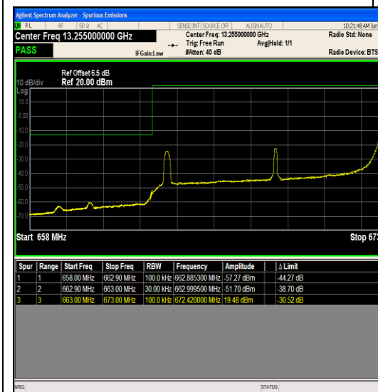
Band71_10MHz_16QAM_133172_1RB#49
