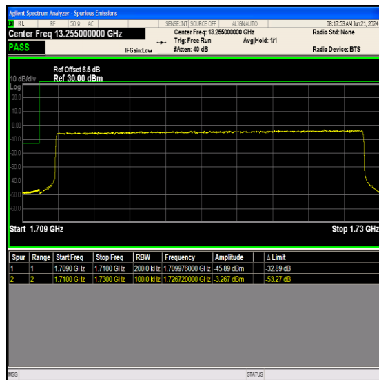
Band66_20MHz_64QAM_132072_100RB#0
