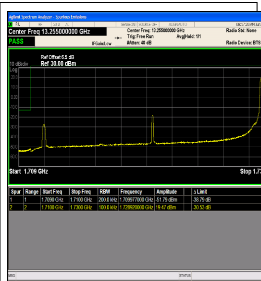
Band66_20MHz_64QAM_132072_1RB#99
