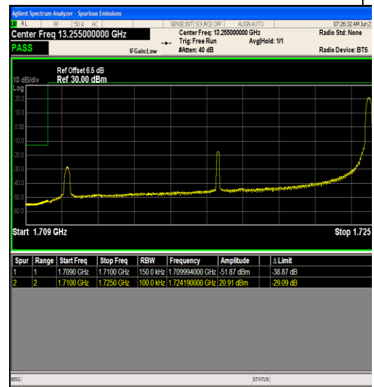
Band66_15MHz_QPSK_132047_1RB#74
