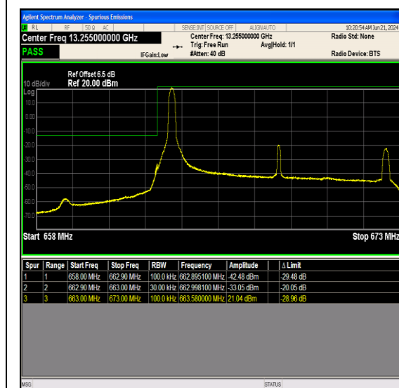
Band71_5MHz_16QAM_133447_1RB#24
