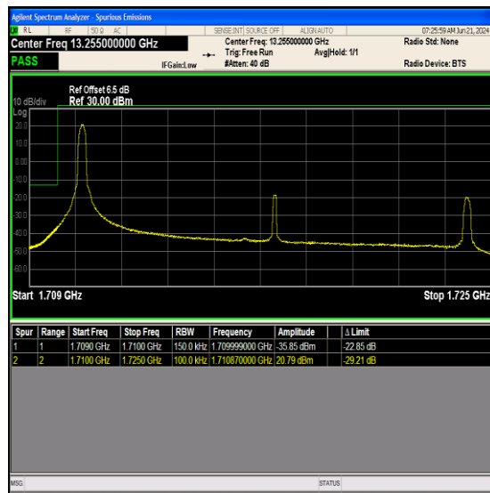
Band66_15MHz_QPSK_132047_1RB#0
