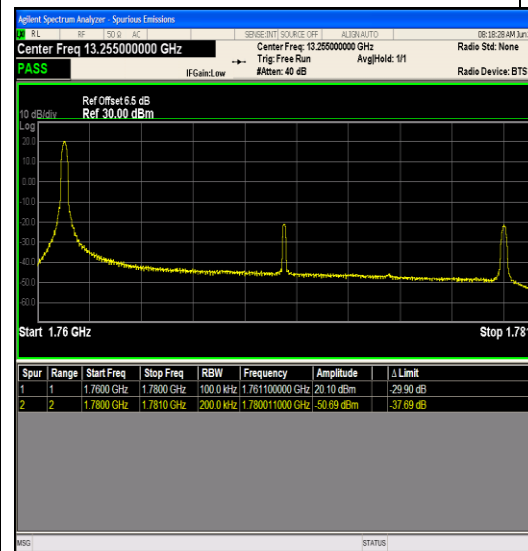
Band66_20MHz_64QAM_132572_1RB#0
