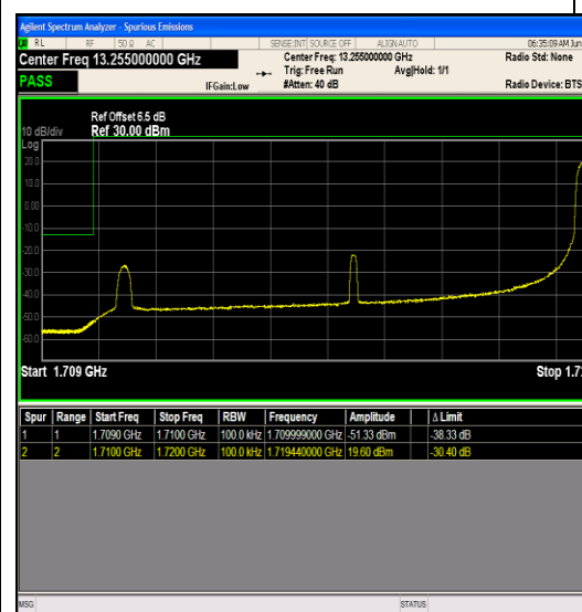
Band66_10MHz_QPSK_132622_50RB#0
