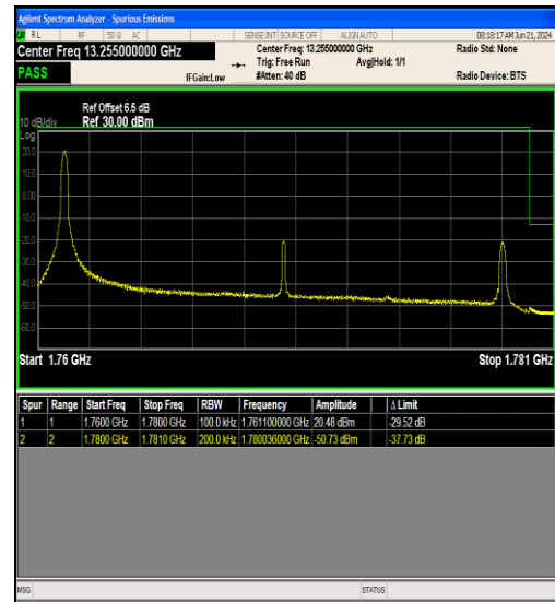
Band66_20MHz_16QAM_132572_1RB#0
