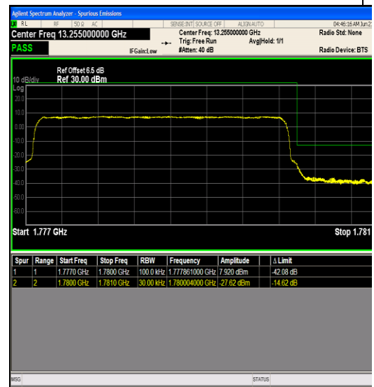
Band66_3MHz_QPSK_132657_15RB#0
