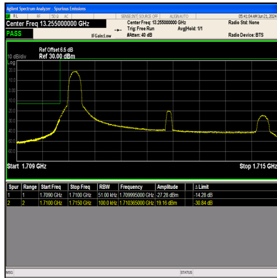
Band66_5MHz_64QAM_131997_1RB#0
