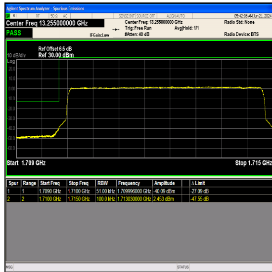
Band66_5MHz_64QAM_131997_25RB#0
