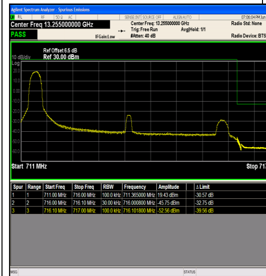
Band17_5MHz_16QAM_23825_1RB#0
