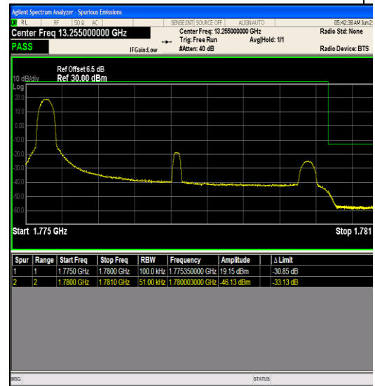
Band66_5MHz_64QAM_132647_1RB#0
