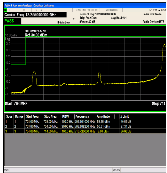
Band17_10MHz_16QAM_23780_1RB#49
