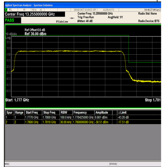
Band66_3MHz_16QAM_132657_15RB#0
