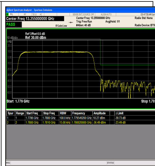
Band66_1.4MHz_16QAM_132665_6RB#0
