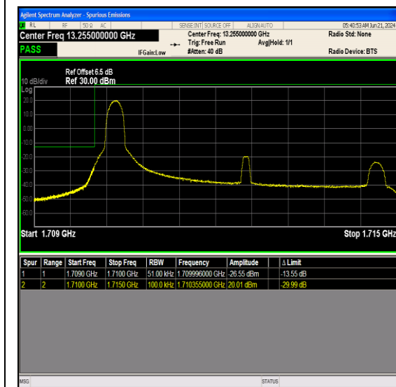
Band66_5MHz_16QAM_131997_1RB#0
