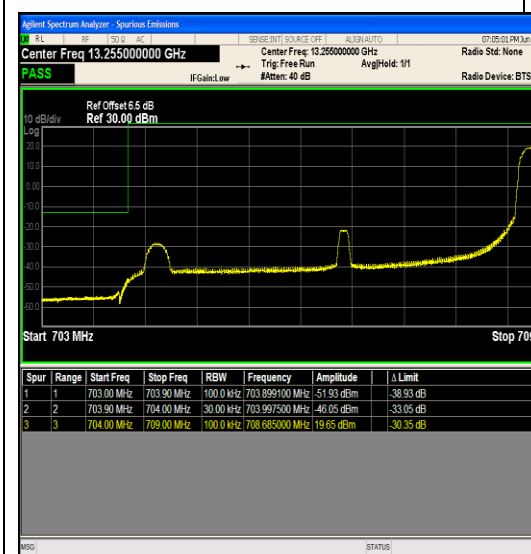
Band17_5MHz_QPSK_23825_25RB#0
