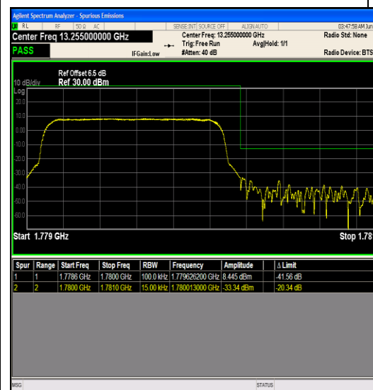
Band66_1.4MHz_64QAM_132665_1RB#0
