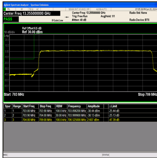
Band17_5MHz_64QAM_23755_25RB#0
