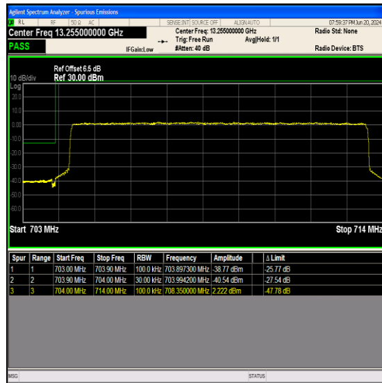
Band17_10MHz_QPSK_23780_50RB#0
