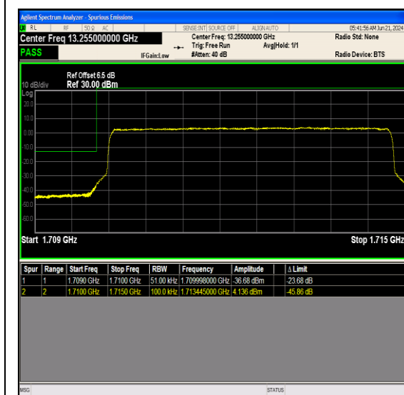
Band66_5MHz_16QAM_131997_1RB#0
