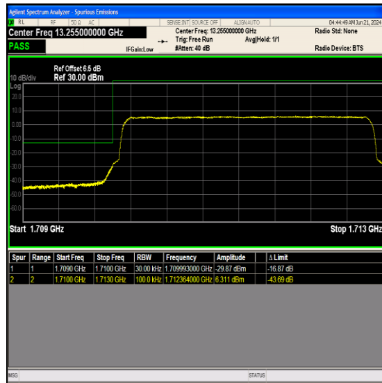
Band66_3MHz_16QAM_131987_15RB#0
