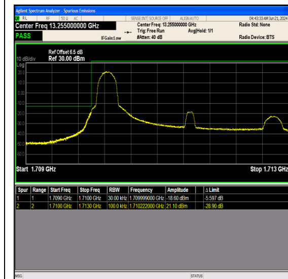
Band66_3MHz_QPSK_131987_1RB#0
