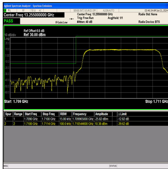
Band66_1.4MHz_16QAM_131979_6RB#0
