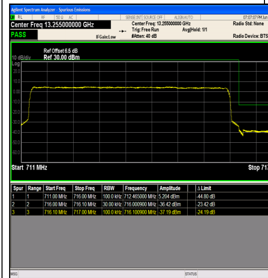
Band17_5MHz_QPSK_23825_25RB#0
