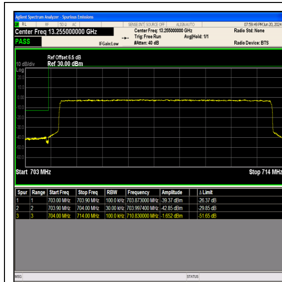
Band17_10MHz_16QAM_23780_50RB#0
