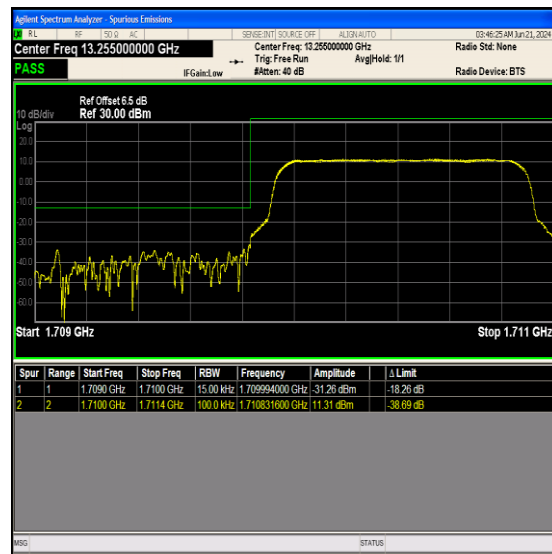
Band66_1.4MHz_QPSK_131979_6RB#0
