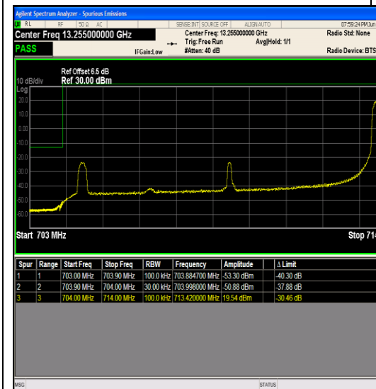
Band17_10MHz_64QAM_23780_1RB#49
