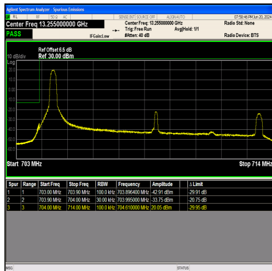
Band17_10MHz_64QAM_23780_1RB#0
