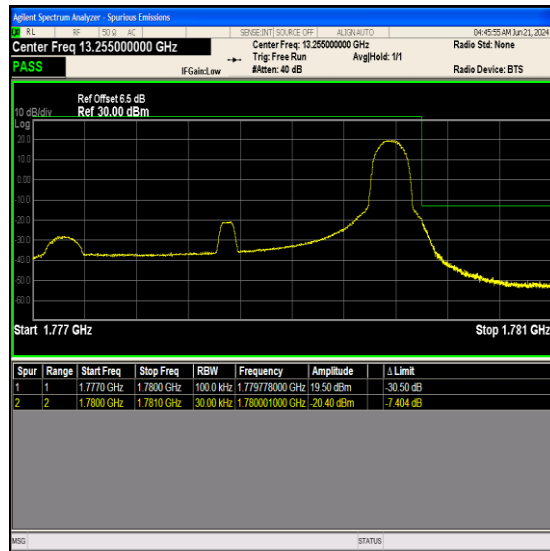
Band66_3MHz_16QAM_132657_1RB#14
