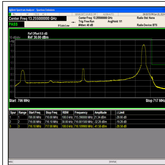
Band17_10MHz_QPSK_23800_1RB#49
