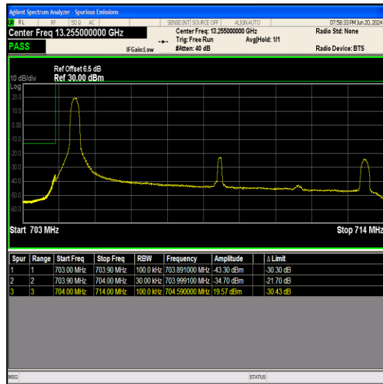
Band17_10MHz_16QAM_23780_1RB#0
