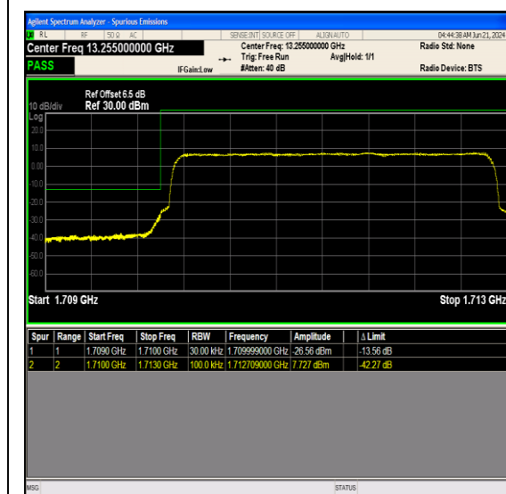
Band66_3MHz_QPSK_131987_1RB#0
