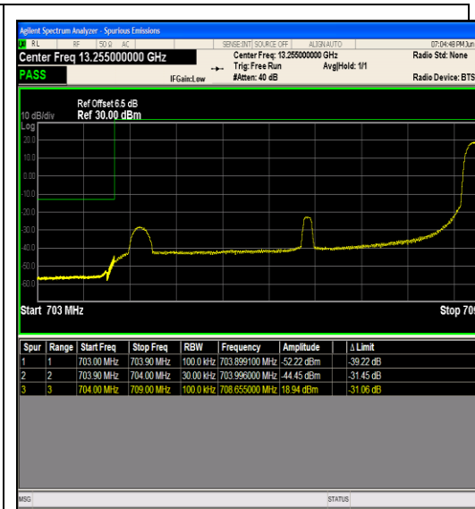
Band17_5MHz_16QAM_23755_1RB#24
