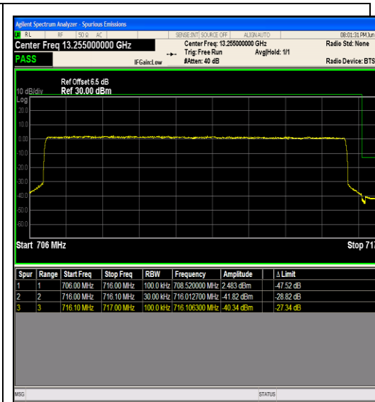
Band17_10MHz_QPSK_23800_50RB#0
