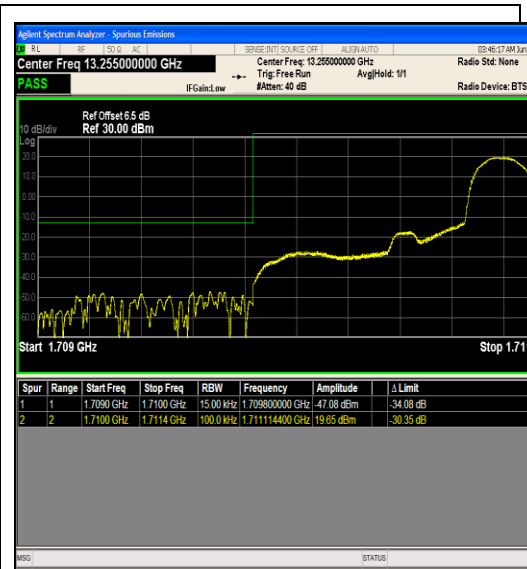
Band66_1.4MHz_64QAM_131979_1RB#5
