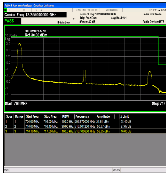
Band17_10MHz_QPSK_23800_1RB#0
