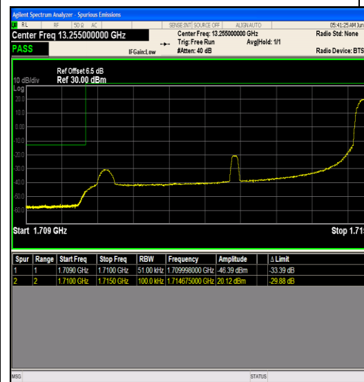
Band66_5MHz_16QAM_131997_1RB#24
