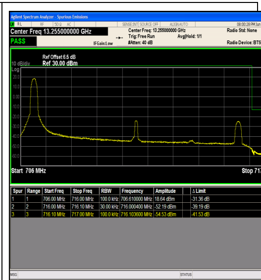
Band17_10MHz_16QAM_23800_1RB#0
