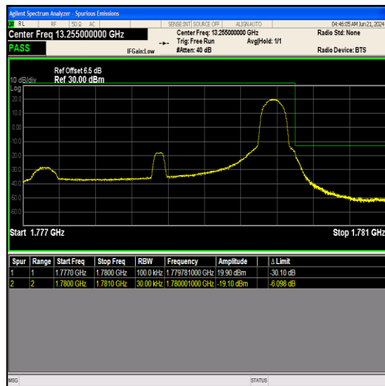
Band66_3MHz_64QAM_132657_1RB#14
