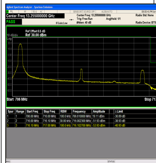
Band17_10MHz_64QAM_23780_1RB#49
