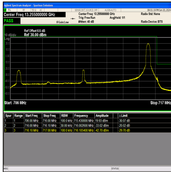
Band17_10MHz_64QAM_23800_1RB#49
