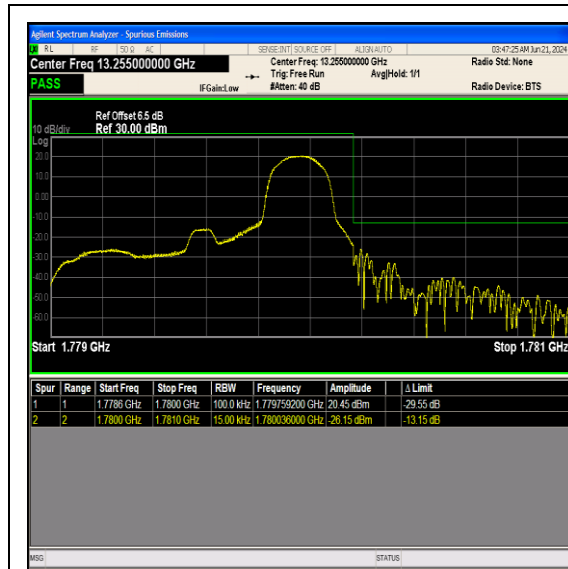
Band66_1.4MHz_16QAM_132665_1RB#5
