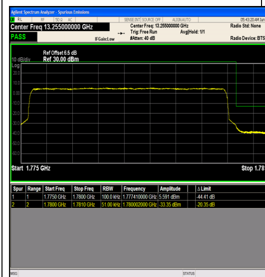
Band66_5MHz_QPSK_132647_1RB#0
