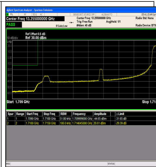
Band66_5MHz_QPSK_131997_1RB#24
