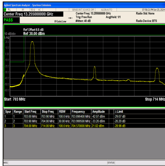
Band17_10MHz_QPSK_23780_1RB#0
