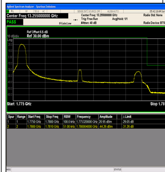
Band66_5MHz_QPSK_132647_1RB#0
