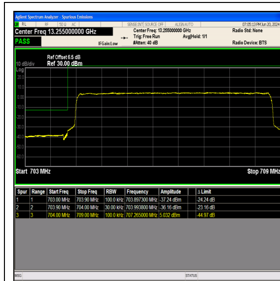
Band17_5MHz_QPSK_23755_25RB#0
