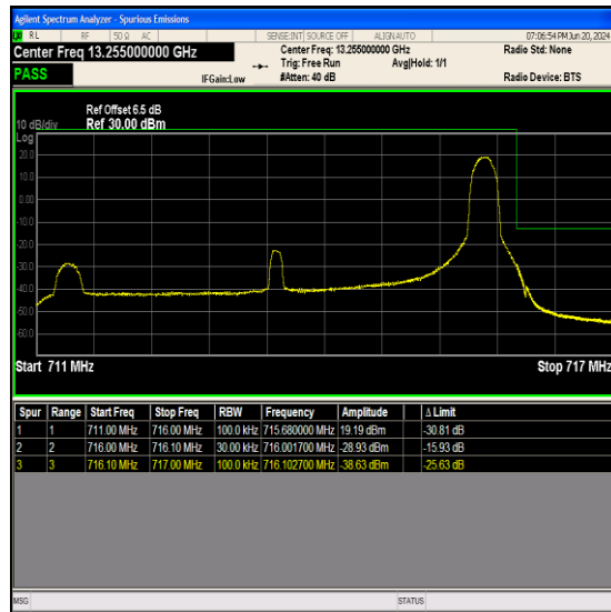
Band17_5MHz_64QAM_23825_1RB#24
