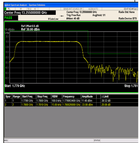
Band66_1.4MHz_QPSK_132665_6RB#0
