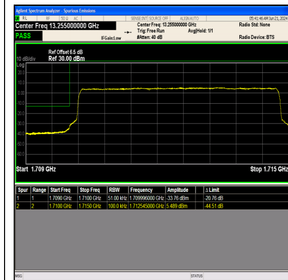
Band66_5MHz_QPSK_131997_25RB#0
