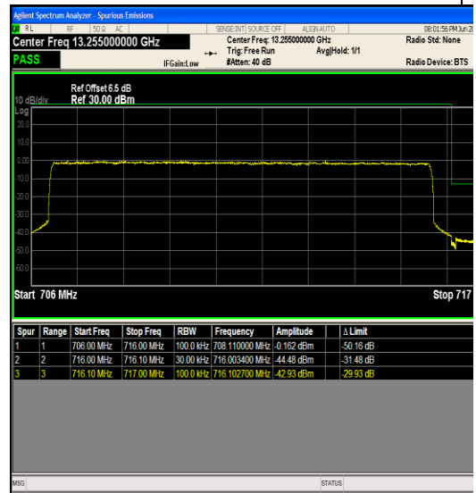
Band17_10MHz_64QAM_23800_50RB#0
