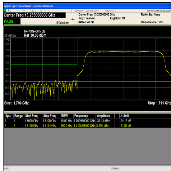
Band66_1.4MHz_64QAM_131979_6RB#0
