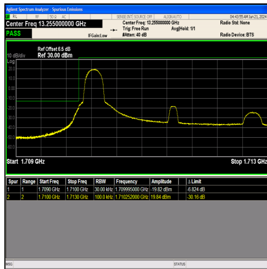
Band66_3MHz_64QAM_131987_1RB#0
