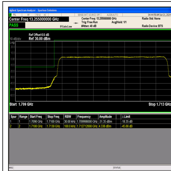
Band66_3MHz_64QAM_131987_15RB#0
