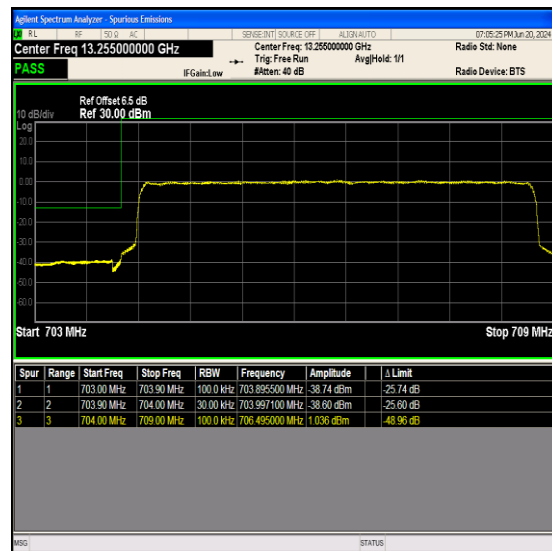
Band17_5MHz_16QAM_23755_25RB#0
