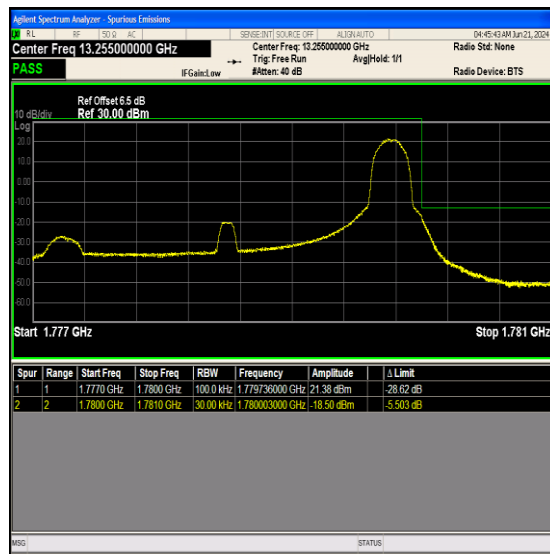
Band66_3MHz_QPSK_132657_1RB#14
