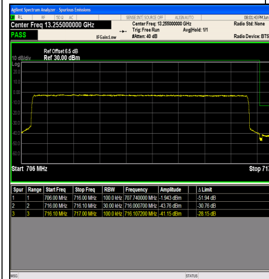
Band17_10MHz_16QAM_23800_50RB#0
