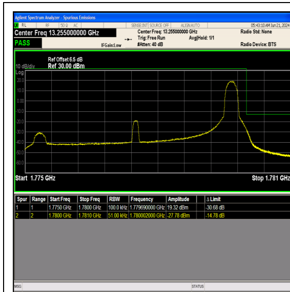
Band66_5MHz_64QAM_132647_1RB#24
