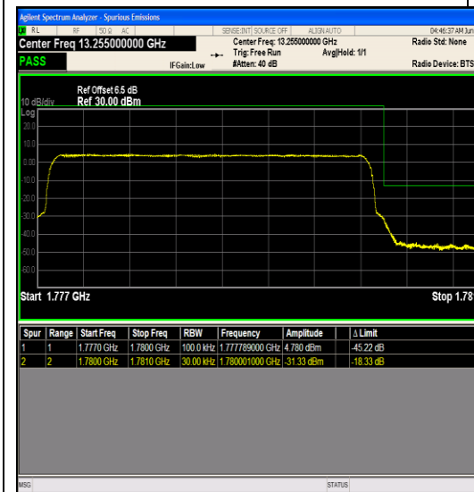
Band66_3MHz_64QAM_132657_15RB#0
