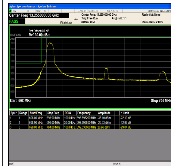
Band12_5MHz_QPSK_23035_1RB#0
