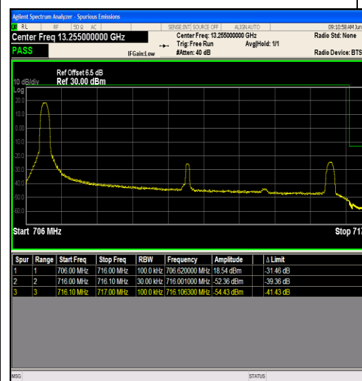
Band12_10MHz_16QAM_23060_1RB#49
