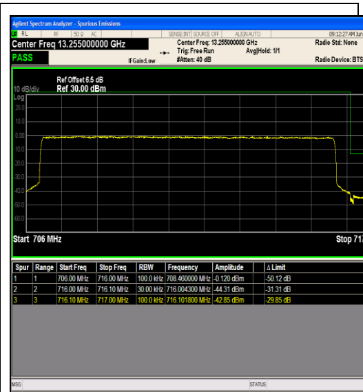
Band12_10MHz_64QAM_23130_50RB#0
