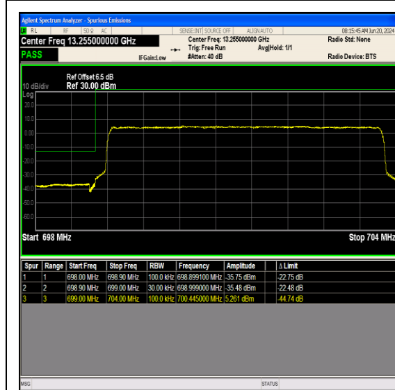
Band12_5MHz_QPSK_23035_1RB#0
