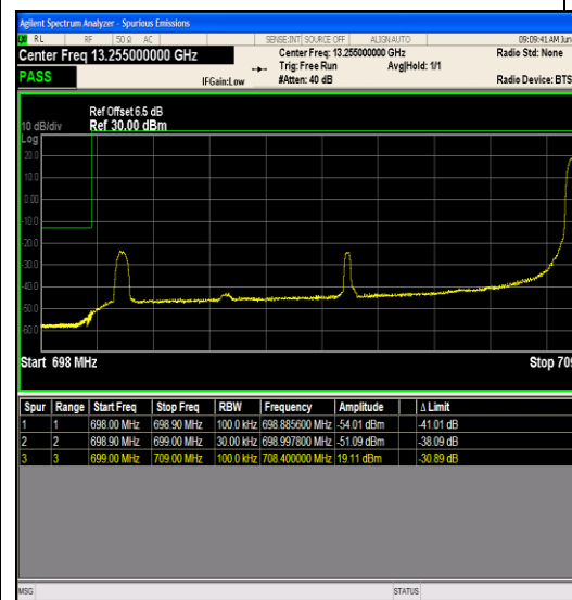
Band12_10MHz_16QAM_23060_1RB#49
