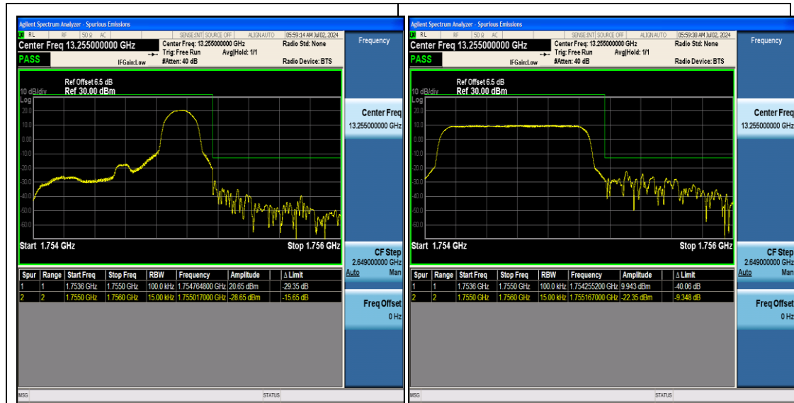
Band4_1.4MHz_16QAM_20393_1RB#5
