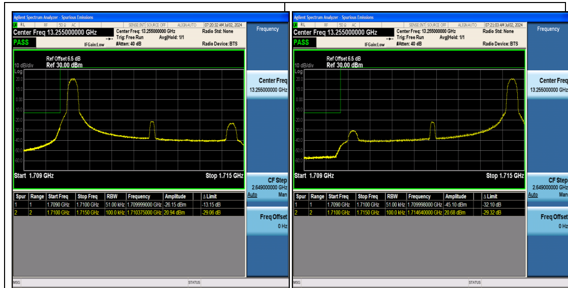
Band4_5MHz_QPSK_19975_1RB#0
