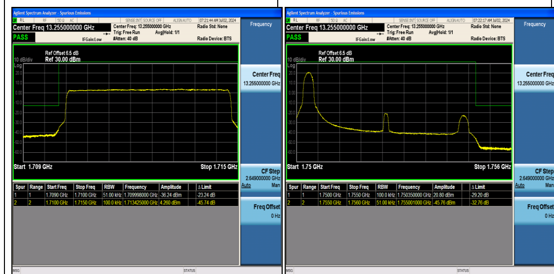
Band4_5MHz_16QAM_19975_1RB#0
