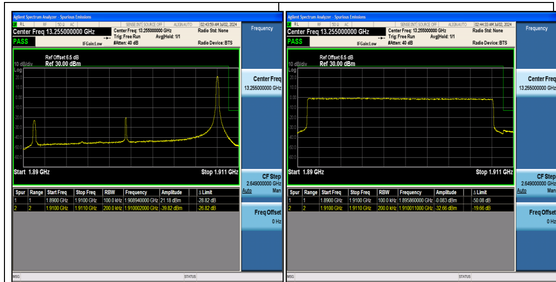
Band2_20MHz_QPSK_19100_1RB#99
