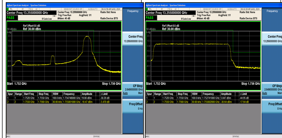
Band4_3MHz_64QAM_20385_1RB#14
