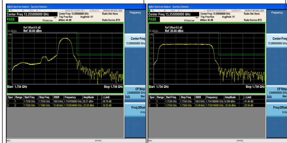
Band4_1.4MHz_64QAM_19957_6RB#0
