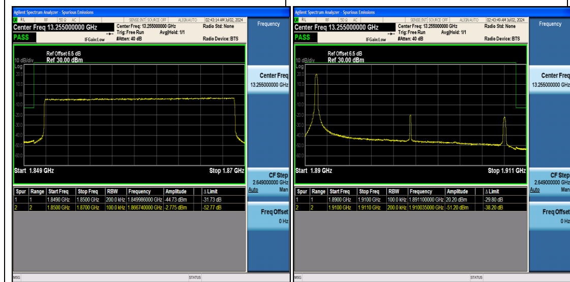
Band2_20MHz_64QAM_18700_1RB#0
