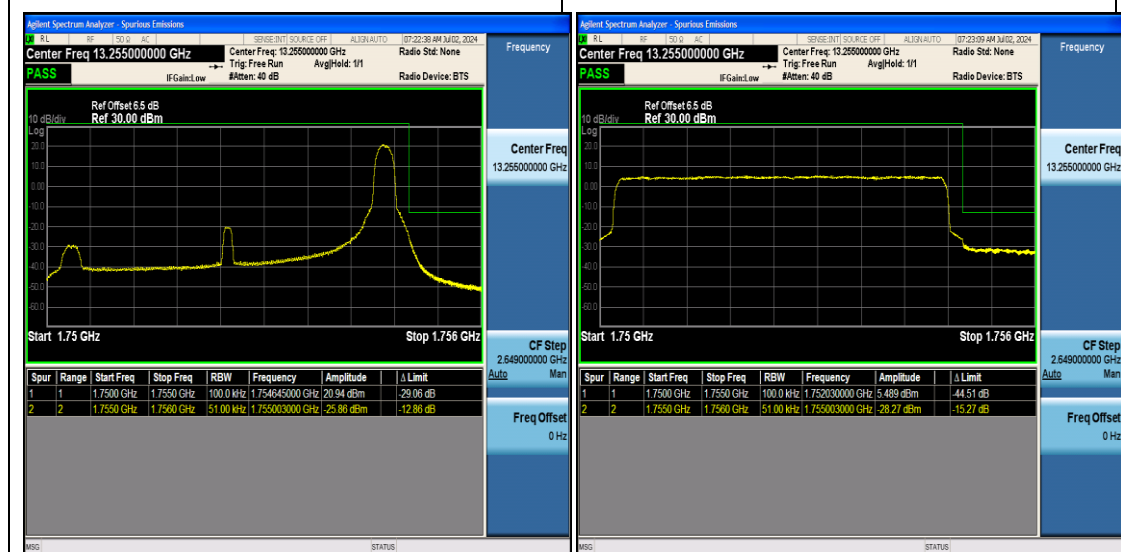
Band4_5MHz_QPSK_20375_1RB#0
