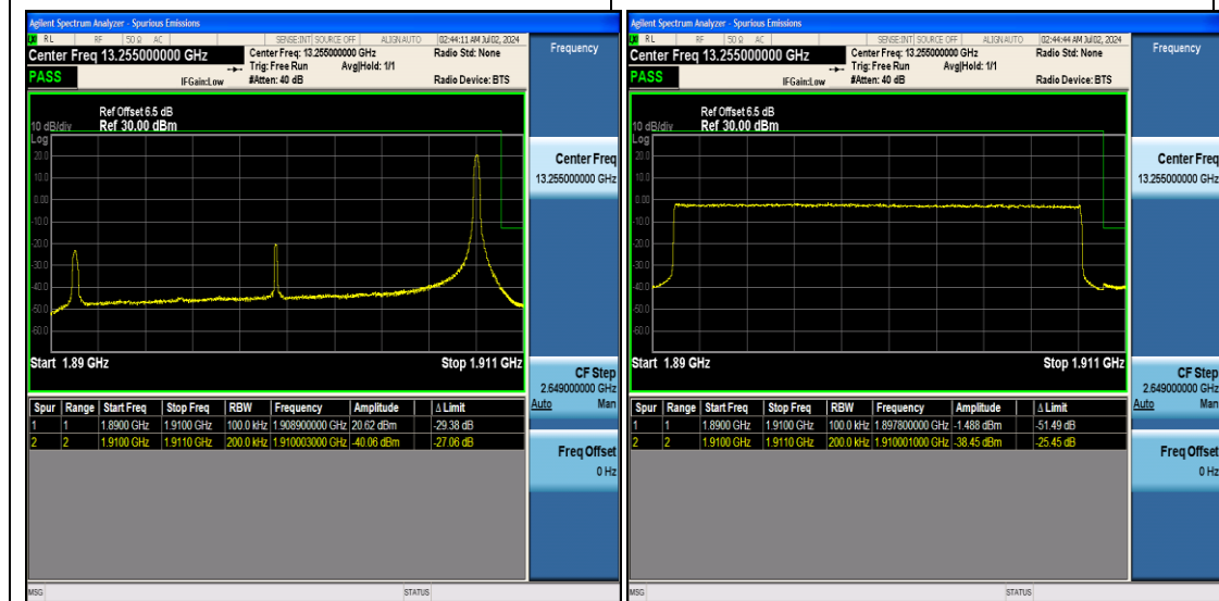
Band2_20MHz_16QAM_19100_1RB#99
