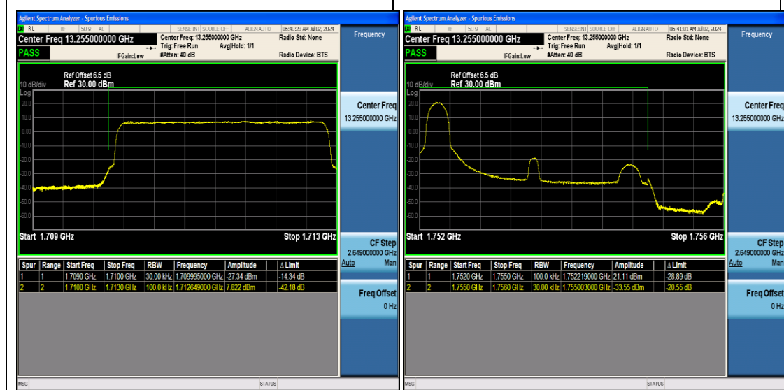
Band4_3MHz_QPSK_19965_1RB#0
