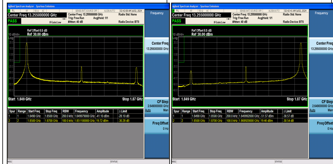
Band2_20MHz_64QAM_18700_1RB#0
