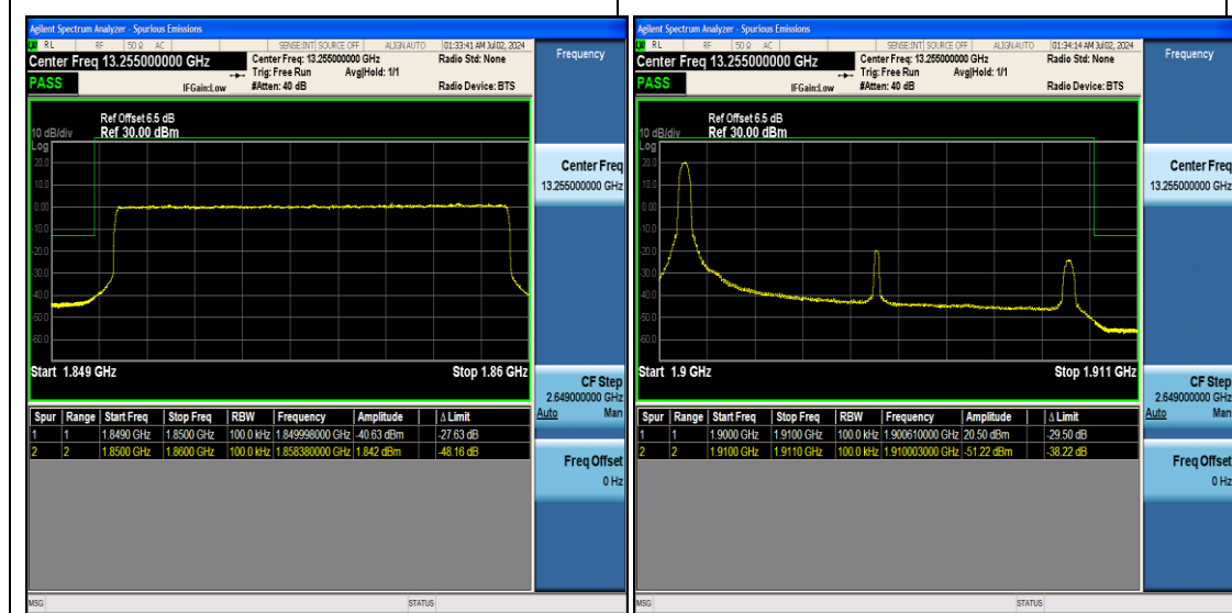
Band2_10MHz_16QAM_18650_1RB#0
