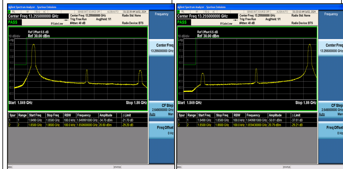
Band2_10MHz_16QAM_18650_1RB#0
