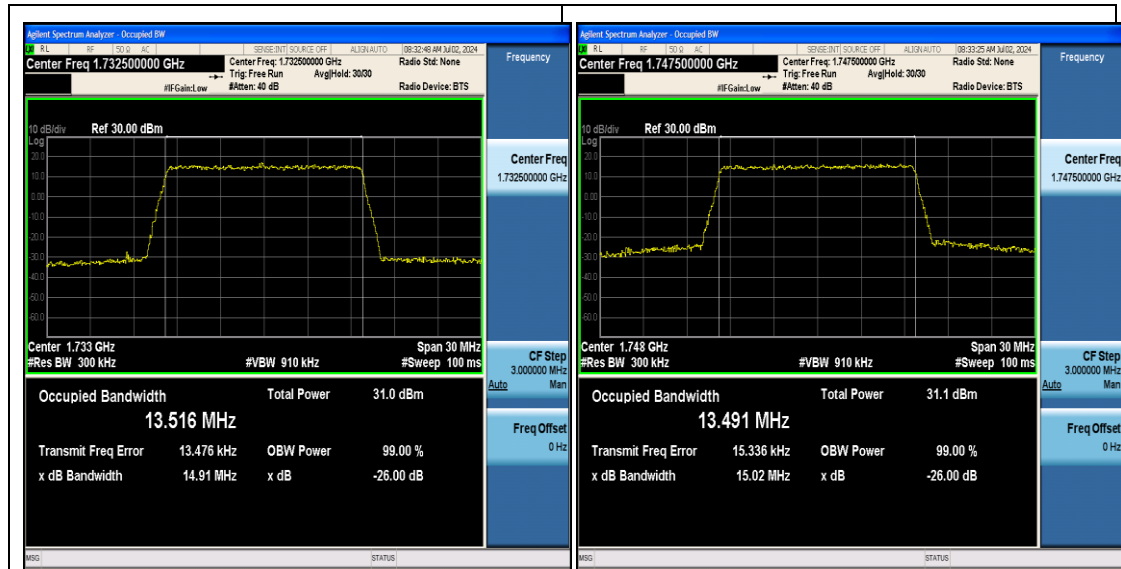
Band4-15MHz-64QAM-20175-75RB#0-PASS
