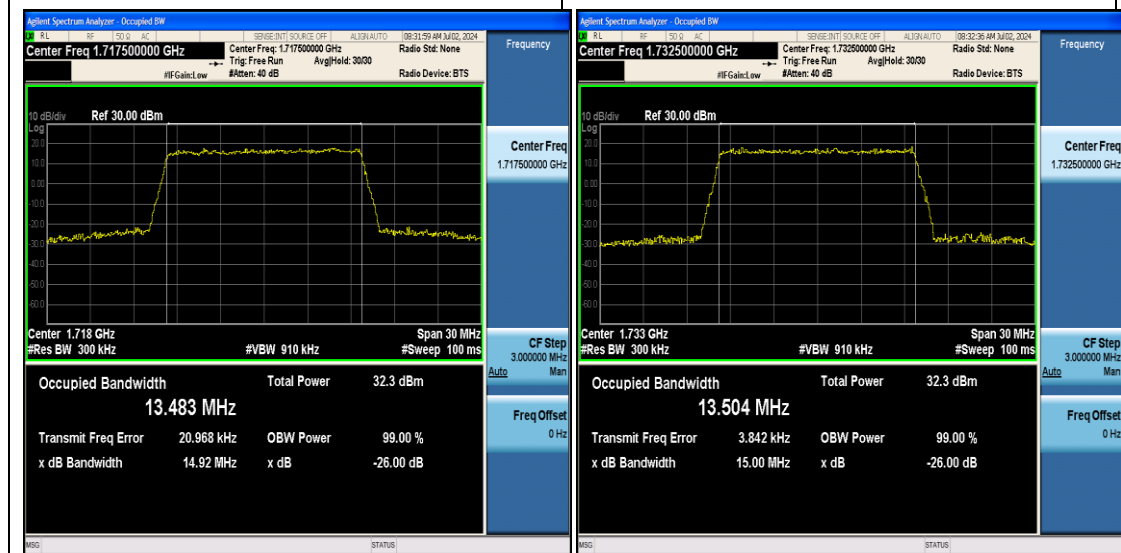
Band4-15MHz-16QAM-20025-75RB#0-PASS
