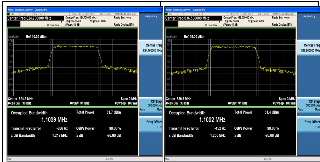
Band5-1.4MHz-16QAM-20407-6RB#0-PASS
