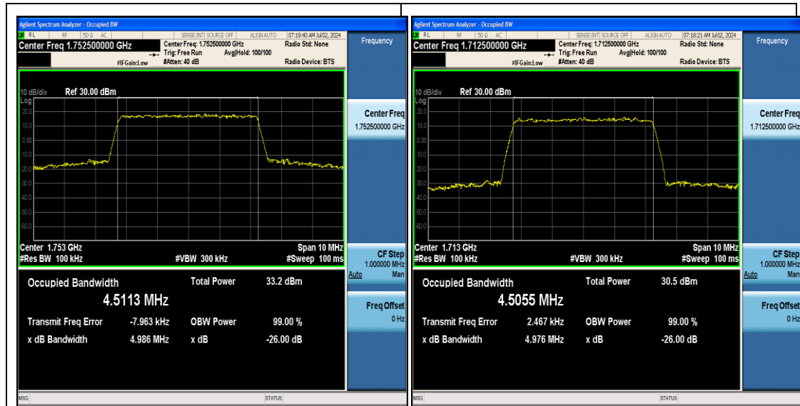
Band4-5MHz-QPSK-20375-25RB#0-PASS
