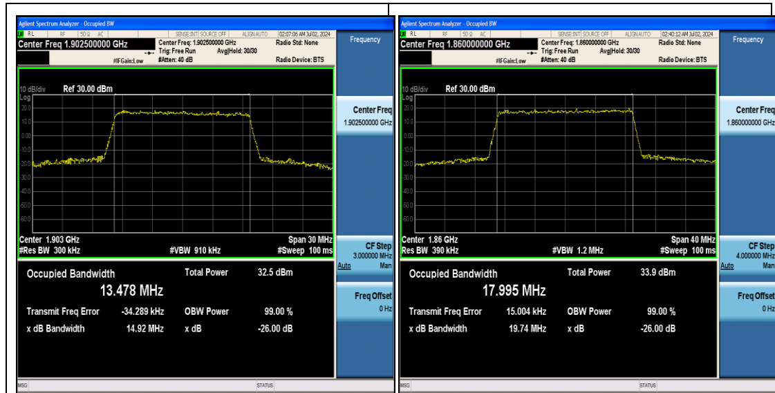
Band2-15MHz-16QAM-19125-75RB#0-PASS
